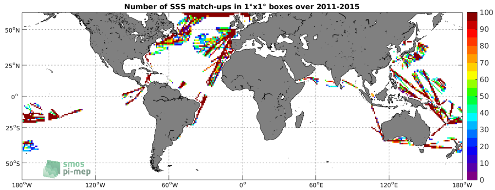
Figure 4: Number of SSS match-ups between TSG-LEGOS-DM SSS and the Aquarius-L3-JPL-V5-7DAY-RUNNING SSS product for the SMOS coastal zone (<800km) 60N-60S Pi-MEP region over 1°x1° boxes and for the full satellite product period.
