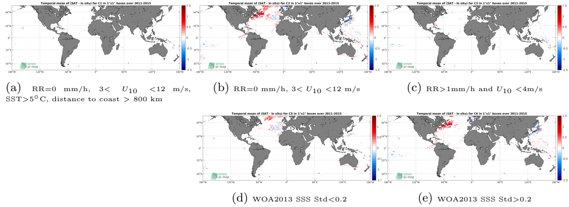
Figure 12: Temporal mean gridded over spatial boxes of size 1^\circ \times 1^\circ of \Delta SSS (Aquarius-L3-JPL-V5-7DAY-RUNNING - TSG-LEGOS-DM) for 5 different subdatasets corresponding to: RR=0 mm/h, 3 < U_{10} < 12 m/s, SST > 5^\circ C , distance to coast > 800 km (a), RR=0 mm/h, 3 < U_{10} < 12 m/s (b), RR > 1 mm/h and U_{10} < 4 m/s (c), WOA2013 SSS Std < 0.2 (d), WOA2013 SSS Std > 0.2 (e).
