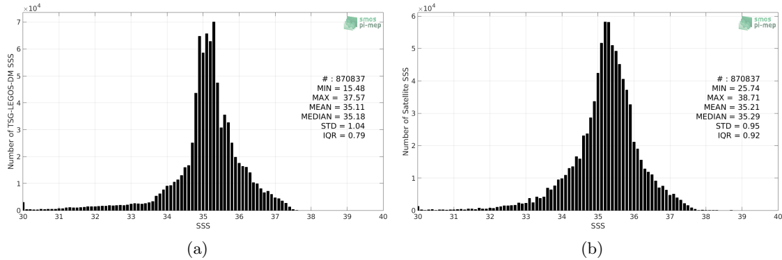
Figure 2: Histograms of SSS from TSG-LEGOS-DM (a) and Aquarius-L3-JPL-V5-7DAY-RUNNING (b) considering all match-up pairs per bins of 0.1 over the SMOS coastal zone (<800km) 60N-60S Pi-MEP region and for the full satellite product period.
