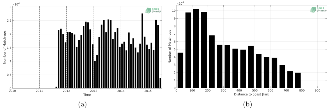
Figure 1: Number of match-ups between TSG-LEGOS-DM and Aquarius-L3-JPL-V5-7DAY-RUNNING SSS as a function of time (a) and as function of the distance to coast (b) over the SMOS coastal zone (<800km) 60N-60S Pi-MEP region and for the full satellite product period.
