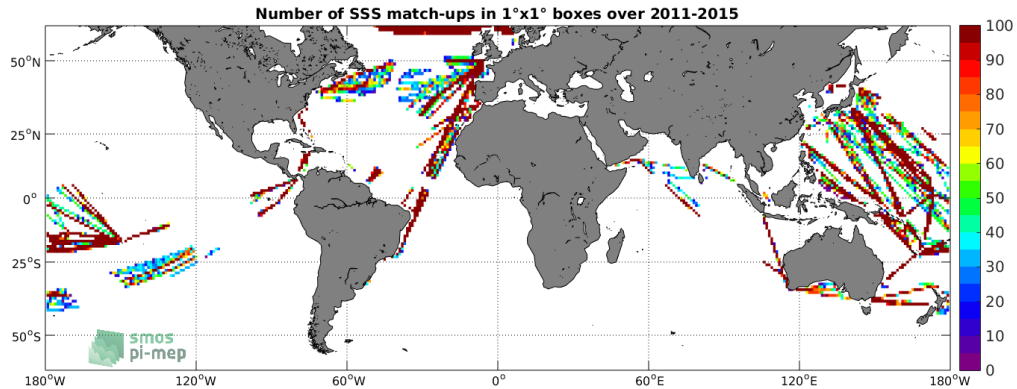
Figure 4: Number of SSS match-ups between TSG-LEGOS-DM SSS and the Aquarius-L3-JPL-V5-7DAY-RUNNING SSS product for the SMOS coastal zone ( \leq 800\text{km} ) 60N-60S Pi-MEP region over 1^\circ \times 1^\circ boxes and for the full satellite product period.
