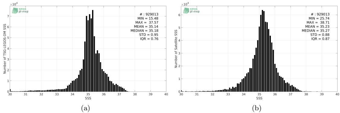
Figure 2: Histograms of SSS from TSG-LEGOS-DM (a) and Aquarius-L3-JPL-V5-7DAY-RUNNING (b) considering all match-up pairs per bins of 0.1 over the SMOS coastal zone ( \geq 800 km) 60N-60S Pi-MEP region and for the full satellite product period.
