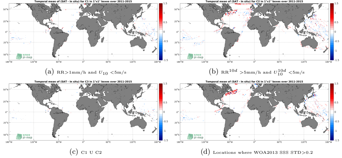
Figure 12: Temporal mean gridded over spatial boxes of size 1^\circ \times 1^\circ of \Delta SSS (Aquarius-L3-JPL-V5-7DAY-RUNNING - TSG-LEGOS-DM) for 4 different subdatasets corresponding to: RR > 1\text{mm/h} and U_{10} < 5\text{m/s} (a), RR^{10d} > 5\text{mm/h} and U_{10}^{10d} < 5\text{m/s} (b), C1 U C2 (c), Locations where WOA2013 SSS STD > 0.2 (d).
