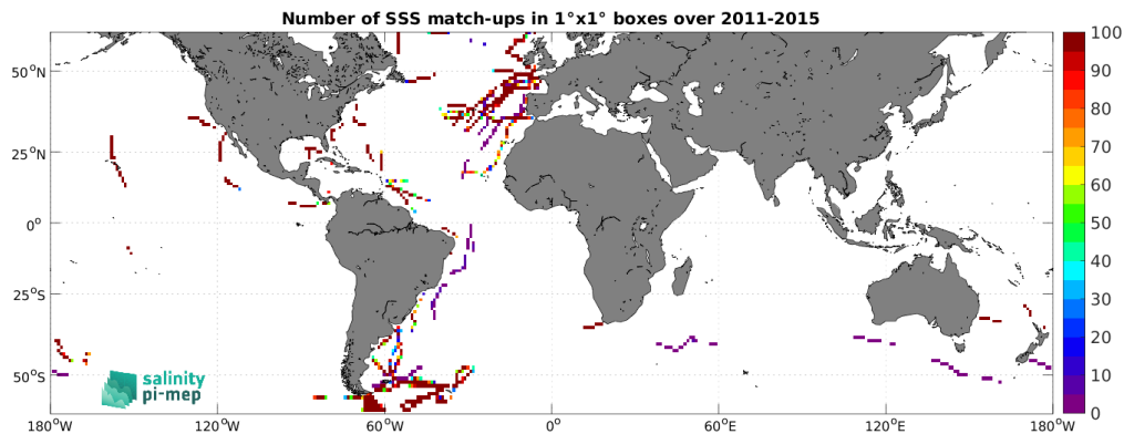
Figure 5: Number of SSS match-ups between TSG (GOSUD-Sailing-ship) SSS and the Aquarius SSS L3 CAP v5 - 7-Day running (JPL) SSS product for the SMOS coastal zone ( <800\text{km} ) 60N-60S Pi-MEP region over 1^\circ \times 1^\circ boxes and for the full satellite product period.
