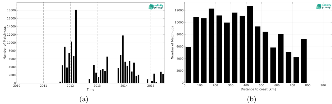
Figure 2: Number of match-ups between TSG (GOSUD-Sailing-ship) and Aquarius SSS L3 CAP v5 - 7-Day running (JPL) SSS as a function of time (a) and as function of the distance to coast (b) over the SMOS coastal zone (<800km) 60N-60S Pi-MEP region and for the full satellite product period.
