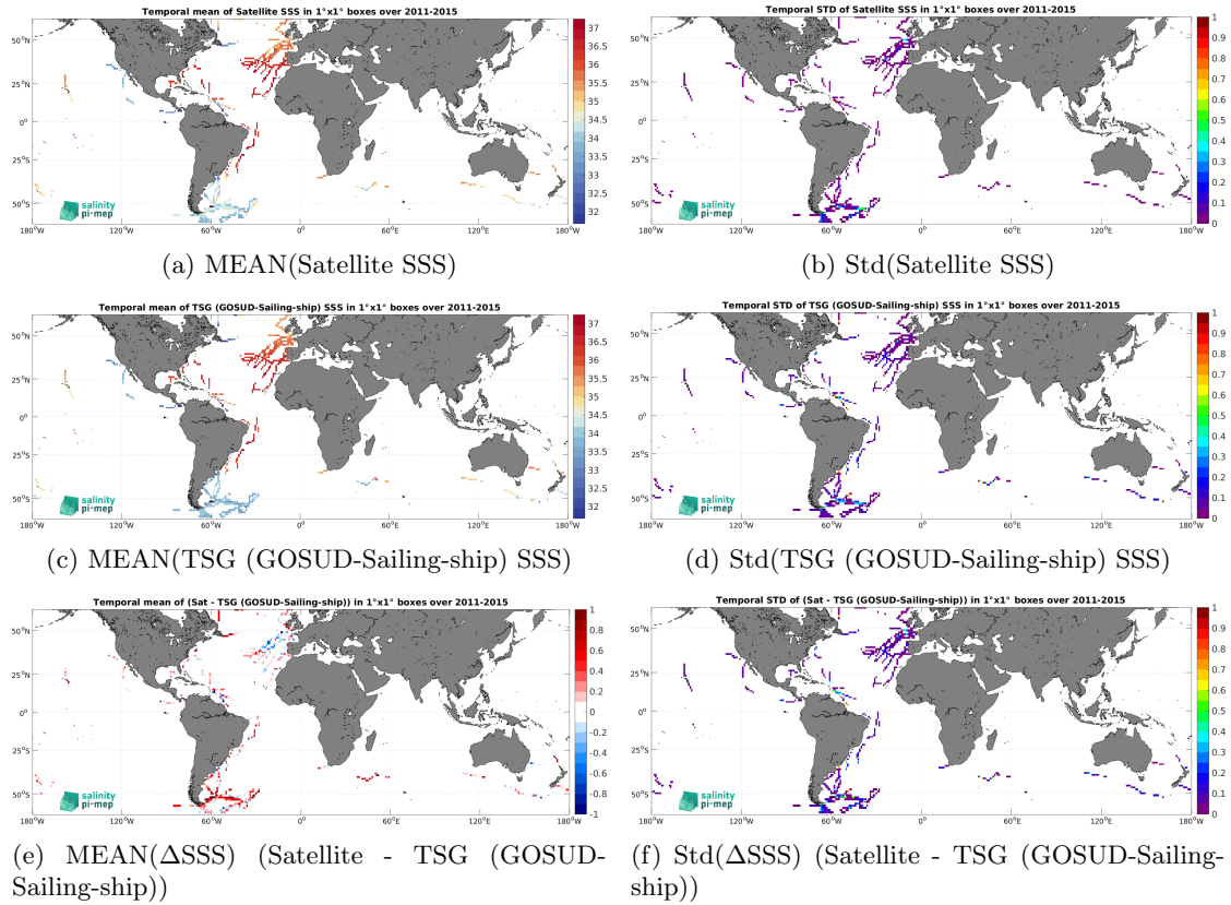
Figure 7: Temporal mean (left) and Std (right) of SSS from Aquarius SSS L3 CAP v5 - 7-Day running (JPL) (top), TSG (GOSUD-Sailing-ship) (middle), and of \Delta SSS (Satellite - TSG (GOSUD-Sailing-ship)). Only match-up pairs are used to generate these maps.
