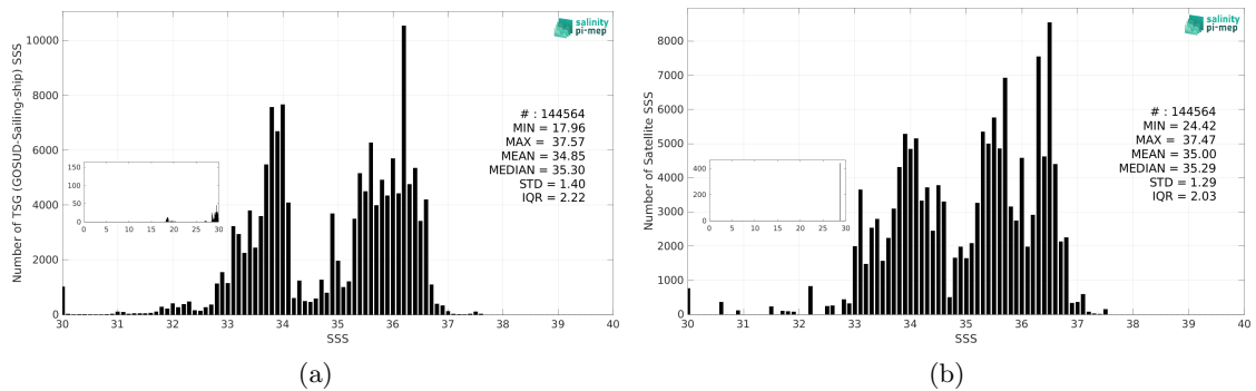
Figure 3: Histograms of SSS from TSG (GOSUD-Sailing-ship) (a) and Aquarius SSS L3 CAP v5 - 7-Day running (JPL) (b) considering all match-up pairs per bins of 0.1 over the SMOS coastal zone (<800km) 60N-60S Pi-MEP region and for the full satellite product period.
