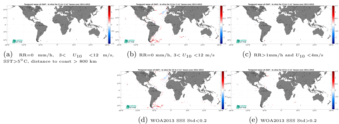
Figure 14: Temporal mean gridded over spatial boxes of size 1^\circ \times 1^\circ of \Delta SSS (Aquarius SSS L3 CAP v5 - 7-Day running (JPL) - TSG (GOSUD-Sailing-ship)) for 5 different subdatasets corresponding to:RR=0 mm/h, 3 < U_{10} < 12 m/s, SST >5^\circ C, distance to coast > 800 km (a), RR=0 mm/h, 3 < U_{10} < 12 m/s (b), RR >1 mm/h and U_{10} < 4 m/s (c), WOA2013 SSS Std <0.2 (d), WOA2013 SSS Std >0.2 (e).
