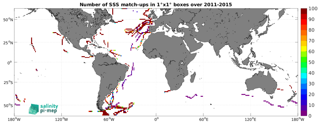
Figure 4: Number of SSS match-ups between TSG (GOSUD-Sailing-ship) SSS and the Aquarius SSS L3 CAP v5 - 7-Day running (JPL) SSS product for the SMOS coastal zone ( <800\text{km} ) 60N-60S Pi-MEP region over 1^\circ \times 1^\circ boxes and for the full satellite product period.
