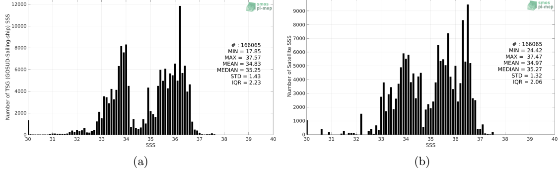
Figure 2: Histograms of SSS from TSG (GOSUD-Sailing-ship) (a) and Aquarius SSS L3 CAP v5 - 7-Day running (JPL) (b) considering all match-up pairs per bins of 0.1 over the SMOS coastal zone (<800km) 60N-60S Pi-MEP region and for the full satellite product period.
