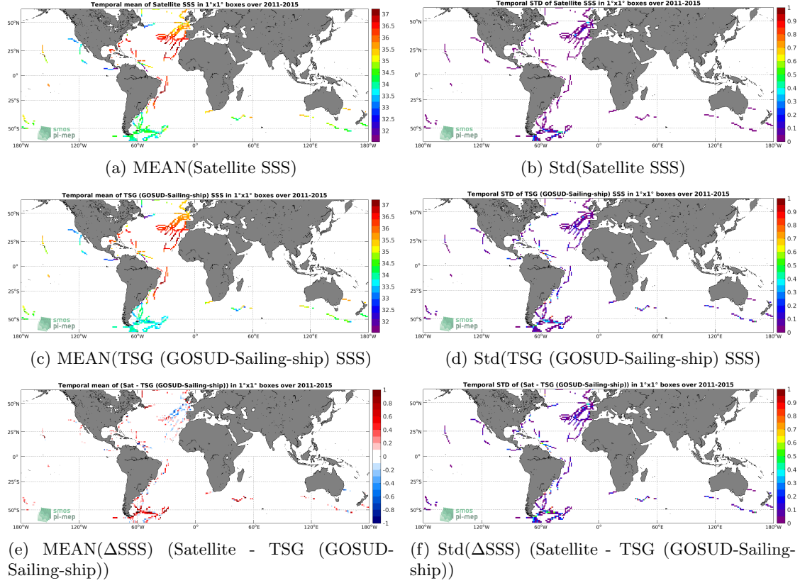
Figure 6: Temporal mean (left) and Std (right) of SSS from Aquarius SSS L3 CAP v5 - 7-Day running (JPL) (top), TSG (GOSUD-Sailing-ship) (middle), and of \Delta SSS (Satellite - TSG (GOSUD-Sailing-ship)). Only match-up pairs are used to generate these maps.
