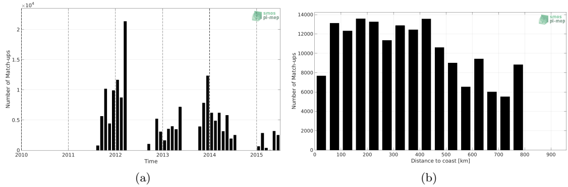
Figure 1: Number of match-ups between TSG (GOSUD-Sailing-ship) and Aquarius SSS L3 CAP v5 - 7-Day running (JPL) SSS as a function of time (a) and as function of the distance to coast (b) over the SMOS coastal zone (<800km) 60N-60S Pi-MEP region and for the full satellite product period.
