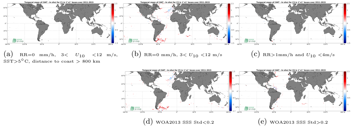
Figure 12: Temporal mean gridded over spatial boxes of size 1^\circ \times 1^\circ of \Delta SSS (Aquarius SSS L3 CAP v5 - 7-Day running (JPL) - TSG (GOSUD-Sailing-ship)) for 5 different subdatasets corresponding to:RR=0 mm/h, 3 < U_{10} < 12 m/s, SST >5^\circ\text{C} , distance to coast > 800 km (a), RR=0 mm/h, 3 < U_{10} < 12 m/s (b), RR >1 mm/h and U_{10} < 4 m/s (c), WOA2013 SSS Std <0.2 (d), WOA2013 SSS Std >0.2 (e).
