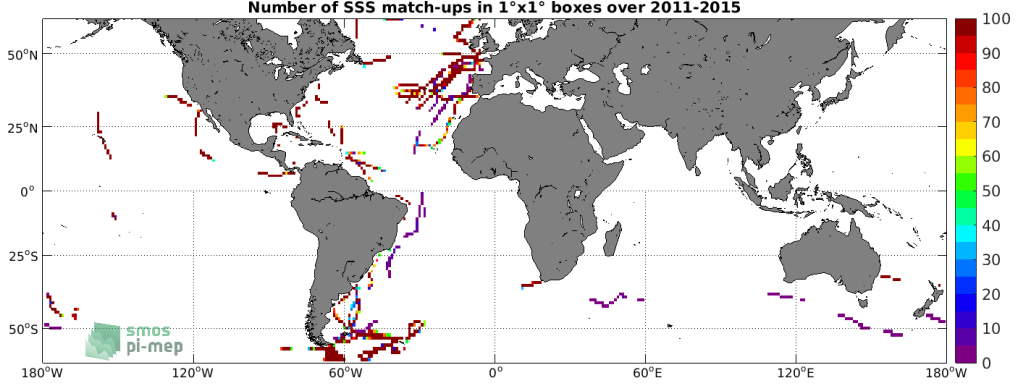
Figure 4: Number of SSS match-ups between TSG (GOSUD-Sailing-ship) SSS and the Aquarius SSS L3 CAP v5 - 7-Day running (JPL) SSS product for the SMOS coastal zone (<800km) 60N-60S Pi-MEP region over 1^\circ \times 1^\circ boxes and for the full satellite product period.
