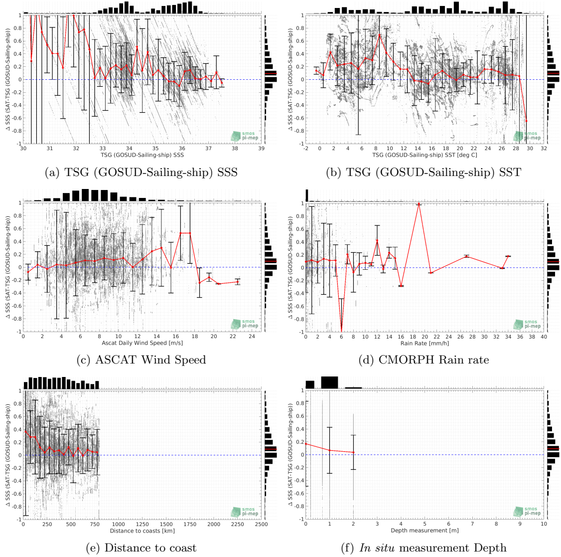
Figure 11: \Delta\text{SSS} (Satellite - TSG (GOSUD-Sailing-ship)) sorted as function of TSG (GOSUD-Sailing-ship) SSS values a), TSG (GOSUD-Sailing-ship) SST b), ASCAT Wind speed c), CMORPH rain rate d), distance to coast (e) and in situ measurement depth (f). In all plots the median and Std of \Delta\text{SSS} for each bin is indicated by the red curves and black vertical thick bars ( \pm 1 Std)
