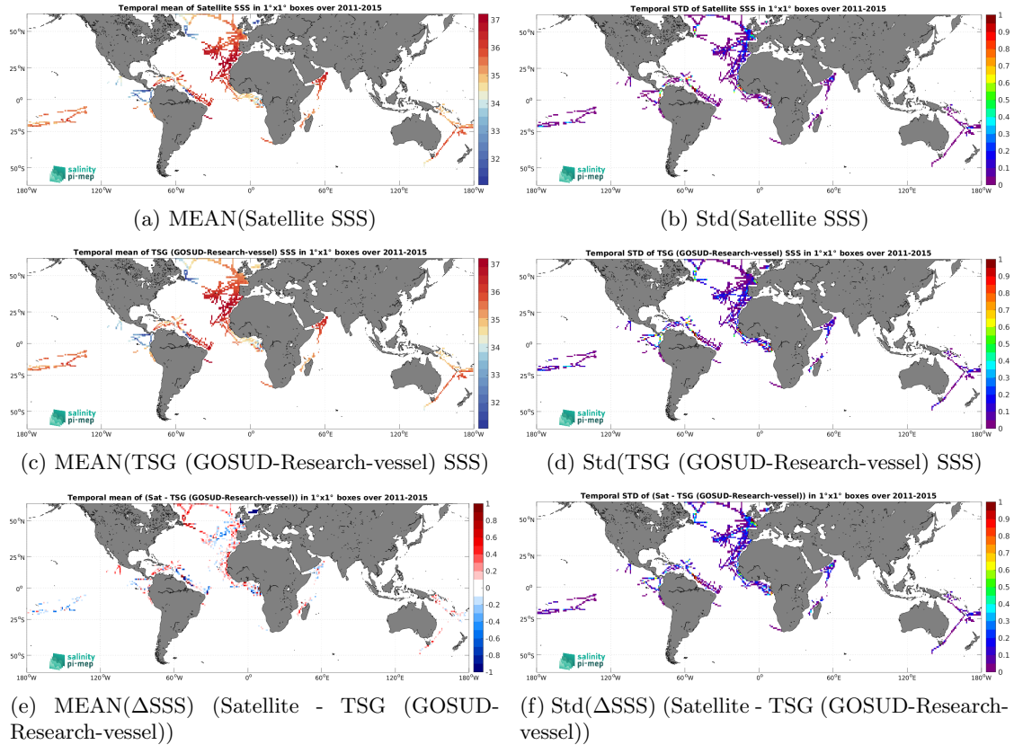
Figure 7: Temporal mean (left) and Std (right) of SSS from Aquarius SSS L3 CAP v5 - 7-Day running (JPL) (top), TSG (GOSUD-Research-vessel) (middle), and of \Delta SSS (Satellite - TSG (GOSUD-Research-vessel)). Only match-up pairs are used to generate these maps.
