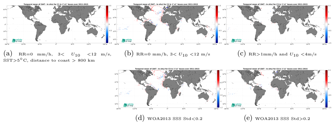
Figure 14: Temporal mean gridded over spatial boxes of size 1^\circ \times 1^\circ of \Delta\text{SSS} (Aquarius SSS L3 CAP v5 - 7-Day running (JPL) - TSG (GOSUD-Research-vessel)) for 5 different subdatasets corresponding to:RR=0 mm/h, 3 < U_{10} < 12 m/s, SST >5^\circ\text{C} , distance to coast > 800 km (a), RR=0 mm/h, 3 < U_{10} < 12 m/s (b), RR >1 mm/h and U_{10} < 4 m/s (c), WOA2013 SSS Std <0.2 (d), WOA2013 SSS Std >0.2 (e).
