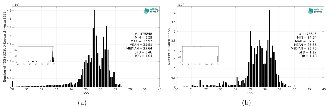
Figure 3: Histograms of SSS from TSG (GOSUD-Research-vessel) (a) and Aquarius SSS L3 CAP v5 - 7-Day running (JPL) (b) considering all match-up pairs per bins of 0.1 over the SMOS coastal zone (<800km) 60N-60S Pi-MEP region and for the full satellite product period.
