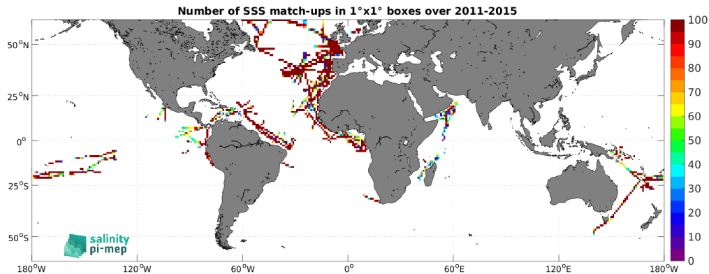
Figure 5: Number of SSS match-ups between TSG (GOSUD-Research-vessel) SSS and the Aquarius SSS L3 CAP v5 - 7-Day running (JPL) SSS product for the SMOS coastal zone ( <800\text{km} ) 60N-60S Pi-MEP region over 1^\circ \times 1^\circ boxes and for the full satellite product period.
