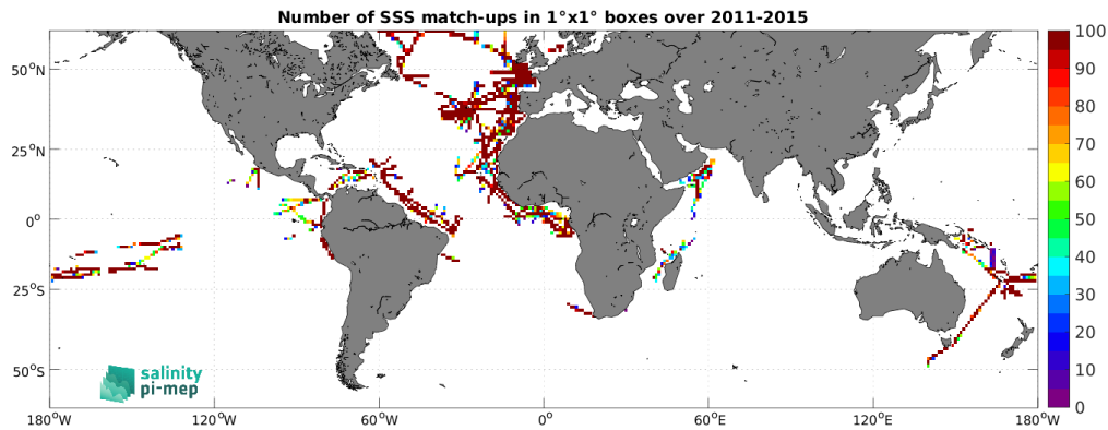
Figure 4: Number of SSS match-ups between TSG (GOSUD-Research-vessel) SSS and the Aquarius SSS L3 CAP v5 - 7-Day running (JPL) SSS product for the SMOS coastal zone ( <800\text{km} ) 60N-60S Pi-MEP region over 1^\circ \times 1^\circ boxes and for the full satellite product period.
