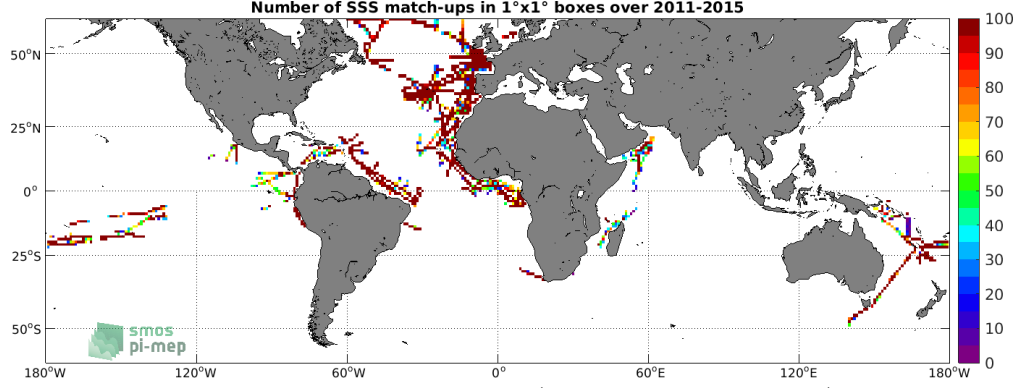
Figure 4: Number of SSS match-ups between TSG (GOSUD-Research-vessel) SSS and the Aquarius SSS L3 CAP v5 - 7-Day running (JPL) SSS product for the SMOS coastal zone (<800km) 60N-60S Pi-MEP region over 1°x1° boxes and for the full satellite product period.
