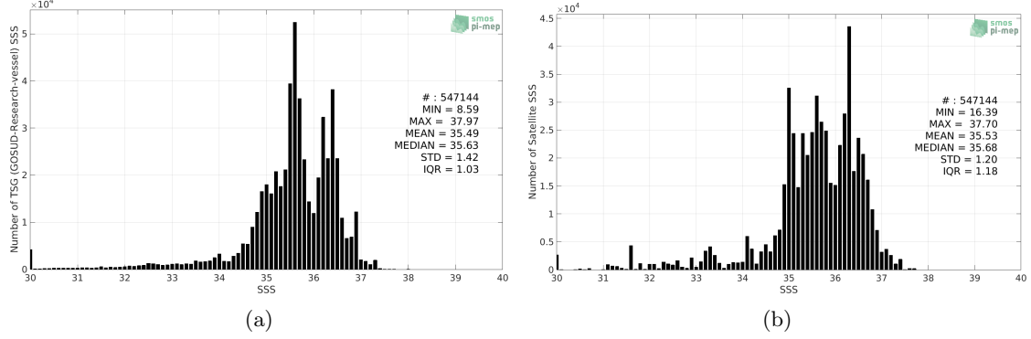
Figure 2: Histograms of SSS from TSG (GOSUD-Research-vessel) (a) and Aquarius SSS L3 CAP v5 - 7-Day running (JPL) (b) considering all match-up pairs per bins of 0.1 over the SMOS coastal zone (<800km) 60N-60S Pi-MEP region and for the full satellite product period.
