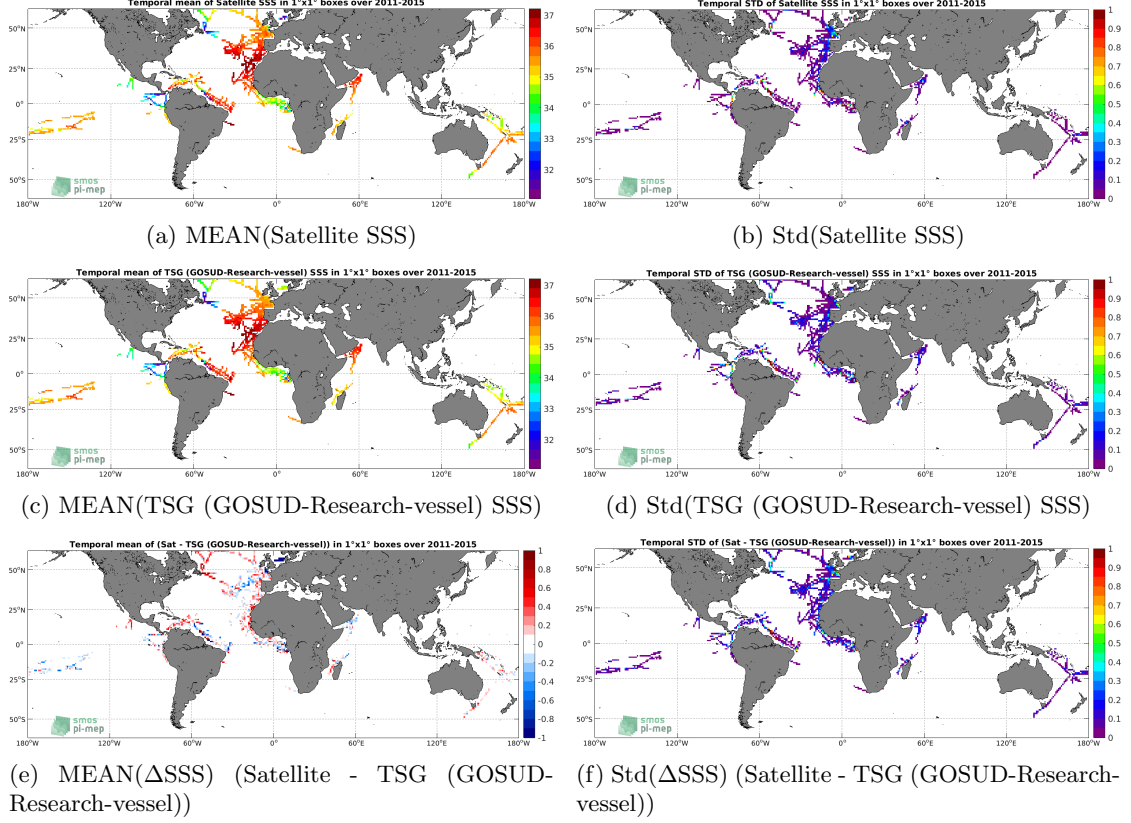
Figure 6: Temporal mean (left) and Std (right) of SSS from Aquarius SSS L3 CAP v5 - 7-Day running (JPL) (top), TSG (GOSUD-Research-vessel) (middle), and of \Delta SSS (Satellite - TSG (GOSUD-Research-vessel)). Only match-up pairs are used to generate these maps.
