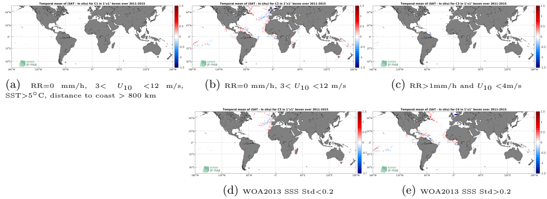
Figure 12: Temporal mean gridded over spatial boxes of size 1^\circ \times 1^\circ of \Delta SSS (Aquarius-L3-JPL-V5-7DAY-RUNNING - TSG-GOSUD-Research-vessel) for 5 different subdatasets corresponding to: RR=0 mm/h, 3 < U_{10} < 12 m/s, SST > 5^\circ\text{C} , distance to coast > 800 km (a), RR=0 mm/h, 3 < U_{10} < 12 m/s (b), RR > 1 mm/h and U_{10} < 4 m/s (c), WOA2013 SSS Std < 0.2 (d), WOA2013 SSS Std > 0.2 (e).
