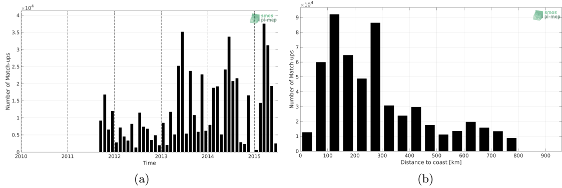
Figure 1: Number of match-ups between TSG-GOSUD-Research-vessel and Aquarius-L3-JPL-V5-7DAY-RUNNING SSS as a function of time (a) and as function of the distance to coast (b) over the SMOS coastal zone (<800km) 60N-60S Pi-MEP region and for the full satellite product period.
