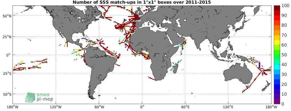
Figure 4: Number of SSS match-ups between TSG-GOSUD-Research-vessel SSS and the Aquarius-L3-JPL-V5-7DAY-RUNNING SSS product for the SMOS coastal zone (<800km) 60N-60S Pi-MEP region over 1°x1° boxes and for the full satellite product period.
