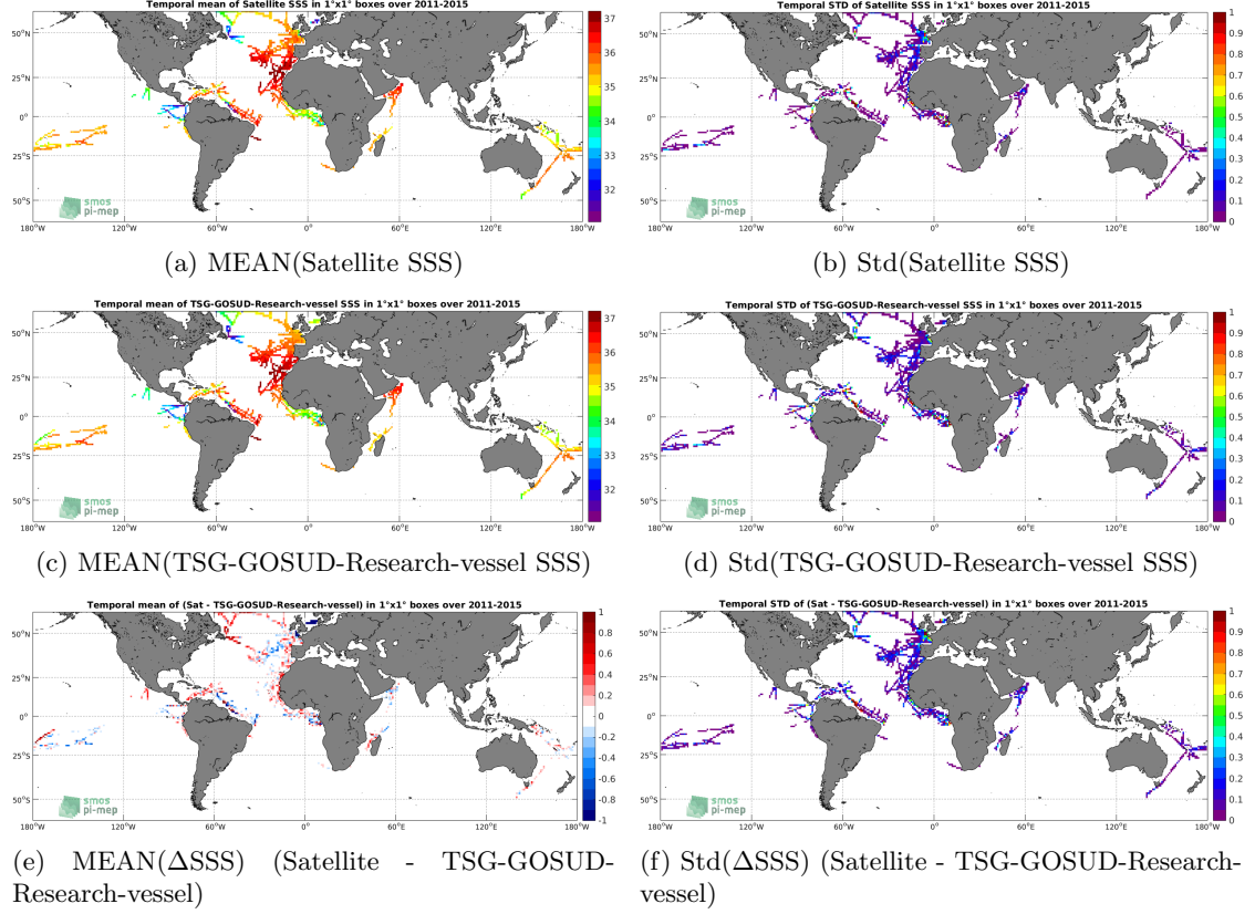
Figure 6: Temporal mean (left) and Std (right) of SSS from Aquarius-L3-JPL-V5-7DAY-RUNNING (top), TSG-GOSUD-Research-vessel (middle), and of \Delta SSS (Satellite - TSG-GOSUD-Research-vessel). Only match-up pairs are used to generate these maps.
