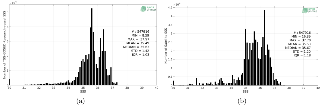
Figure 2: Histograms of SSS from TSG-GOSUD-Research-vessel (a) and Aquarius-L3-JPL-V5-7DAY-RUNNING (b) considering all match-up pairs per bins of 0.1 over the SMOS coastal zone (<800km) 60N-60S Pi-MEP region and for the full satellite product period.
