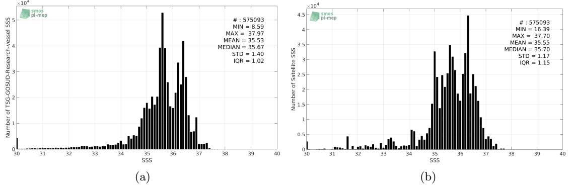
Figure 2: Histograms of SSS from TSG-GOSUD-Research-vessel (a) and Aquarius-L3-JPL-V5-7DAY-RUNNING (b) considering all match-up pairs per bins of 0.1 over the SMOS coastal zone ( \pm 800\text{km} ) 60N-60S Pi-MEP region and for the full satellite product period.
