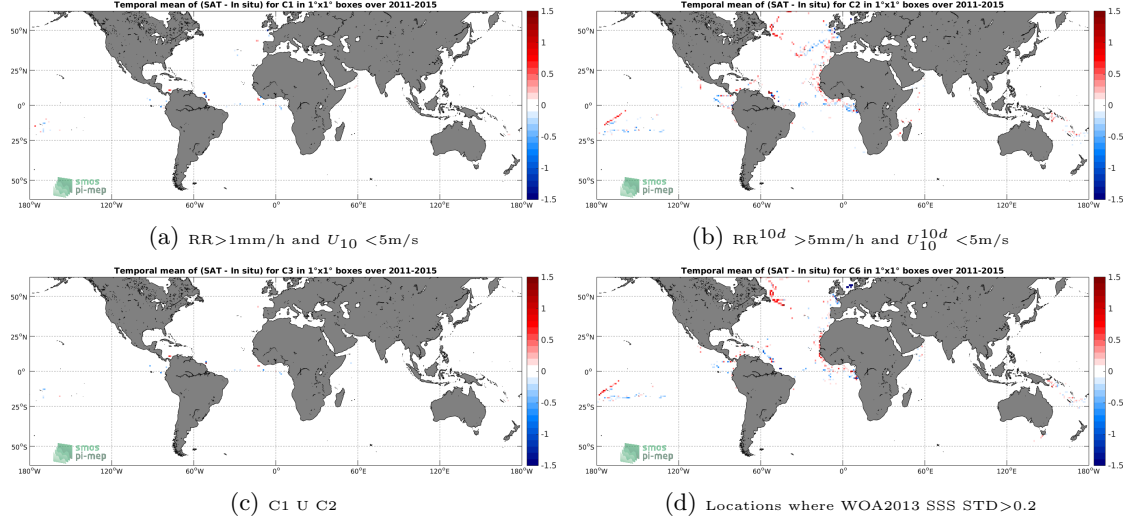
Figure 12: Temporal mean gridded over spatial boxes of size 1^\circ \times 1^\circ of \Delta SSS (Aquarius-L3-JPL-V5-7DAY-RUNNING - TSG-GOSUD-Research-vessel) for 4 different subdatasets corresponding to: RR > 1\text{mm/h} and U_{10} < 5\text{m/s} (a), RR^{10d} > 5\text{mm/h} and U_{10}^{10d} < 5\text{m/s} (b), C1 U C2 (c), Locations where WOA2013 SSS STD > 0.2 (d).
