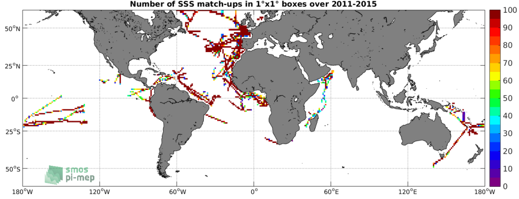
Figure 4: Number of SSS match-ups between TSG-GOSUD-Research-vessel SSS and the Aquarius-L3-JPL-V5-7DAY-RUNNING SSS product for the SMOS coastal zone ( \pm 800\text{km} ) 60N-60S Pi-MEP region over 1^\circ \times 1^\circ boxes and for the full satellite product period.
