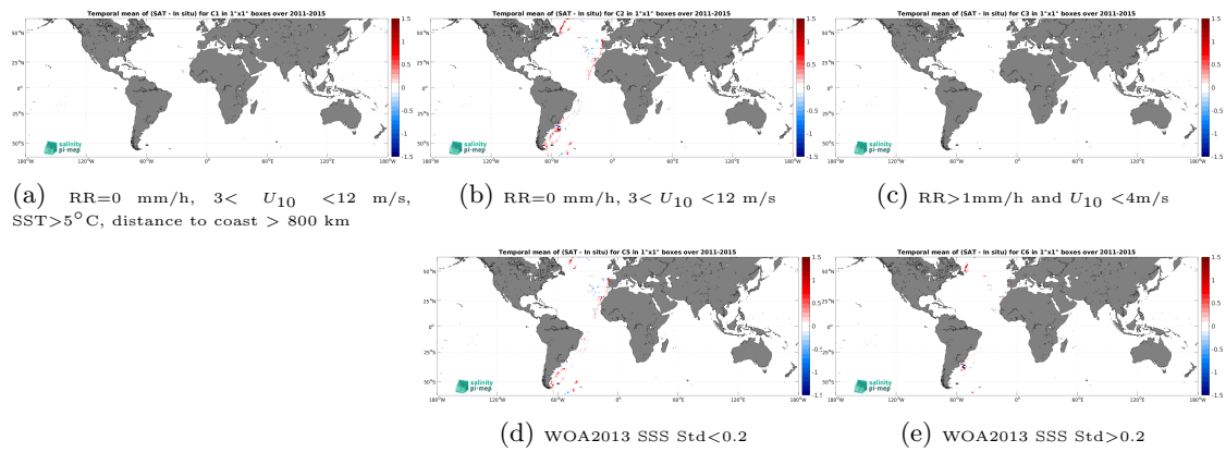
Figure 14: Temporal mean gridded over spatial boxes of size 1^\circ \times 1^\circ of \Delta\text{SSS} (Aquarius SSS L3 CAP v5 - 7-Day running (JPL) - TSG (CSIC-UTM)) for 5 different subdatasets corresponding to:RR=0 mm/h, 3 < U_{10} < 12 m/s, SST >5^\circ\text{C} , distance to coast > 800 km (a), RR=0 mm/h, 3 < U_{10} < 12 m/s (b), RR >1 mm/h and U_{10} < 4 m/s (c), WOA2013 SSS Std <0.2 (d), WOA2013 SSS Std >0.2 (e).
