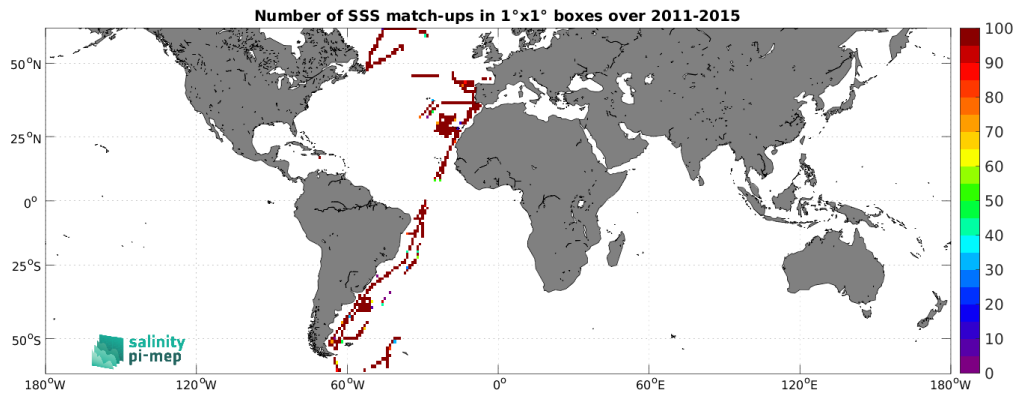
Figure 5: Number of SSS match-ups between TSG (CSIC-UTM) SSS and the Aquarius SSS L3 CAP v5 - 7-Day running (JPL) SSS product for the SMOS coastal zone (<800km) 60N-60S Pi-MEP region over 1^\circ \times 1^\circ boxes and for the full satellite product period.
