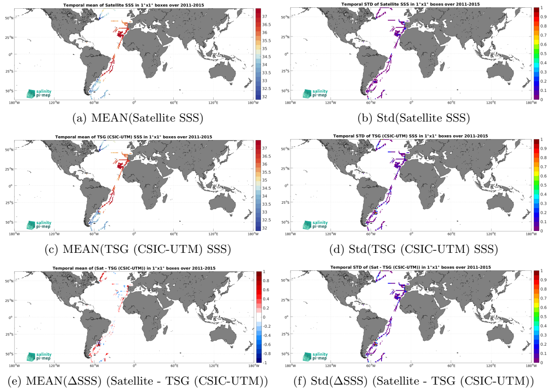
Figure 7: Temporal mean (left) and Std (right) of SSS from Aquarius SSS L3 CAP v5 - 7-Day running (JPL) (top), TSG (CSIC-UTM) (middle), and of \Delta SSS (Satellite - TSG (CSIC-UTM)). Only match-up pairs are used to generate these maps.
