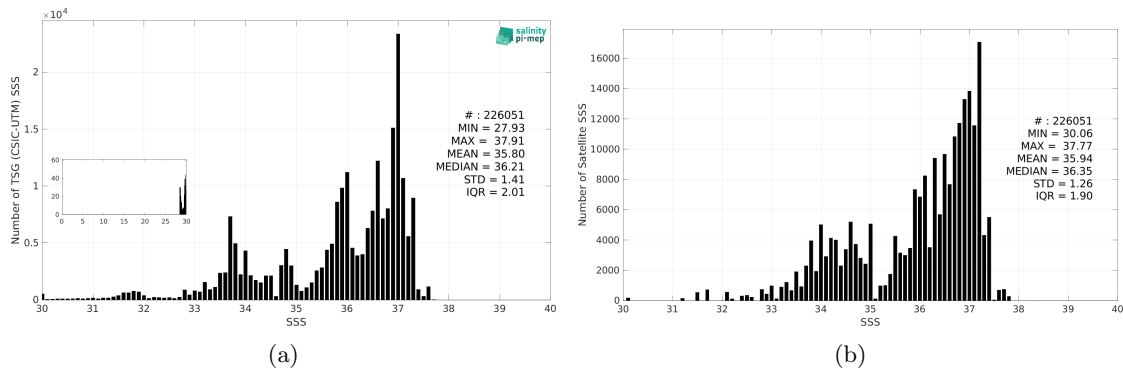
Figure 3: Histograms of SSS from TSG (CSIC-UTM) (a) and Aquarius SSS L3 CAP v5 - 7-Day running (JPL) (b) considering all match-up pairs per bins of 0.1 over the SMOS coastal zone (<800km) 60N-60S Pi-MEP region and for the full satellite product period.
