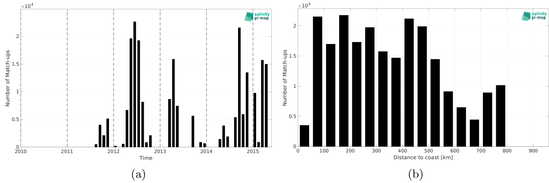
Figure 2: Number of match-ups between TSG (CSIC-UTM) and Aquarius SSS L3 CAP v5 - 7-Day running (JPL) SSS as a function of time (a) and as function of the distance to coast (b) over the SMOS coastal zone (<800km) 60N-60S Pi-MEP region and for the full satellite product period.
