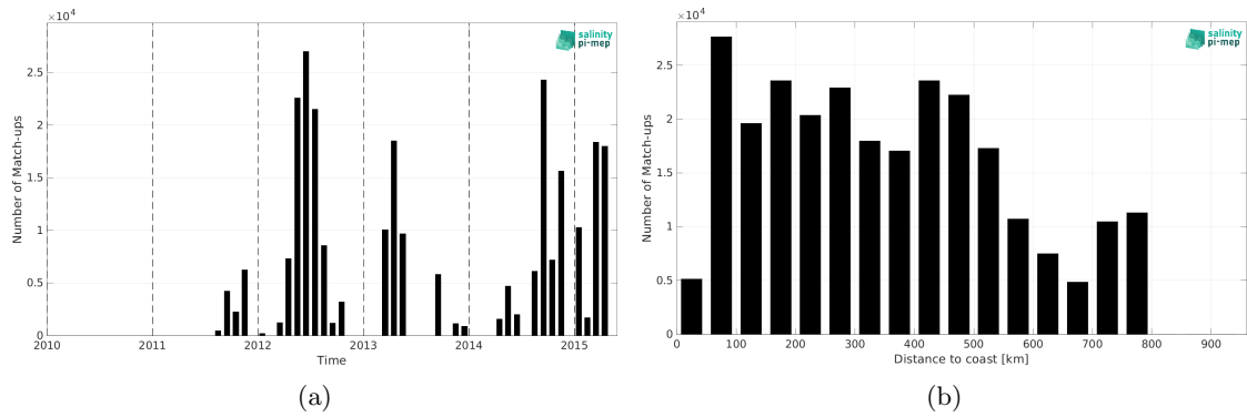
Figure 1: Number of match-ups between TSG (CSIC-UTM) and Aquarius SSS L3 CAP v5 - 7-Day running (JPL) SSS as a function of time (a) and as function of the distance to coast (b) over the SMOS coastal zone (<800km) 60N-60S Pi-MEP region and for the full satellite product period.
