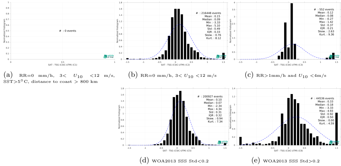
Figure 13: Normalized histogram of \Delta SSS (Aquarius SSS L3 CAP v5 - 7-Day running (JPL) - TSG (CSIC-UTM)) for 5 different subdatasets corresponding to: RR=0 mm/h, 3 < U_{10} < 12 m/s, SST > 5°C, distance to coast > 800 km (a), RR=0 mm/h, 3 < U_{10} < 12 m/s (b), RR > 1mm/h and U_{10} < 4 m/s (c), WOA2013 SSS Std < 0.2 (d), WOA2013 SSS Std > 0.2 (e).
