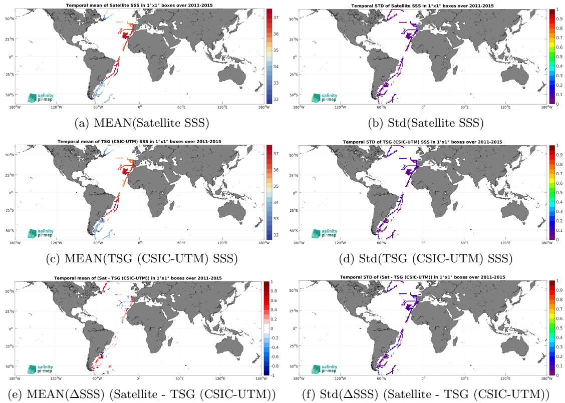
Figure 6: Temporal mean (left) and Std (right) of SSS from Aquarius SSS L3 CAP v5 - 7-Day running (JPL) (top), TSG (CSIC-UTM) (middle), and of \Delta SSS (Satellite - TSG (CSIC-UTM)). Only match-up pairs are used to generate these maps.
