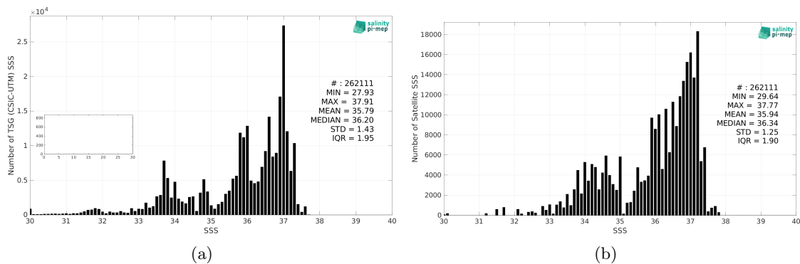
Figure 2: Histograms of SSS from TSG (CSIC-UTM) (a) and Aquarius SSS L3 CAP v5 - 7-Day running (JPL) (b) considering all match-up pairs per bins of 0.1 over the SMOS coastal zone (<800km) 60N-60S Pi-MEP region and for the full satellite product period.
