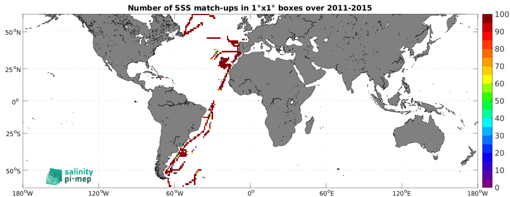
Figure 4: Number of SSS match-ups between TSG (CSIC-UTM) SSS and the Aquarius SSS L3 CAP v5 - 7-Day running (JPL) SSS product for the SMOS coastal zone (<800km) 60N-60S Pi-MEP region over 1^\circ \times 1^\circ boxes and for the full satellite product period.
