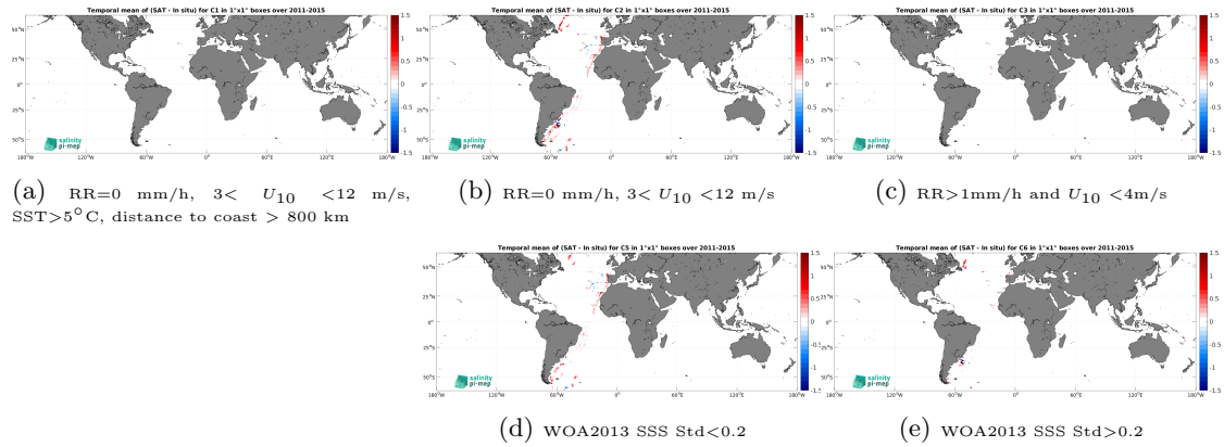
Figure 12: Temporal mean gridded over spatial boxes of size 1^\circ \times 1^\circ of \Delta\text{SSS} (Aquarius SSS L3 CAP v5 - 7-Day running (JPL) - TSG (CSIC-UTM)) for 5 different subdatasets corresponding to:RR=0 mm/h, 3 < U_{10} < 12 m/s, SST >5^\circ\text{C} , distance to coast > 800 km (a), RR=0 mm/h, 3 < U_{10} < 12 m/s (b), RR >1 mm/h and U_{10} < 4 m/s (c), WOA2013 SSS Std <0.2 (d), WOA2013 SSS Std >0.2 (e).
