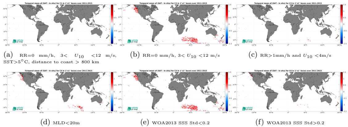
Figure 14: Temporal mean gridded over spatial boxes of size 1^\circ \times 1^\circ of \Delta SSS (Aquarius SSS L3 CAP v5 - 7-Day running (JPL) - Marine mammals) for 6 different subdatasets corresponding to:RR=0 mm/h, 3 < U_{10} < 12 m/s, SST>5°C, distance to coast > 800 km (a), RR=0 mm/h, 3 < U_{10} < 12 m/s (b), RR>1mm/h and U_{10} < 4 m/s (c),MLD<20m (d),WOA2013 SSS Std<0.2 (e),WOA2013 SSS Std>0.2 (f).
