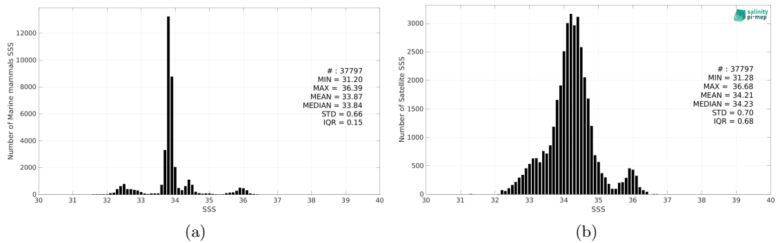
Figure 2: Histograms of SSS from Marine mammals (a) and Aquarius SSS L3 CAP v5 - 7-Day running (JPL) (b) considering all match-up pairs per bins of 0.1 over the SMOS coastal zone (<800km) 60N-60S Pi-MEP region and for the full satellite product period.
