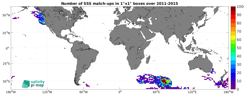
Figure 4: Number of SSS match-ups between Marine mammals SSS and the Aquarius SSS L3 CAP v5 - 7-Day running (JPL) SSS product for the SMOS coastal zone (<800km) 60N-60S Pi-MEP region over 1^\circ \times 1^\circ boxes and for the full satellite product period.
