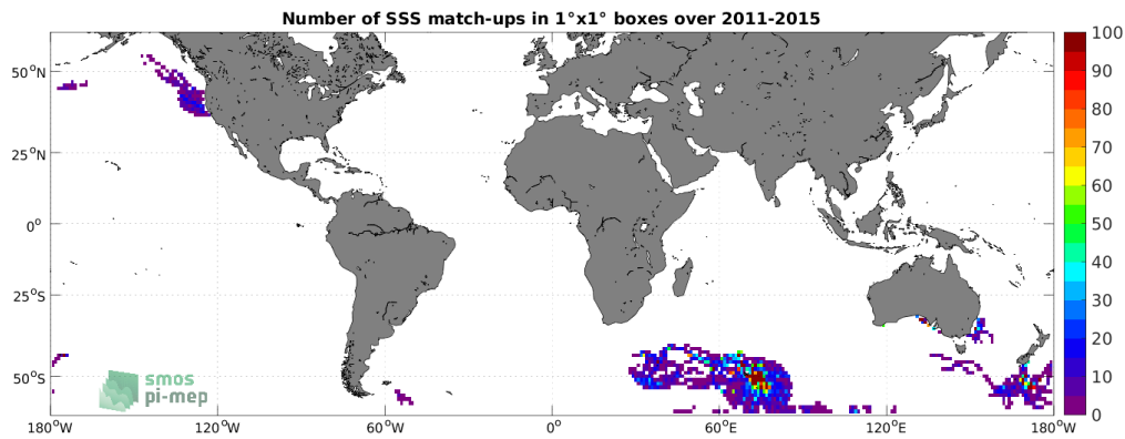
Figure 4: Number of SSS match-ups between Marine mammals SSS and the Aquarius SSS L3 CAP v5 - 7-Day running (JPL) SSS product for the SMOS coastal zone (<800km) 60N-60S Pi-MEP region over 1°×1° boxes and for the full satellite product period.
