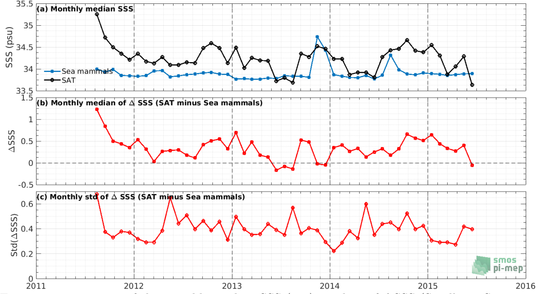
Figure 7: Time series of the monthly median SSS (top), median of \Delta SSS (Satellite - Sea mammals) and Std of \Delta SSS (Satellite - Sea mammals) over the SMOS coastal zone ( <800\text{km} ) 60\text{N} - 60\text{S} Pi-MEP region considering all match-ups collected by the Pi-MEP.
