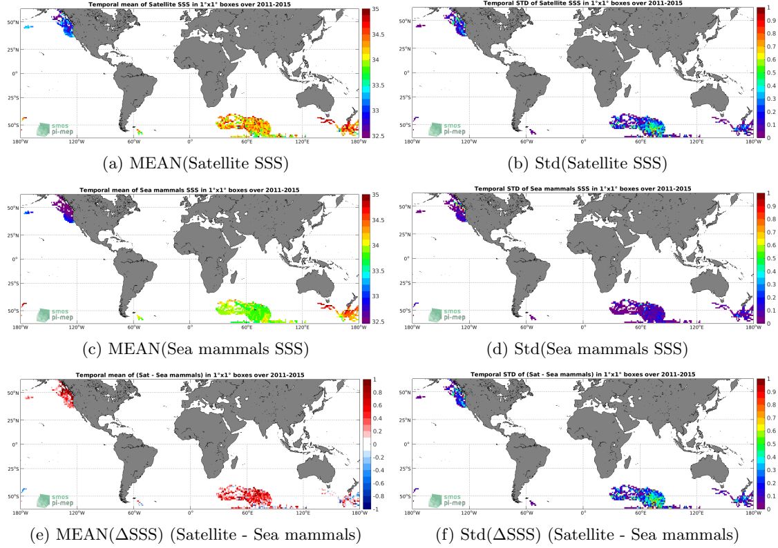
Figure 6: Temporal mean (left) and Std (right) of SSS from Aquarius SSS L3 CAP v5 - 7-Day running (JPL) (top), Sea mammals (middle), and of \Delta SSS (Satellite - Sea mammals). Only match-up pairs are used to generate these maps.
