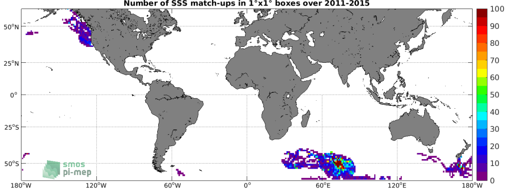
Figure 4: Number of SSS match-ups between Sea mammals SSS and the Aquarius SSS L3 CAP v5 - 7-Day running (JPL) SSS product for the SMOS coastal zone (<800km) 60N-60S Pi-MEP region over 1°x1° boxes and for the full satellite product period.
