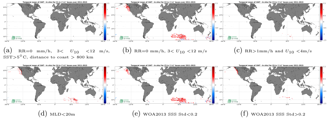
Figure 12: Temporal mean gridded over spatial boxes of size 1^\circ \times 1^\circ of \Delta SSS (Aquarius SSS L3 CAP v5 - 7-Day running (JPL) - Sea mammals) for 6 different subdatasets corresponding to: RR=0 mm/h, 3 < U_{10} < 12 m/s, SST > 5^\circ C , distance to coast > 800 km (a), RR=0 mm/h, 3 < U_{10} < 12 m/s (b), RR > 1 mm/h and U_{10} < 4 m/s (c), MLD < 20 m (d), WOA2013 SSS Std < 0.2 (e), WOA2013 SSS Std > 0.2 (f).
