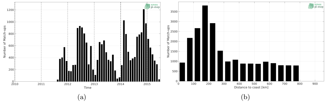
Figure 1: Number of match-ups between Sea mammals and Aquarius SSS L3 CAP v5 - 7-Day running (JPL) SSS as a function of time (a) and as function of the distance to coast (b) over the SMOS coastal zone (<800km) 60N-60S Pi-MEP region and for the full satellite product period.
