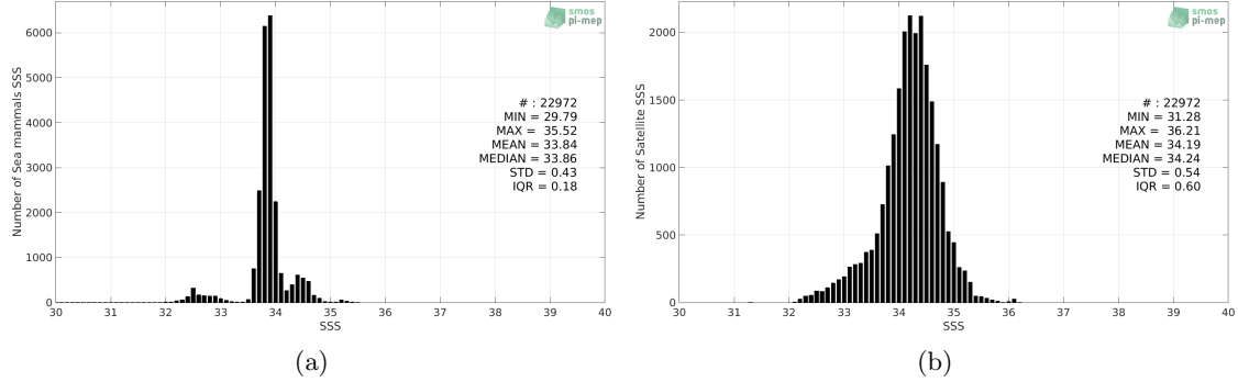
Figure 2: Histograms of SSS from Sea mammals (a) and Aquarius SSS L3 CAP v5 - 7-Day running (JPL) (b) considering all match-up pairs per bins of 0.1 over the SMOS coastal zone (<800km) 60N-60S Pi-MEP region and for the full satellite product period.
