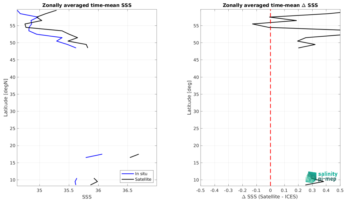
Figure 9: Left panel: Zonal mean SSS from Aquarius SSS L3 CAP v5 - 7-Day running (JPL) satellite product (black) and from ICES (blue). Right panel: Zonal mean of \Delta SSS (Satellite - ICES) for all the collected Pi-MEP match-up pairs estimated over the full satellite product period.
