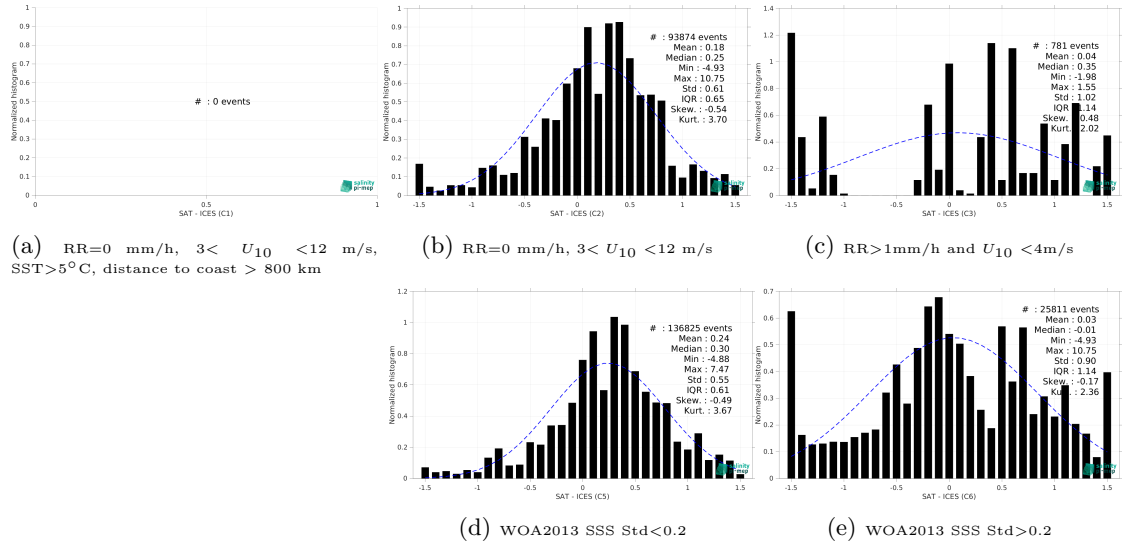
Figure 15: Normalized histogram of \Delta SSS (Aquarius SSS L3 CAP v5 - 7-Day running (JPL) - ICES) for 5 different subdatasets corresponding to: RR=0 mm/h, 3 < U_{10} < 12 m/s, SST > 5°C, distance to coast > 800 km (a), RR=0 mm/h, 3 < U_{10} < 12 m/s (b), RR > 1mm/h and U_{10} < 4 m/s (c), WOA2013 SSS Std < 0.2 (d), WOA2013 SSS Std > 0.2 (e).
