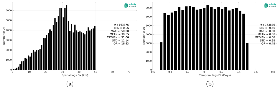
Figure 6: Histograms of the spatial (a) and temporal (b) lags between the location/time of the ICES measurement and the date of the corresponding Aquarius SSS L3 CAP v5 - 7-Day running (JPL) SSS pixel.
