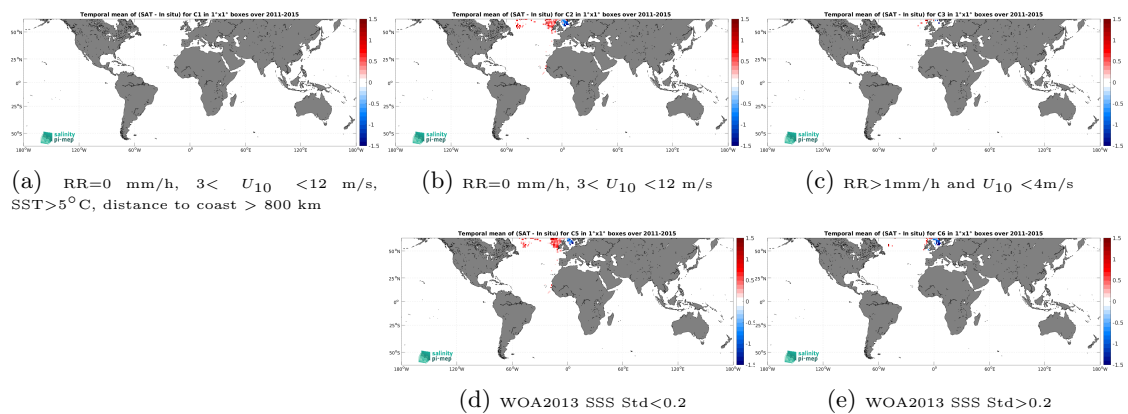
Figure 14: Temporal mean gridded over spatial boxes of size 1^\circ \times 1^\circ of \Delta SSS (Aquarius SSS L3 CAP v5 - 7-Day running (JPL) - ICES) for 5 different subdatasets corresponding to:RR=0 mm/h, 3 < U_{10} < 12 m/s, SST > 5^\circ\text{C} , distance to coast > 800 km (a), RR=0 mm/h, 3 < U_{10} < 12 m/s (b), RR > 1 mm/h and U_{10} < 4 m/s (c), WOA2013 SSS Std < 0.2 (d), WOA2013 SSS Std > 0.2 (e).
