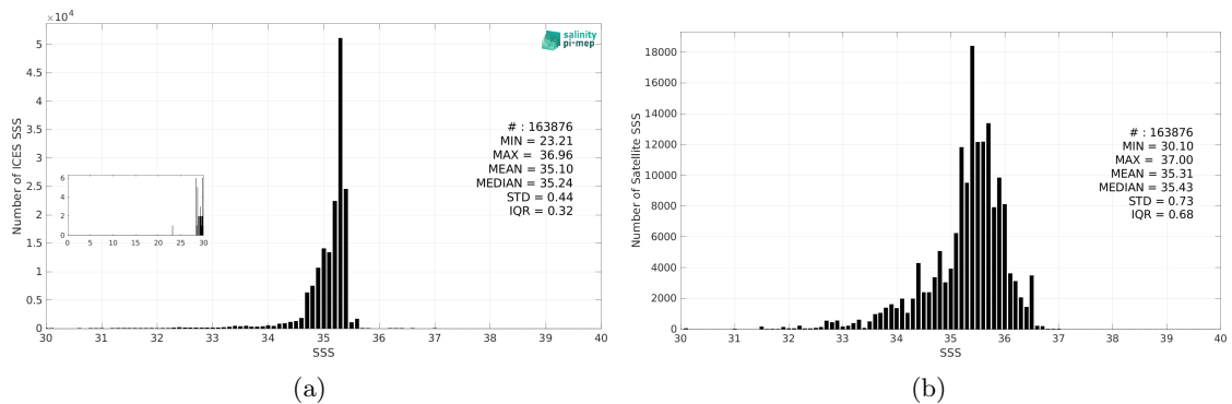
Figure 3: Histograms of SSS from ICES (a) and Aquarius SSS L3 CAP v5 - 7-Day running (JPL) (b) considering all match-up pairs per bins of 0.1 over the SMOS coastal zone (<800km) 60N-60S Pi-MEP region and for the full satellite product period.
