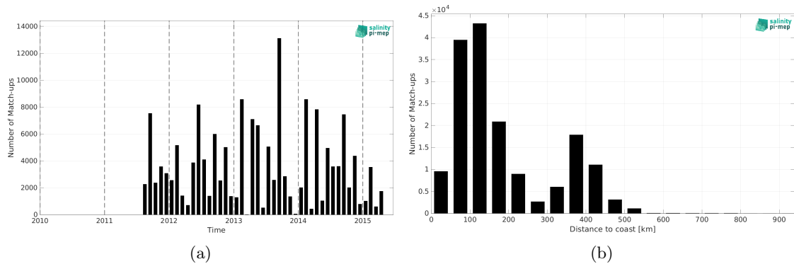
Figure 2: Number of match-ups between ICES and Aquarius SSS L3 CAP v5 - 7-Day running (JPL) SSS as a function of time (a) and as function of the distance to coast (b) over the SMOS coastal zone (<800km) 60N-60S Pi-MEP region and for the full satellite product period.
