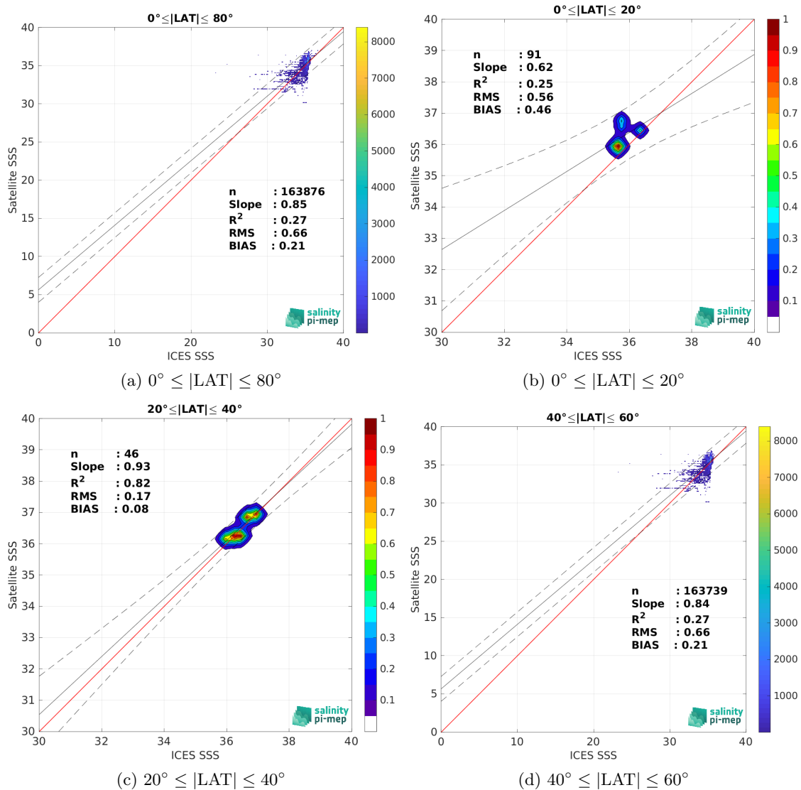
Figure 10: Contour maps of the concentration of Aquarius SSS L3 CAP v5 - 7-Day running (JPL) SSS (y-axis) versus ICES SSS (x-axis) at match-up pairs for different latitude bands. For each plot, the red line shows x=y . The black thin and dashed lines indicate a linear fit through the data cloud and the \pm 95\% confidence levels, respectively. The number match-up pairs n , the slope and R^2 coefficient of the linear fit, the root mean square (RMS) and the mean bias between satellite and in situ data are indicated for each latitude band in each plots.
