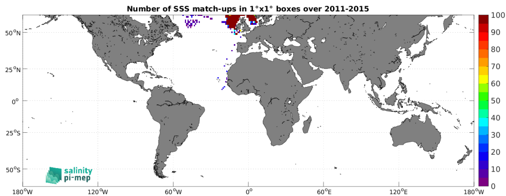
Figure 5: Number of SSS match-ups between ICES SSS and the Aquarius SSS L3 CAP v5 - 7-Day running (JPL) SSS product for the SMOS coastal zone (<800km) 60N-60S Pi-MEP region over 1^\circ \times 1^\circ boxes and for the full satellite product period.
