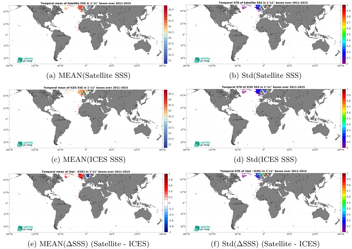
Figure 7: Temporal mean (left) and Std (right) of SSS from Aquarius SSS L3 CAP v5 - 7-Day running (JPL) (top), ICES (middle), and of \Delta SSS (Satellite - ICES). Only match-up pairs are used to generate these maps.
