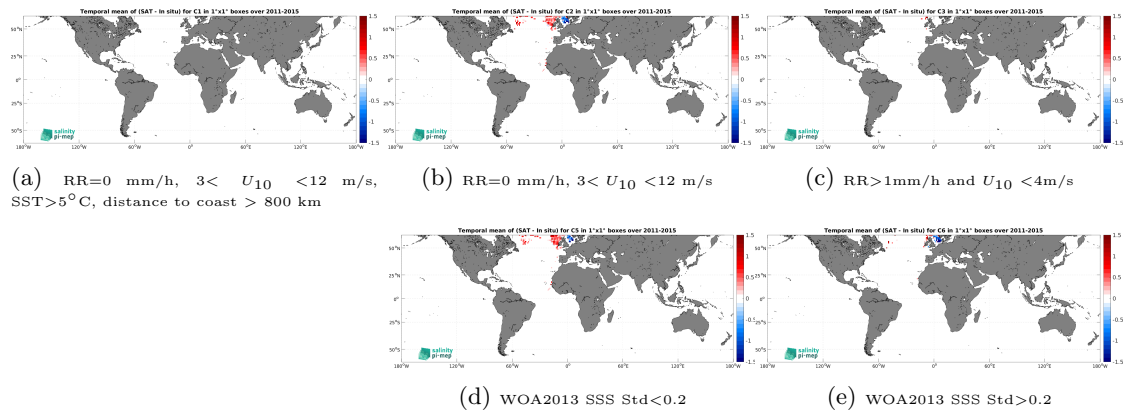
Figure 12: Temporal mean gridded over spatial boxes of size 1^\circ \times 1^\circ of \Delta\text{SSS} (Aquarius SSS L3 CAP v5 - 7-Day running (JPL) - ICES) for 5 different subdatasets corresponding to:RR=0 mm/h, 3 < U_{10} < 12 m/s, SST >5^\circ\text{C} , distance to coast > 800 km (a), RR=0 mm/h, 3 < U_{10} < 12 m/s (b), RR >1 mm/h and U_{10} < 4 m/s (c), WOA2013 SSS Std <0.2 (d), WOA2013 SSS Std >0.2 (e).
