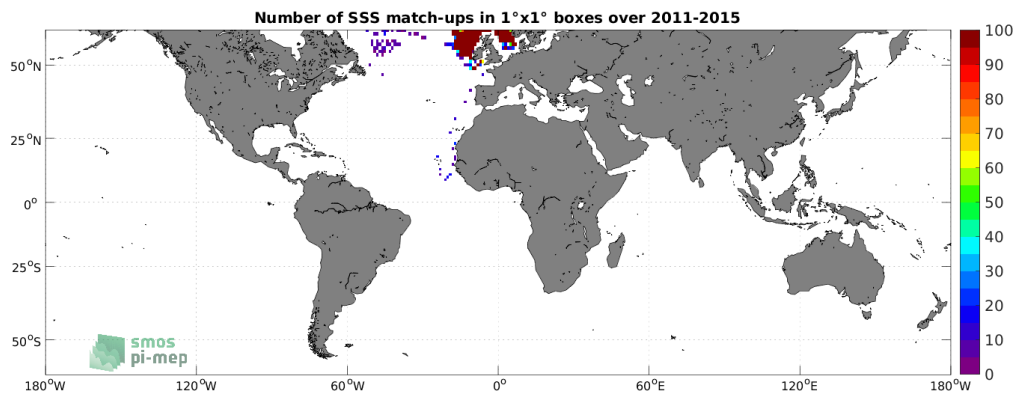
Figure 4: Number of SSS match-ups between ICES SSS and the Aquarius SSS L3 CAP v5 - 7-Day running (JPL) SSS product for the SMOS coastal zone (<800km) 60N-60S Pi-MEP region over 1^\circ \times 1^\circ boxes and for the full satellite product period.
