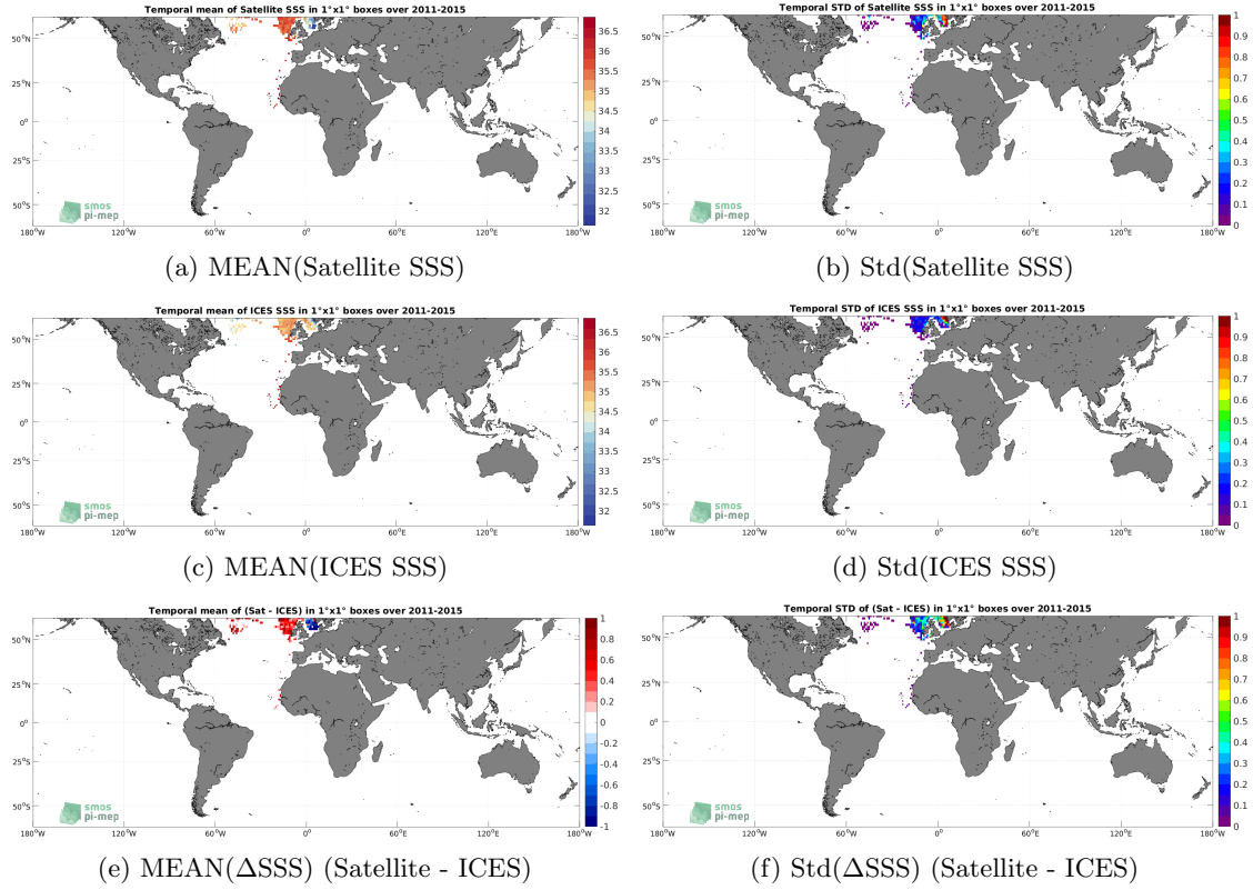
Figure 6: Temporal mean (left) and Std (right) of SSS from Aquarius SSS L3 CAP v5 - 7-Day running (JPL) (top), ICES (middle), and of \Delta SSS (Satellite - ICES). Only match-up pairs are used to generate these maps.
