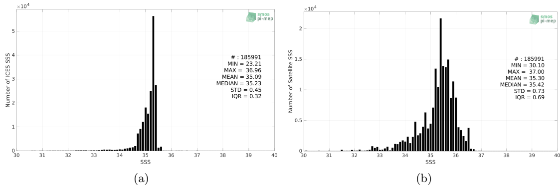
Figure 2: Histograms of SSS from ICES (a) and Aquarius SSS L3 CAP v5 - 7-Day running (JPL) (b) considering all match-up pairs per bins of 0.1 over the SMOS coastal zone (<800km) 60N-60S Pi-MEP region and for the full satellite product period.
