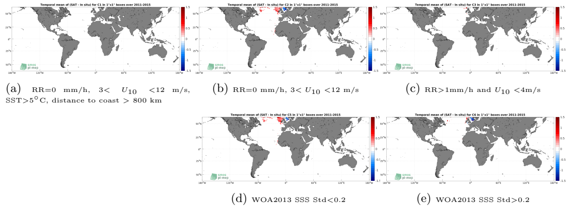
Figure 12: Temporal mean gridded over spatial boxes of size 1^\circ \times 1^\circ of \Delta SSS (Aquarius SSS L3 CAP v5 - 7-Day running (JPL) - ICES) for 5 different subdatasets corresponding to:RR=0 mm/h, 3 < U_{10} < 12 m/s, SST >5^\circ\text{C} , distance to coast > 800 km (a), RR=0 mm/h, 3 < U_{10} < 12 m/s (b), RR >1 mm/h and U_{10} < 4 m/s (c), WOA2013 SSS Std <0.2 (d), WOA2013 SSS Std >0.2 (e).
