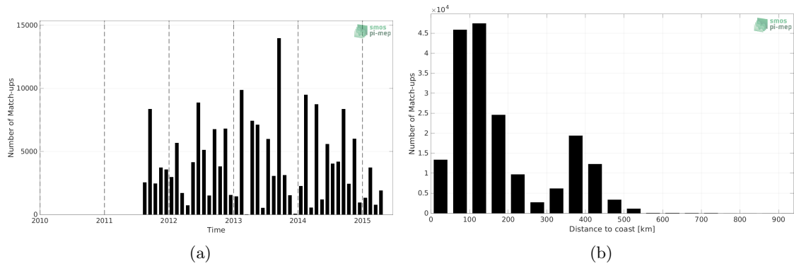
Figure 1: Number of match-ups between ICES and Aquarius SSS L3 CAP v5 - 7-Day running (JPL) SSS as a function of time (a) and as function of the distance to coast (b) over the SMOS coastal zone (<800km) 60N-60S Pi-MEP region and for the full satellite product period.
