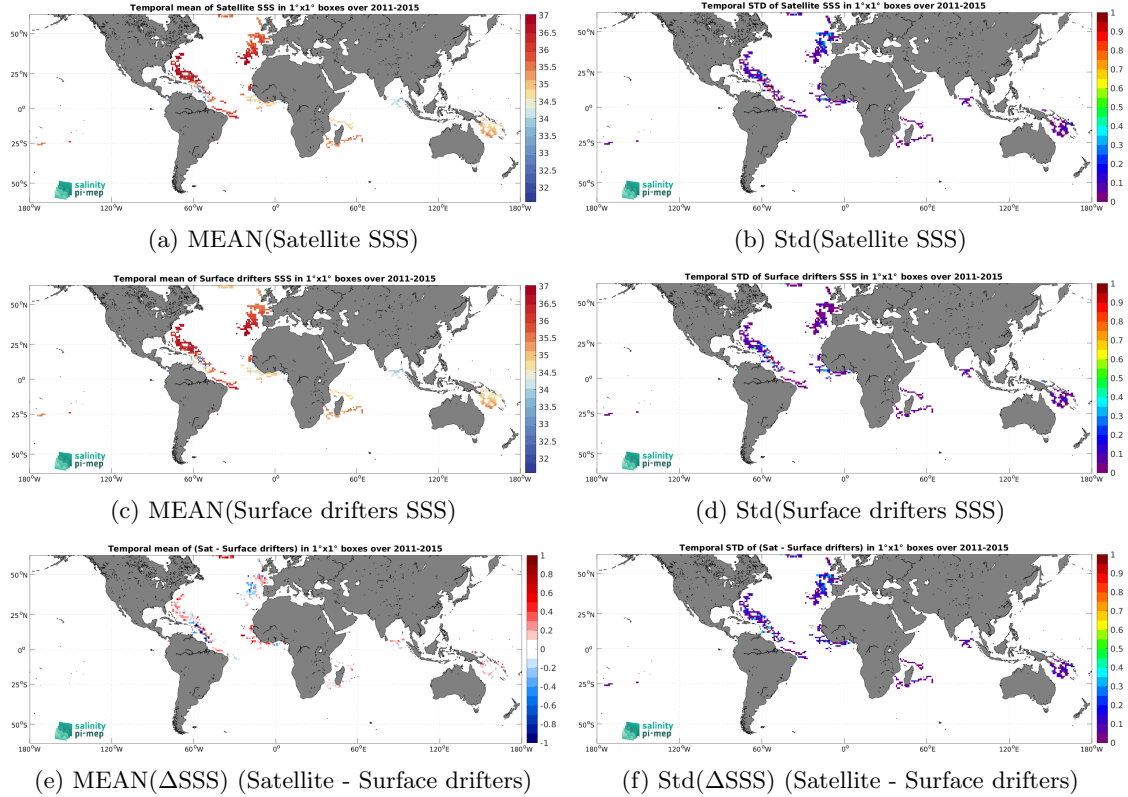
Figure 6: Temporal mean (left) and Std (right) of SSS from Aquarius SSS L3 CAP v5 - 7-Day running (JPL) (top), Surface drifters (middle), and of \Delta SSS (Satellite - Surface drifters). Only match-up pairs are used to generate these maps.
