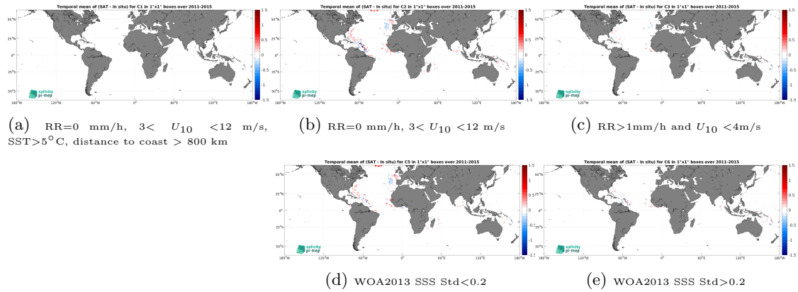
Figure 13: Temporal mean gridded over spatial boxes of size 1^\circ \times 1^\circ of \Delta\text{SSS} (Aquarius SSS L3 CAP v5 - 7-Day running (JPL) - Surface drifters) for 5 different subdatasets corresponding to:RR=0 mm/h, 3 < U_{10} < 12 m/s, SST >5^\circ\text{C} , distance to coast > 800 km (a), RR=0 mm/h, 3 < U_{10} < 12 m/s (b), RR >1 mm/h and U_{10} < 4 m/s (c), WOA2013 SSS Std <0.2 (d), WOA2013 SSS Std >0.2 (e).
