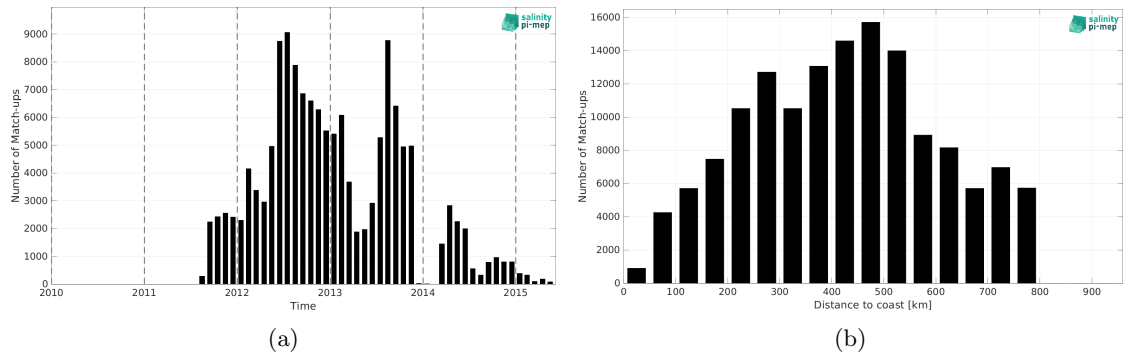
Figure 2: Number of match-ups between Surface drifters and Aquarius SSS L3 CAP v5 - 7-Day running (JPL) SSS as a function of time (a) and as function of the distance to coast (b) over the SMOS coastal zone (<800km) 60N-60S Pi-MEP region and for the full satellite product period.
