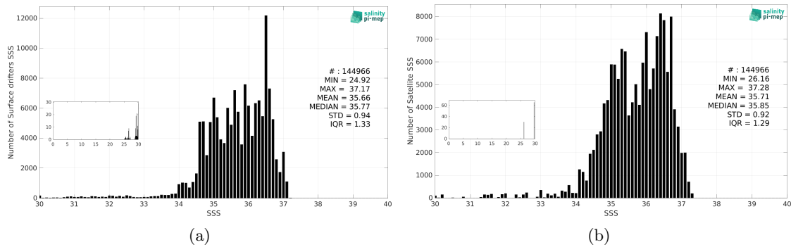
Figure 3: Histograms of SSS from Surface drifters (a) and Aquarius SSS L3 CAP v5 - 7-Day running (JPL) (b) considering all match-up pairs per bins of 0.1 over the SMOS coastal zone (<800km) 60N-60S Pi-MEP region and for the full satellite product period.
