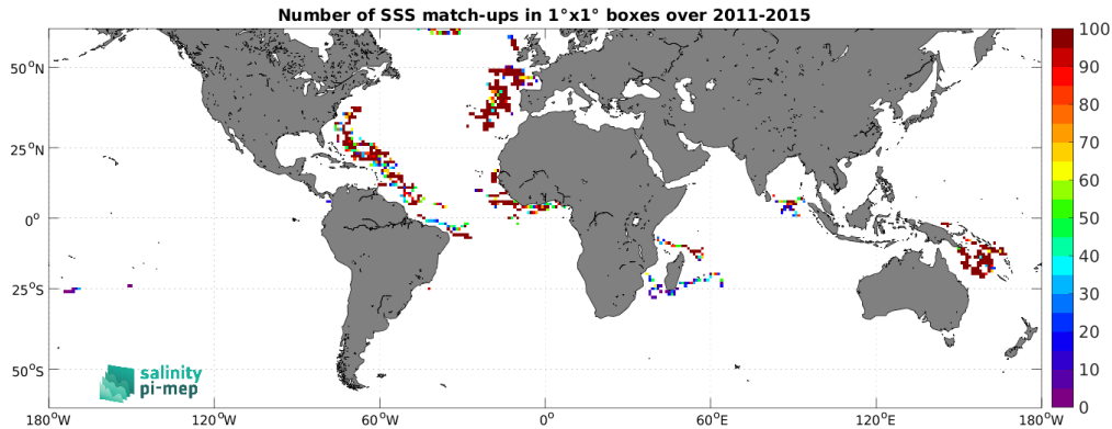
Figure 4: Number of SSS match-ups between Surface drifters SSS and the Aquarius SSS L3 CAP v5 - 7-Day running (JPL) SSS product for the SMOS coastal zone ( <800\text{km} ) 60N-60S Pi-MEP region over 1^\circ \times 1^\circ boxes and for the full satellite product period.
