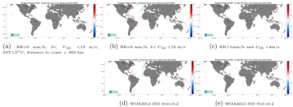
Figure 13: Temporal mean gridded over spatial boxes of size 1^\circ \times 1^\circ of \Delta SSS (Aquarius SSS L3 CAP v5 - 7-Day running (JPL) - Surface drifters) for 5 different subdatasets corresponding to:RR=0 mm/h, 3 < U_{10} < 12 m/s, SST >5^\circ C, distance to coast > 800 km (a), RR=0 mm/h, 3 < U_{10} < 12 m/s (b), RR >1 mm/h and U_{10} < 4 m/s (c), WOA2013 SSS Std <0.2 (d), WOA2013 SSS Std >0.2 (e).
