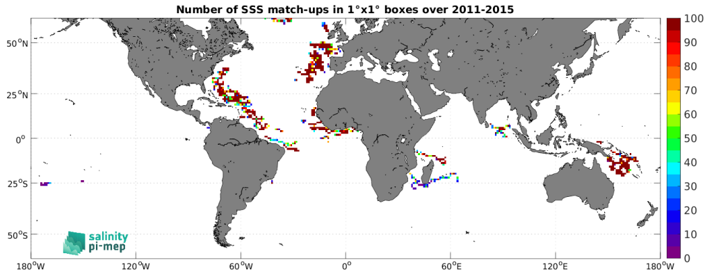
Figure 3: Number of SSS match-ups between Surface drifters SSS and the Aquarius SSS L3 CAP v5 - 7-Day running (JPL) SSS product for the SMOS coastal zone ( <800\text{km} ) 60N-60S Pi-MEP region over 1^\circ \times 1^\circ boxes and for the full satellite product period.
