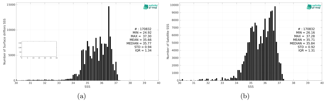
Figure 2: Histograms of SSS from Surface drifters (a) and Aquarius SSS L3 CAP v5 - 7-Day running (JPL) (b) considering all match-up pairs per bins of 0.1 over the SMOS coastal zone (<800km) 60N-60S Pi-MEP region and for the full satellite product period.
