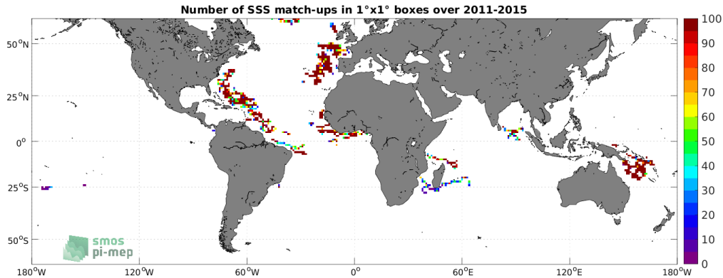
Figure 3: Number of SSS match-ups between Surface drifters SSS and the Aquarius SSS L3 CAP v5 - 7-Day running (JPL) SSS product for the SMOS coastal zone (<800km) 60N-60S Pi-MEP region over 1^\circ \times 1^\circ boxes and for the full satellite product period.
