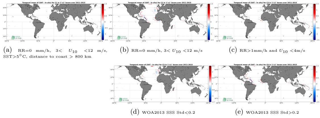
Figure 11: Temporal mean gridded over spatial boxes of size 1^\circ \times 1^\circ of \Delta SSS (Aquarius SSS L3 CAP v5 - 7-Day running (JPL) - Surface drifters) for 5 different subdatasets corresponding to: RR=0 mm/h, 3 < U_{10} < 12 m/s, SST >5^\circ C, distance to coast > 800 km (a), RR=0 mm/h, 3 < U_{10} < 12 m/s (b), RR >1 mm/h and U_{10} < 4 m/s (c), WOA2013 SSS Std <0.2 (d), WOA2013 SSS Std >0.2 (e).
