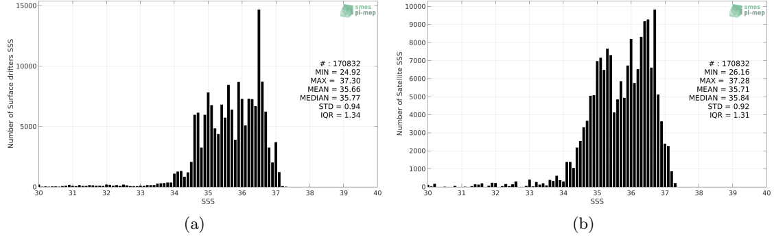
Figure 2: Histograms of SSS from Surface drifters (a) and Aquarius SSS L3 CAP v5 - 7-Day running (JPL) (b) considering all match-up pairs per bins of 0.1 over the SMOS coastal zone (<800km) 60N-60S Pi-MEP region and for the full satellite product period.
