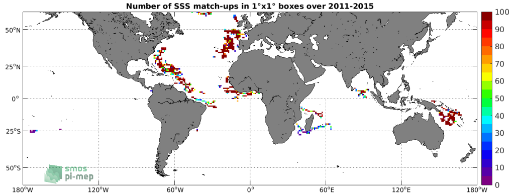
Figure 3: Number of SSS match-ups between Surface drifters SSS and the Aquarius SSS L3 CAP v5 - 7-Day running (JPL) SSS product for the SMOS coastal zone (<800km) 60N-60S Pi-MEP region over 1°x1° boxes and for the full satellite product period.
