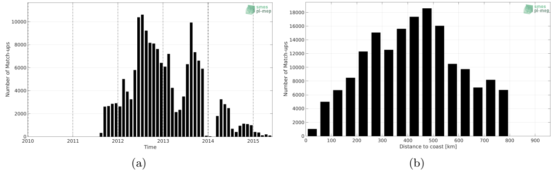
Figure 1: Number of match-ups between Surface drifters and Aquarius SSS L3 CAP v5 - 7-Day running (JPL) SSS as a function of time (a) and as function of the distance to coast (b) over the SMOS coastal zone (<800km) 60N-60S Pi-MEP region and for the full satellite product period.
