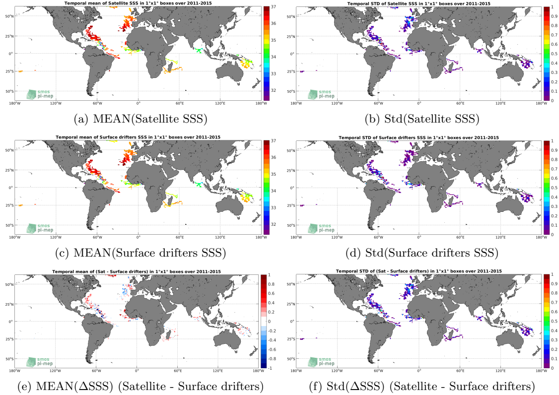
Figure 5: Temporal mean (left) and Std (right) of SSS from Aquarius SSS L3 CAP v5 - 7-Day running (JPL) (top), Surface drifters (middle), and of \Delta SSS (Satellite - Surface drifters). Only match-up pairs are used to generate these maps.
