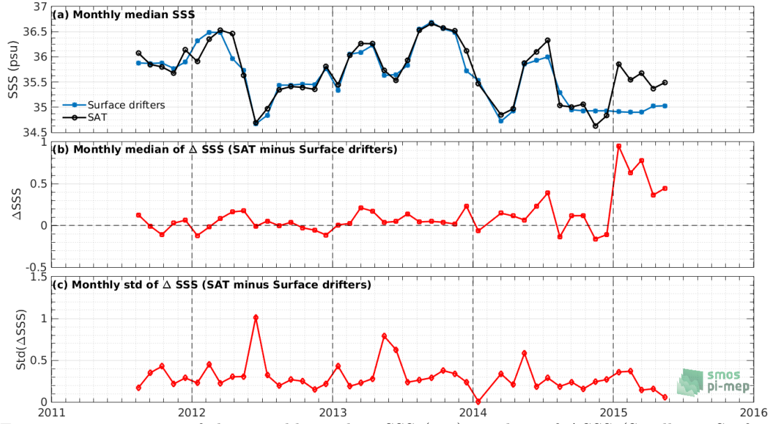
Figure 6: Time series of the monthly median SSS (top), median of \Delta\text{SSS} (Satellite - Surface drifters) and Std of \Delta\text{SSS} (Satellite - Surface drifters) over the SMOS coastal zone ( <800\text{km} ) 60\text{N} - 60\text{S} Pi-MEP region considering all match-ups collected by the Pi-MEP.
