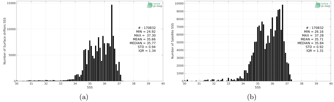
Figure 2: Histograms of SSS from Surface drifters (a) and Aquarius-L3-JPL-V5-7DAY-RUNNING (b) considering all match-up pairs per bins of 0.1 over the SMOS coastal zone (<800km) 60N-60S Pi-MEP region and for the full satellite product period.
