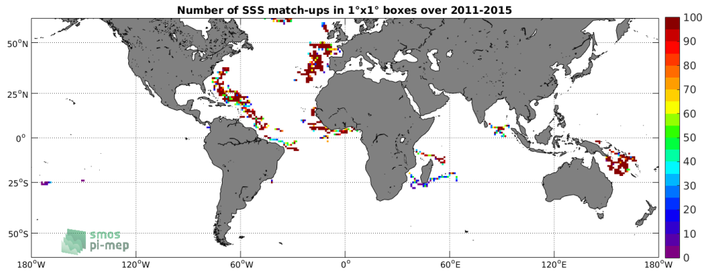
Figure 3: Number of SSS match-ups between Surface drifters SSS and the Aquarius-L3-JPL-V5-7DAY-RUNNING SSS product for the SMOS coastal zone (<800km) 60N-60S Pi-MEP region over 1°x1° boxes and for the full satellite product period.
