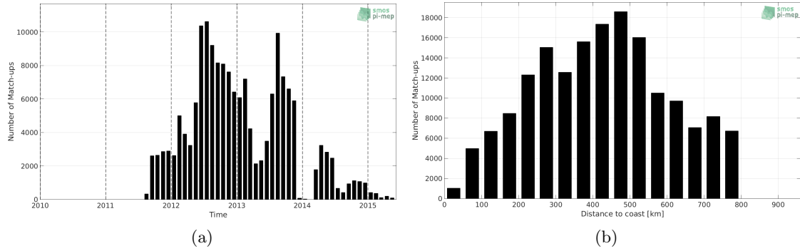
Figure 1: Number of match-ups between Surface drifters and Aquarius-L3-JPL-V5-7DAY-RUNNING SSS as a function of time (a) and as function of the distance to coast (b) over the SMOS coastal zone (<800km) 60N-60S Pi-MEP region and for the full satellite product period.
