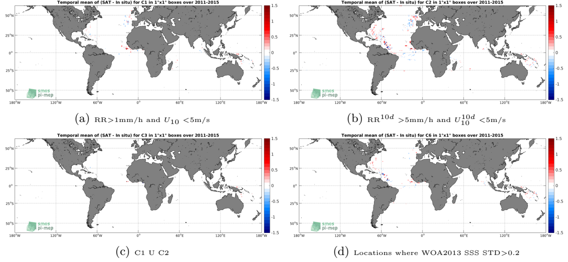
Figure 11: Temporal mean gridded over spatial boxes of size 1^\circ \times 1^\circ of \Delta SSS (Aquarius-L3-JPL-V5-7DAY-RUNNING - Surface drifters) for 4 different subdatasets corresponding to: RR > 1\text{mm/h} and U_{10} < 5\text{m/s} (a), RR^{10d} > 5\text{mm/h} and U_{10}^{10d} < 5\text{m/s} (b), C1 U C2 (c), Locations where WOA2013 SSS STD > 0.2 (d).
