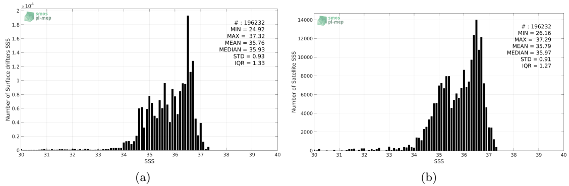
Figure 2: Histograms of SSS from Surface drifters (a) and Aquarius-L3-JPL-V5-7DAY-RUNNING (b) considering all match-up pairs per bins of 0.1 over the SMOS coastal zone ( \pm 800\text{km} ) 60N-60S Pi-MEP region and for the full satellite product period.
