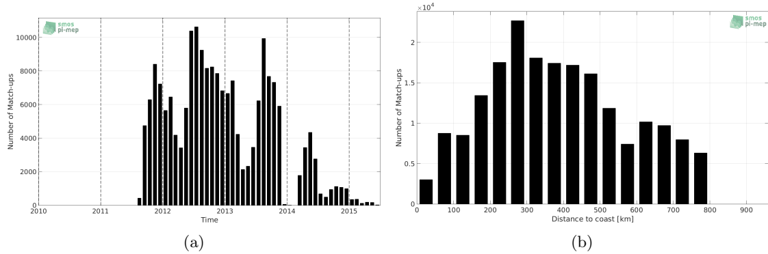
Figure 1: Number of match-ups between Surface drifters and Aquarius-L3-JPL-V5-7DAY-RUNNING SSS as a function of time (a) and as function of the distance to coast (b) over the SMOS coastal zone ( \pm 800 km) 60N-60S Pi-MEP region and for the full satellite product period.
