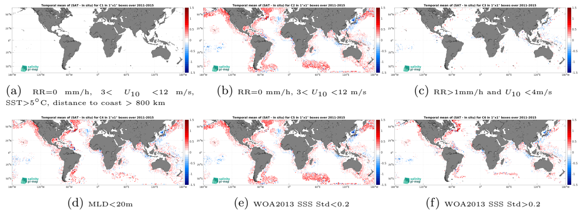
Figure 14: Temporal mean gridded over spatial boxes of size 1^\circ \times 1^\circ of \Delta SSS (Aquarius SSS L3 CAP v5 - 7-Day running (JPL) - Argo) for 6 different subdatasets corresponding to:RR=0 mm/h, 3 < U_{10} < 12 m/s, SST >5^\circ C, distance to coast > 800 km (a), RR=0 mm/h, 3 < U_{10} < 12 m/s (b), RR >1 mm/h and U_{10} < 4 m/s (c),MLD <20 m (d),WOA2013 SSS Std <0.2 (e),WOA2013 SSS Std >0.2 (f).
