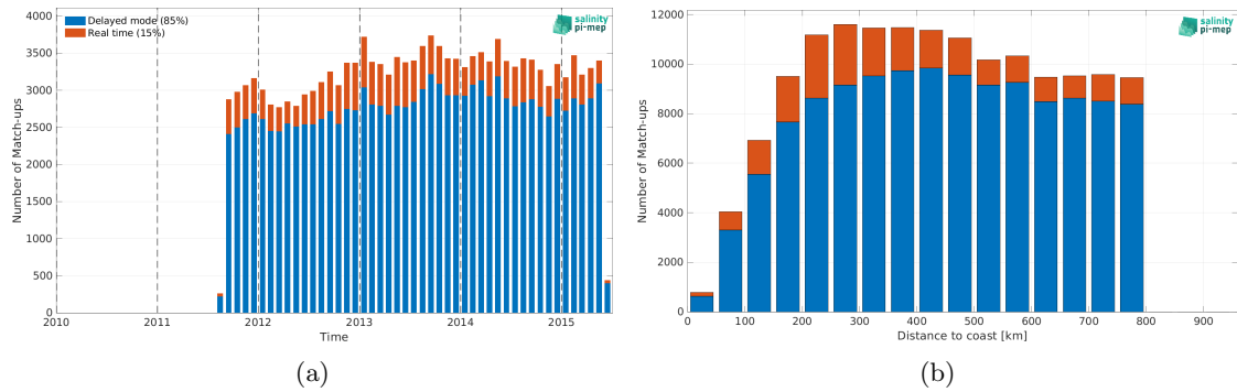
Figure 2: Number of match-ups between Argo and Aquarius SSS L3 CAP v5 - 7-Day running (JPL) SSS as a function of time (a) and as function of the distance to coast (b) over the SMOS coastal zone (<800km) 60N-60S Pi-MEP region and for the full satellite product period.
