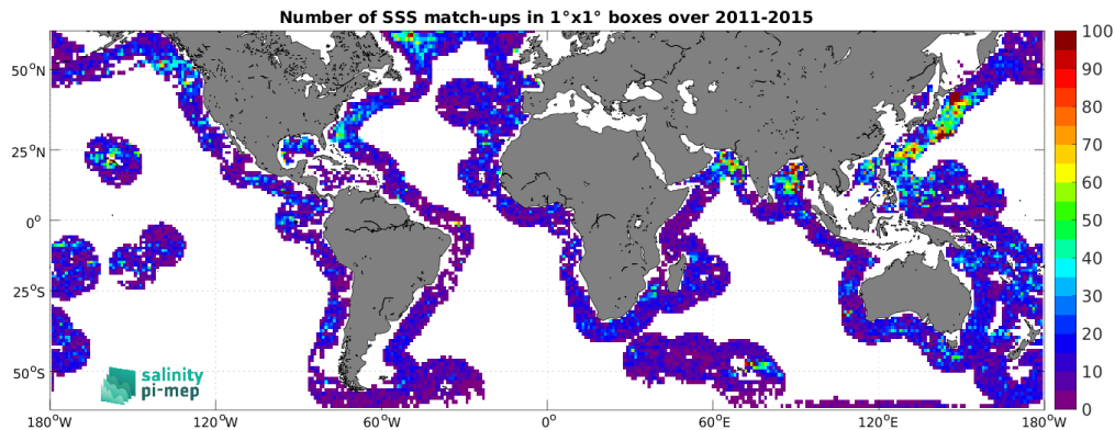
Figure 5: Number of SSS match-ups between Argo SSS and the Aquarius SSS L3 CAP v5 - 7-Day running (JPL) SSS product for the SMOS coastal zone (<800km) 60N-60S Pi-MEP region over 1^\circ \times 1^\circ boxes and for the full satellite product period.
