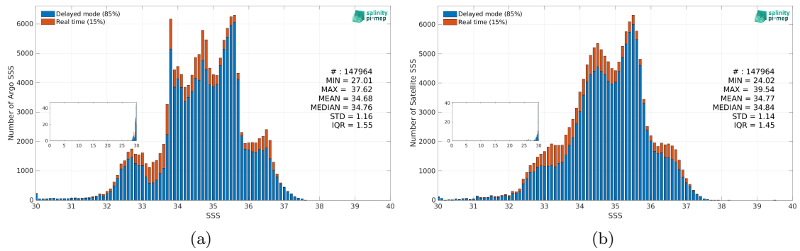
Figure 3: Histograms of SSS from Argo (a) and Aquarius SSS L3 CAP v5 - 7-Day running (JPL) (b) considering all match-up pairs per bins of 0.1 over the SMOS coastal zone (<800km) 60N-60S Pi-MEP region and for the full satellite product period.
