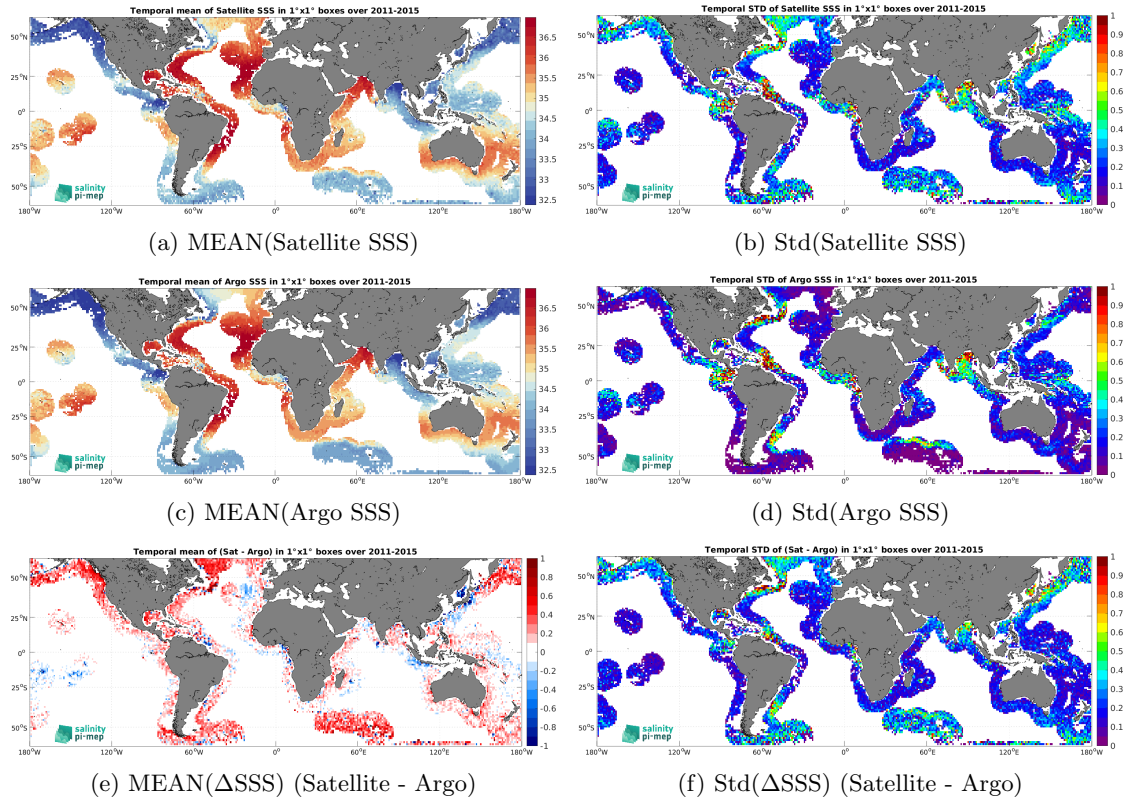
Figure 7: Temporal mean (left) and Std (right) of SSS from Aquarius SSS L3 CAP v5 - 7-Day running (JPL) (top), Argo (middle), and of \Delta SSS (Satellite - Argo). Only match-up pairs are used to generate these maps.
