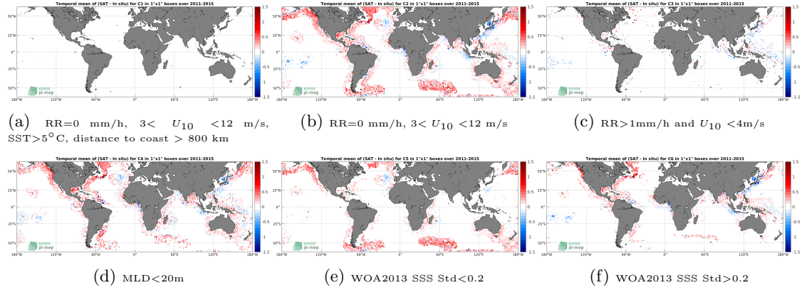
Figure 12: Temporal mean gridded over spatial boxes of size 1^\circ \times 1^\circ of \Delta SSS (Aquarius SSS L3 CAP v5 - 7-Day running (JPL) - Argo) for 6 different subdatasets corresponding to: RR=0 mm/h, 3 < U_{10} < 12 m/s, SST > 5^\circ C , distance to coast > 800 km (a), RR=0 mm/h, 3 < U_{10} < 12 m/s (b), RR > 1 mm/h and U_{10} < 4 m/s (c), MLD < 20 m (d), WOA2013 SSS Std < 0.2 (e), WOA2013 SSS Std > 0.2 (f).
