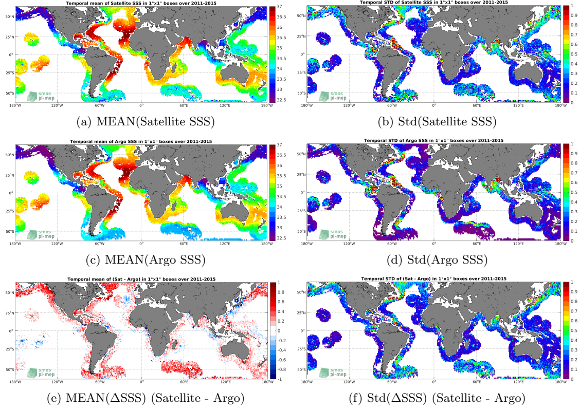
Figure 6: Temporal mean (left) and Std (right) of SSS from Aquarius SSS L3 CAP v5 - 7-Day running (JPL) (top), Argo (middle), and of \Delta SSS (Satellite - Argo). Only match-up pairs are used to generate these maps.
