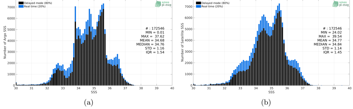
Figure 2: Histograms of SSS from Argo (a) and Aquarius SSS L3 CAP v5 - 7-Day running (JPL) (b) considering all match-up pairs per bins of 0.1 over the SMOS coastal zone (<800km) 60N-60S Pi-MEP region and for the full satellite product period.
