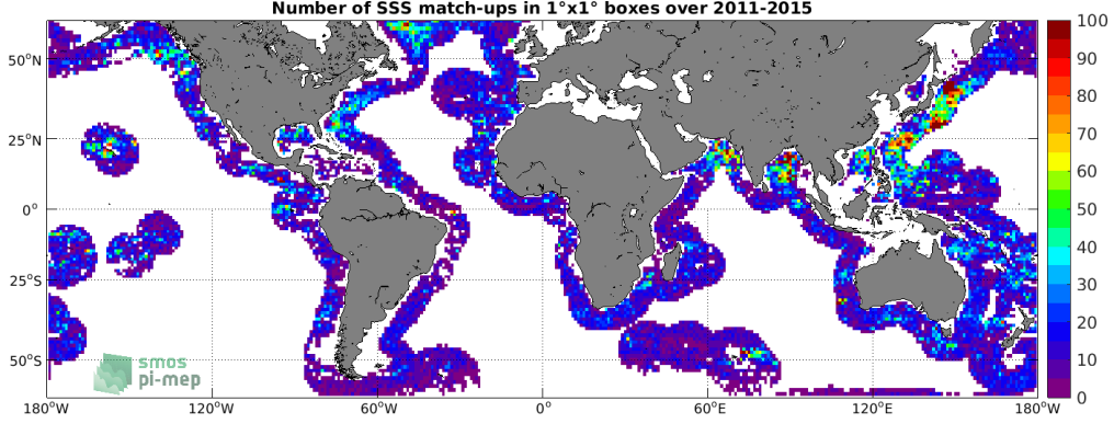
Figure 4: Number of SSS match-ups between Argo SSS and the Aquarius SSS L3 CAP v5 - 7-Day running (JPL) SSS product for the SMOS coastal zone (<800km) 60N-60S Pi-MEP region over 1^\circ \times 1^\circ boxes and for the full satellite product period.
