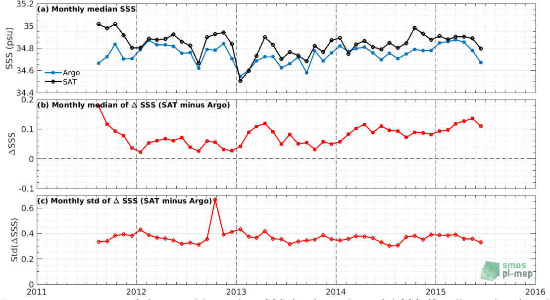
Figure 7: Time series of the monthly median SSS (top), median of \Delta\text{SSS} (Satellite - Argo) and Std of \Delta\text{SSS} (Satellite - Argo) over the SMOS coastal zone (<800km) 60N-60S Pi-MEP region considering all match-ups collected by the Pi-MEP.
