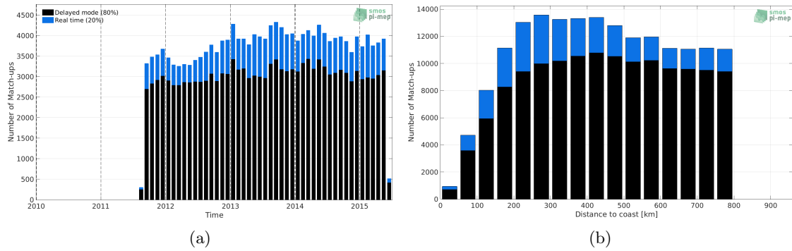
Figure 1: Number of match-ups between Argo and Aquarius SSS L3 CAP v5 - 7-Day running (JPL) SSS as a function of time (a) and as function of the distance to coast (b) over the SMOS coastal zone (<800km) 60N-60S Pi-MEP region and for the full satellite product period.
