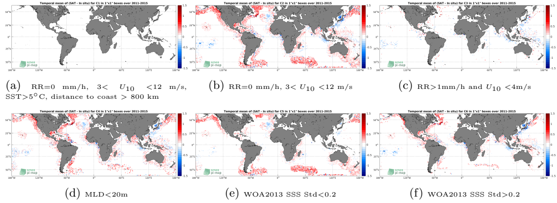
Figure 12: Temporal mean gridded over spatial boxes of size 1^\circ \times 1^\circ of \Delta SSS (Aquarius-L3-JPL-V5-7DAY-RUNNING - Argo) for 6 different subdatasets corresponding to: RR=0 mm/h, 3 < U_{10} < 12 m/s, SST > 5^\circ C , distance to coast > 800 km (a), RR=0 mm/h, 3 < U_{10} < 12 m/s (b), RR > 1 mm/h and U_{10} < 4 m/s (c), MLD < 20 m (d), WOA2013 SSS Std < 0.2 (e), WOA2013 SSS Std > 0.2 (f).
