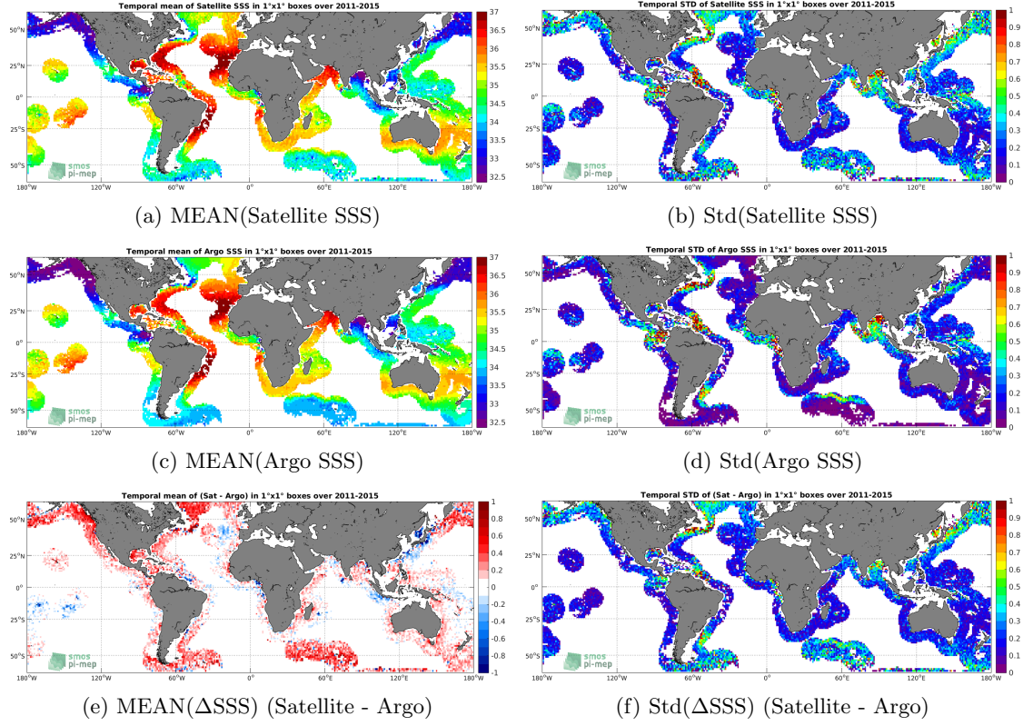
Figure 6: Temporal mean (left) and Std (right) of SSS from Aquarius-L3-JPL-V5-7DAY-RUNNING (top), Argo (middle), and of \Delta SSS (Satellite - Argo). Only match-up pairs are used to generate these maps.
