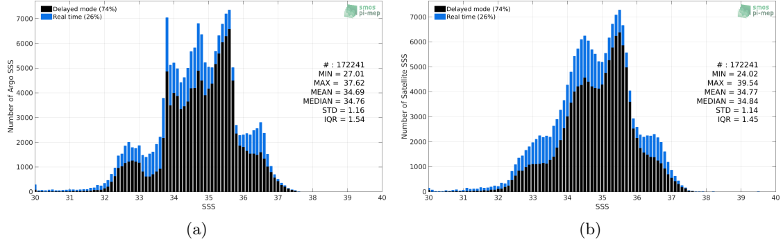
Figure 2: Histograms of SSS from Argo (a) and Aquarius-L3-JPL-V5-7DAY-RUNNING (b) considering all match-up pairs per bins of 0.1 over the SMOS coastal zone (<800km) 60N-60S Pi-MEP region and for the full satellite product period.
