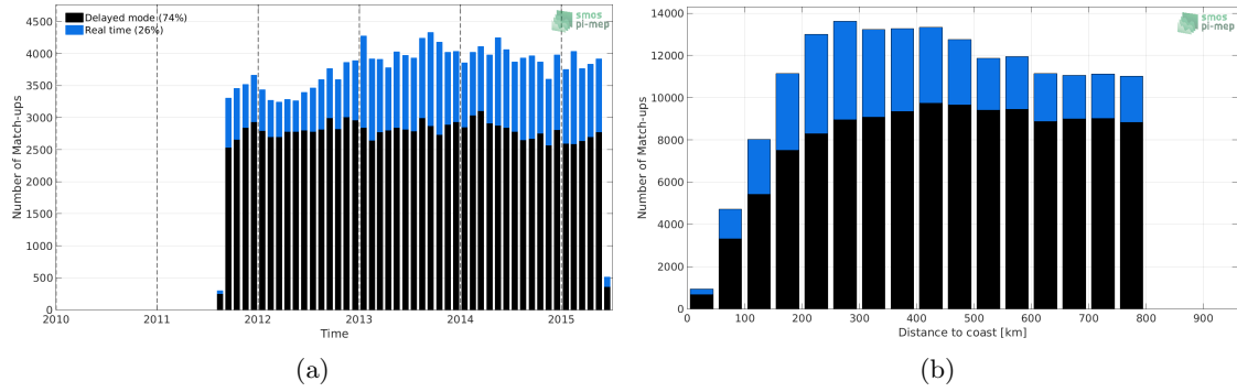
Figure 1: Number of match-ups between Argo and Aquarius-L3-JPL-V5-7DAY-RUNNING SSS as a function of time (a) and as function of the distance to coast (b) over the SMOS coastal zone (<800km) 60N-60S Pi-MEP region and for the full satellite product period.
