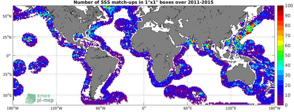
Figure 4: Number of SSS match-ups between Argo SSS and the Aquarius-L3-JPL-V5-7DAY-RUNNING SSS product for the SMOS coastal zone (<800km) 60N-60S Pi-MEP region over 1°x1° boxes and for the full satellite product period.
