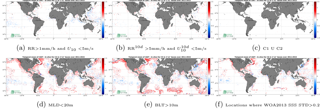
Figure 12: Temporal mean gridded over spatial boxes of size 1^\circ \times 1^\circ of \Delta SSS (Aquarius-L3-JPL-V5-7DAY-RUNNING - Argo) for 6 different subdatasets corresponding to: RR > 1\text{mm/h} and U_{10} < 5\text{m/s} (a), RR^{10d} > 5\text{mm/h} and U_{10}^{10d} < 5\text{m/s} (b), C1 U C2 (c), MLD < 20\text{m} (d), BLT > 10\text{m} (e), Locations where WOA2013 SSS STD > 0.2 (f).
