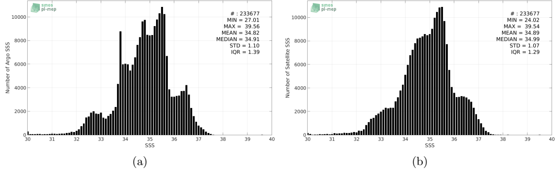
Figure 2: Histograms of SSS from Argo (a) and Aquarius-L3-JPL-V5-7DAY-RUNNING (b) considering all match-up pairs per bins of 0.1 over the SMOS coastal zone ( \approx 800\text{km} ) 60N-60S Pi-MEP region and for the full satellite product period.
