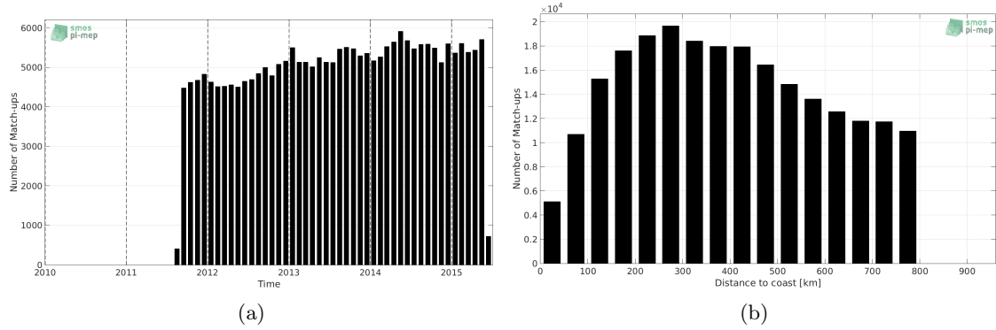
Figure 1: Number of match-ups between Argo and Aquarius-L3-JPL-V5-7DAY-RUNNING SSS as a function of time (a) and as function of the distance to coast (b) over the SMOS coastal zone (800km) 60N-60S Pi-MEP region and for the full satellite product period.
