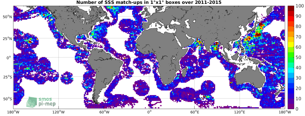
Figure 4: Number of SSS match-ups between Argo SSS and the Aquarius-L3-JPL-V5-7DAY-RUNNING SSS product for the SMOS coastal zone ( \leq 800\text{km} ) 60N-60S Pi-MEP region over 1^\circ \times 1^\circ boxes and for the full satellite product period.
