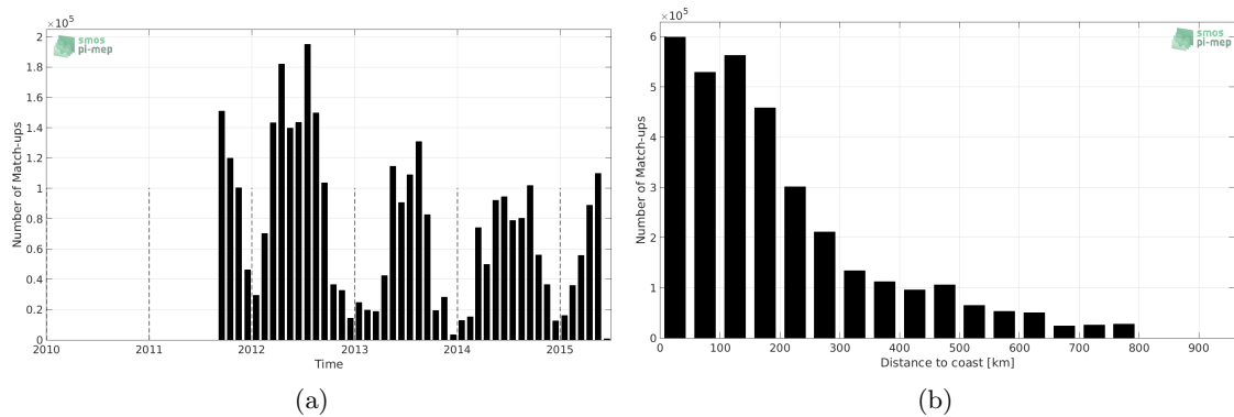
Figure 1: Number of match-ups between TSG-SAMOS and Aquarius-L3-JPL-V5-MONTHLY SSS as a function of time (a) and as function of the distance to coast (b) over the SMOS coastal zone ( \approx 800 km) 60N-60S Pi-MEP region and for the full satellite product period.
