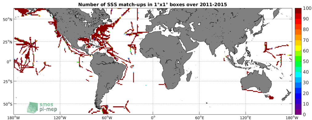
Figure 4: Number of SSS match-ups between TSG-SAMOS SSS and the Aquarius-L3-JPL-V5-MONTHLY SSS product for the SMOS coastal zone ( \approx 800\text{km} ) 60N-60S Pi-MEP region over 1^\circ \times 1^\circ boxes and for the full satellite product period.
