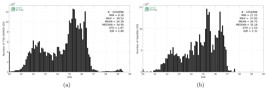
Figure 2: Histograms of SSS from TSG-SAMOS (a) and Aquarius-L3-JPL-V5-MONTHLY (b) considering all match-up pairs per bins of 0.1 over the SMOS coastal zone ( \approx 800 km) 60N-60S Pi-MEP region and for the full satellite product period.
