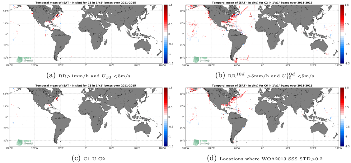
Figure 12: Temporal mean gridded over spatial boxes of size 1^\circ \times 1^\circ of \Delta SSS (Aquarius-L3-JPL-V5-MONTHLY - TSG-SAMOS) for 4 different subdatasets corresponding to: RR > 1\text{mm/h} and U_{10} < 5\text{m/s} (a), RR^{10d} > 5\text{mm/h} and U_{10}^{10d} < 5\text{m/s} (b), C1 U C2 (c), Locations where WOA2013 SSS STD > 0.2 (d).
