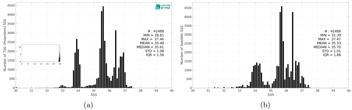
Figure 3: Histograms of SSS from TSG (Polarstern) (a) and Aquarius SSS L3 CAP v5 - Monthly (JPL) (b) considering all match-up pairs per bins of 0.1 over the SMOS coastal zone (<800km) 60N-60S Pi-MEP region and for the full satellite product period.
