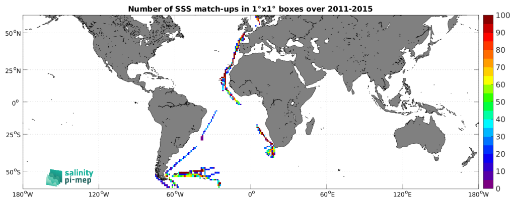
Figure 5: Number of SSS match-ups between TSG (Polarstern) SSS and the Aquarius SSS L3 CAP v5 - Monthly (JPL) SSS product for the SMOS coastal zone (<800km) 60N-60S Pi-MEP region over 1^\circ \times 1^\circ boxes and for the full satellite product period.
