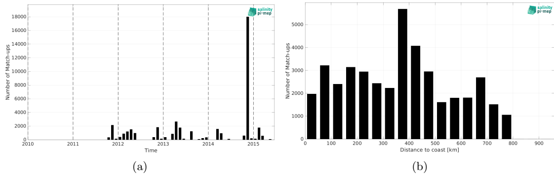
Figure 2: Number of match-ups between TSG (Polarstern) and Aquarius SSS L3 CAP v5 - Monthly (JPL) SSS as a function of time (a) and as function of the distance to coast (b) over the SMOS coastal zone (<800km) 60N-60S Pi-MEP region and for the full satellite product period.
