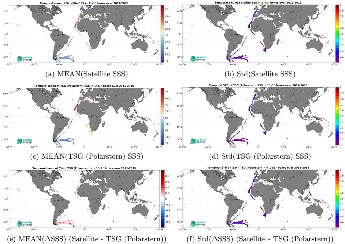
Figure 7: Temporal mean (left) and Std (right) of SSS from Aquarius SSS L3 CAP v5 - Monthly (JPL) (top), TSG (Polarstern) (middle), and of \Delta SSS (Satellite - TSG (Polarstern)). Only match-up pairs are used to generate these maps.
