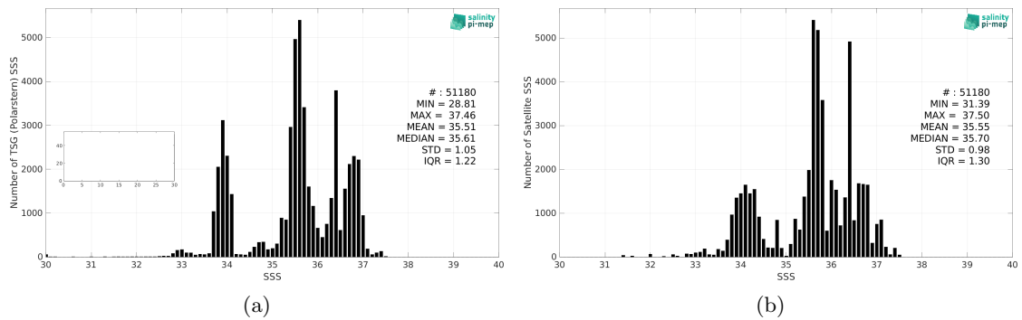
Figure 2: Histograms of SSS from TSG (Polarstern) (a) and Aquarius SSS L3 CAP v5 - Monthly (JPL) (b) considering all match-up pairs per bins of 0.1 over the SMOS coastal zone ( <800\text{km} ) 60N-60S Pi-MEP region and for the full satellite product period.
