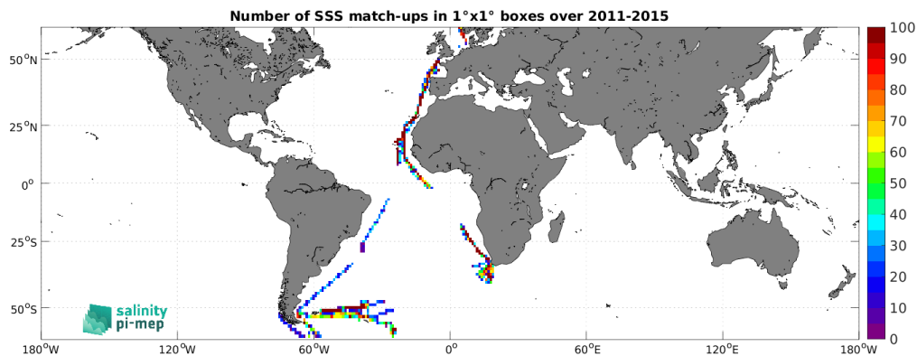
Figure 4: Number of SSS match-ups between TSG (Polarstern) SSS and the Aquarius SSS L3 CAP v5 - Monthly (JPL) SSS product for the SMOS coastal zone (<800km) 60N-60S Pi-MEP region over 1^\circ \times 1^\circ boxes and for the full satellite product period.
