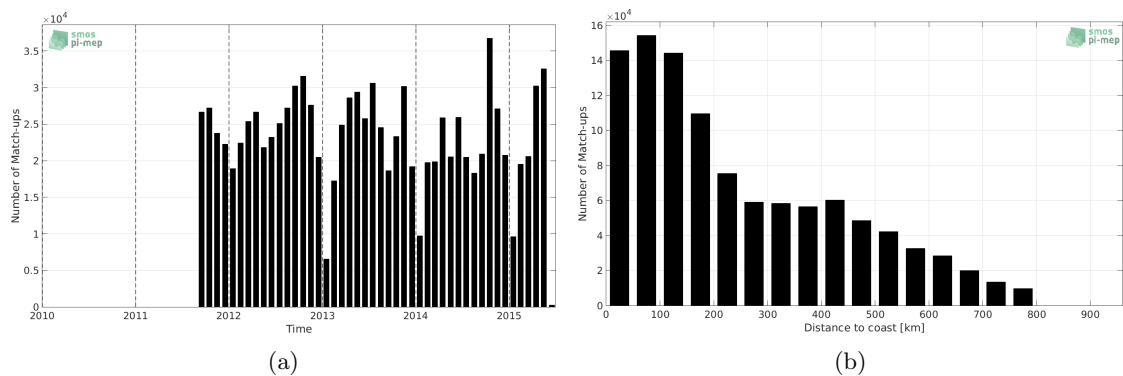
Figure 1: Number of match-ups between TSG-LEGOS-DM and Aquarius-L3-JPL-V5-MONTHLY SSS as a function of time (a) and as function of the distance to coast (b) over the SMOS coastal zone ( \approx 800\text{km} ) 60N-60S Pi-MEP region and for the full satellite product period.
