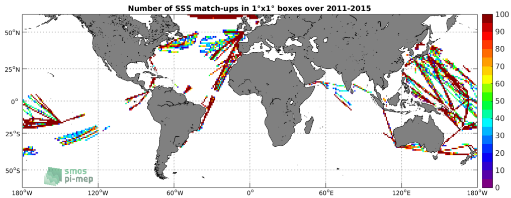
Figure 4: Number of SSS match-ups between TSG-LEGOS-DM SSS and the Aquarius-L3-JPL-V5-MONTHLY SSS product for the SMOS coastal zone ( \pm 800\text{km} ) 60N-60S Pi-MEP region over 1^\circ \times 1^\circ boxes and for the full satellite product period.
