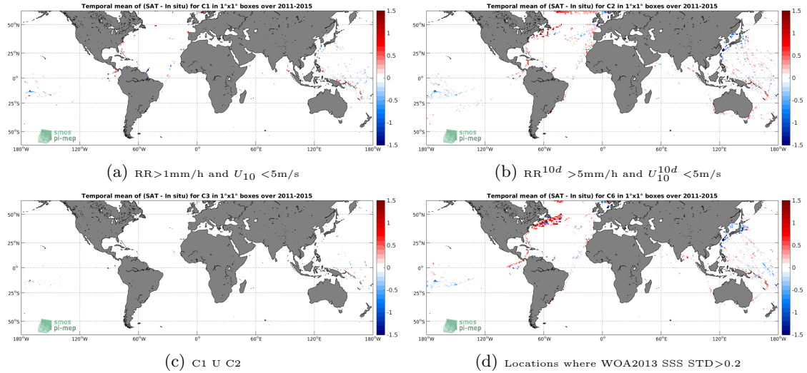
Figure 12: Temporal mean gridded over spatial boxes of size 1^\circ \times 1^\circ of \Delta SSS (Aquarius-L3-JPL-V5-MONTHLY - TSG-LEGOS-DM) for 4 different subdatasets corresponding to: RR > 1\text{mm/h} and U_{10} < 5\text{m/s} (a), RR^{10d} > 5\text{mm/h} and U_{10}^{10d} < 5\text{m/s} (b), C1 U C2 (c), Locations where WOA2013 SSS STD > 0.2 (d).
