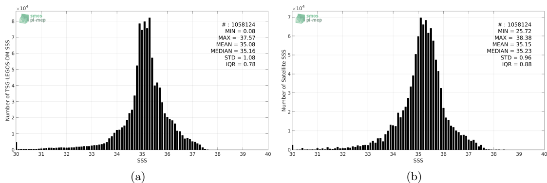
Figure 2: Histograms of SSS from TSG-LEGOS-DM (a) and Aquarius-L3-JPL-V5-MONTHLY (b) considering all match-up pairs per bins of 0.1 over the SMOS coastal zone ( \approx 800\text{km} ) 60N-60S Pi-MEP region and for the full satellite product period.
