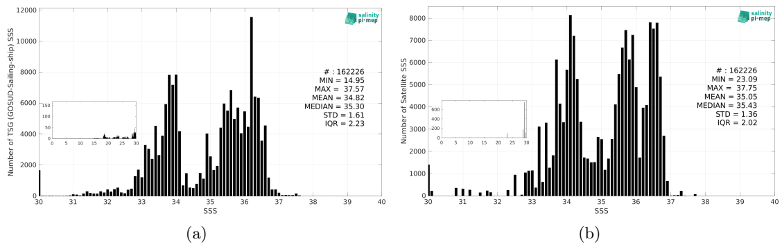
Figure 3: Histograms of SSS from TSG (GOSUD-Sailing-ship) (a) and Aquarius SSS L3 CAP v5 - Monthly (JPL) (b) considering all match-up pairs per bins of 0.1 over the SMOS coastal zone (<800km) 60N-60S Pi-MEP region and for the full satellite product period.
