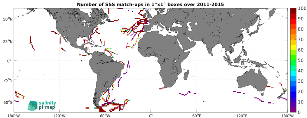
Figure 5: Number of SSS match-ups between TSG (GOSUD-Sailing-ship) SSS and the Aquarius SSS L3 CAP v5 - Monthly (JPL) SSS product for the SMOS coastal zone ( <800\text{km} ) 60N-60S Pi-MEP region over 1^\circ \times 1^\circ boxes and for the full satellite product period.
