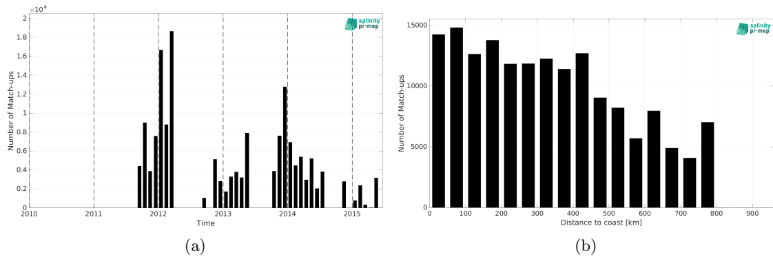
Figure 2: Number of match-ups between TSG (GOSUD-Sailing-ship) and Aquarius SSS L3 CAP v5 - Monthly (JPL) SSS as a function of time (a) and as function of the distance to coast (b) over the SMOS coastal zone (<800km) 60N-60S Pi-MEP region and for the full satellite product period.
