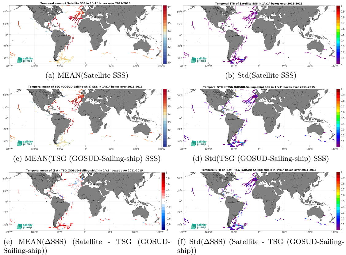
Figure 7: Temporal mean (left) and Std (right) of SSS from Aquarius SSS L3 CAP v5 - Monthly (JPL) (top), TSG (GOSUD-Sailing-ship) (middle), and of \Delta SSS (Satellite - TSG (GOSUD-Sailing-ship)). Only match-up pairs are used to generate these maps.
