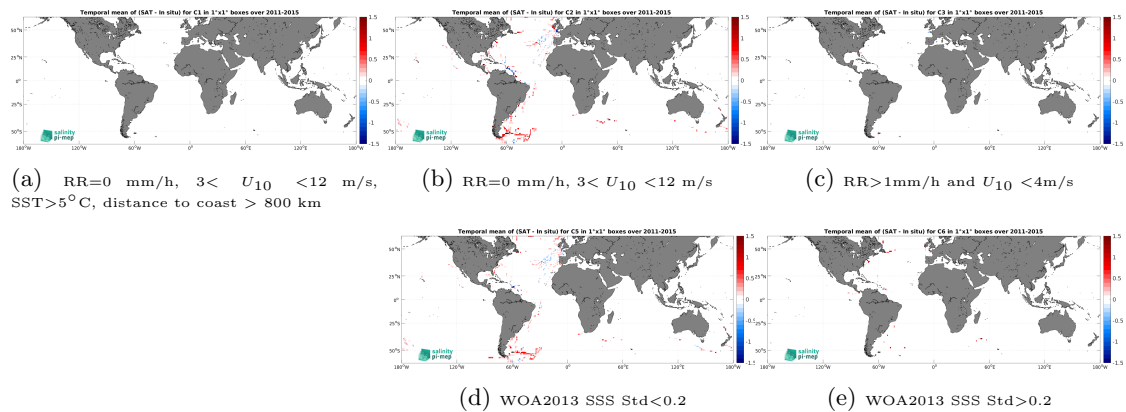
Figure 14: Temporal mean gridded over spatial boxes of size 1^\circ \times 1^\circ of \Delta\text{SSS} (Aquarius SSS L3 CAP v5 - Monthly (JPL) - TSG (GOSUD-Sailing-ship)) for 5 different subdatasets corresponding to:RR=0 mm/h, 3 < U_{10} < 12 m/s, SST>5°C, distance to coast > 800 km (a), RR=0 mm/h, 3 < U_{10} < 12 m/s (b), RR>1mm/h and U_{10} < 4 m/s (c), WOA2013 SSS Std<0.2 (d), WOA2013 SSS Std>0.2 (e).
