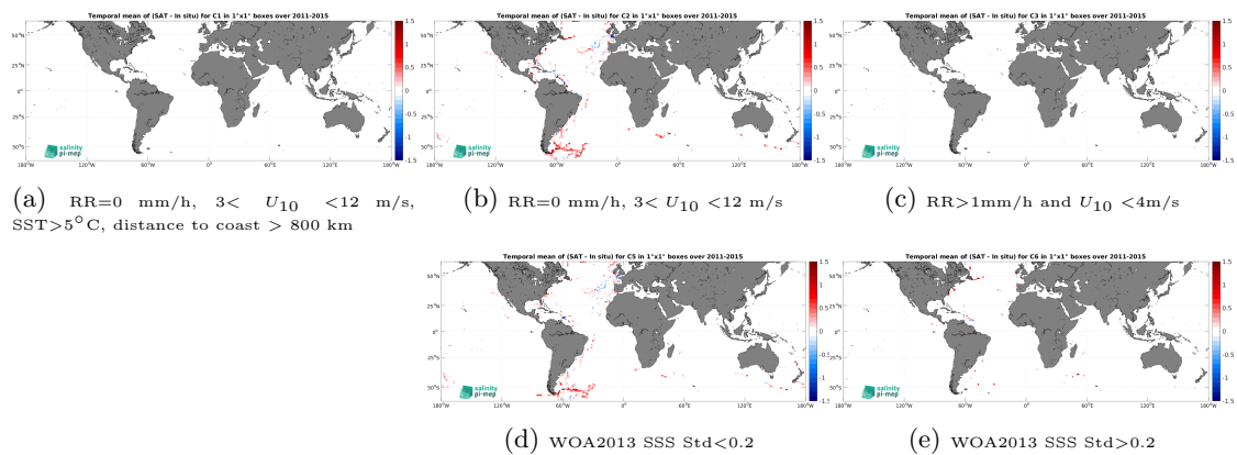
Figure 12: Temporal mean gridded over spatial boxes of size 1^\circ \times 1^\circ of \Delta\text{SSS} (Aquarius SSS L3 CAP v5 - Monthly (JPL) - TSG (GOSUD-Sailing-ship)) for 5 different subdatasets corresponding to:RR=0 mm/h, 3 < U_{10} < 12 m/s, SST >5^\circ\text{C} , distance to coast > 800 km (a), RR=0 mm/h, 3 < U_{10} < 12 m/s (b), RR >1 mm/h and U_{10} < 4 m/s (c), WOA2013 SSS Std <0.2 (d), WOA2013 SSS Std >0.2 (e).
