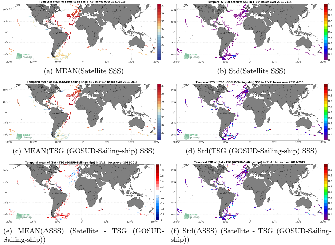
Figure 6: Temporal mean (left) and Std (right) of SSS from Aquarius SSS L3 CAP v5 - Monthly (JPL) (top), TSG (GOSUD-Sailing-ship) (middle), and of \Delta SSS (Satellite - TSG (GOSUD-Sailing-ship)). Only match-up pairs are used to generate these maps.
