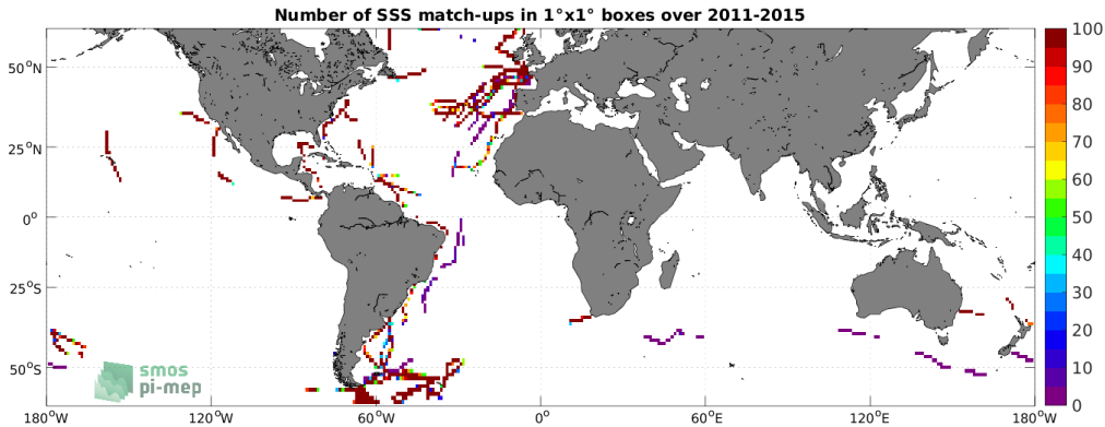
Figure 4: Number of SSS match-ups between TSG (GOSUD-Sailing-ship) SSS and the Aquarius SSS L3 CAP v5 - Monthly (JPL) SSS product for the SMOS coastal zone (<800km) 60N-60S Pi-MEP region over 1^\circ \times 1^\circ boxes and for the full satellite product period.
