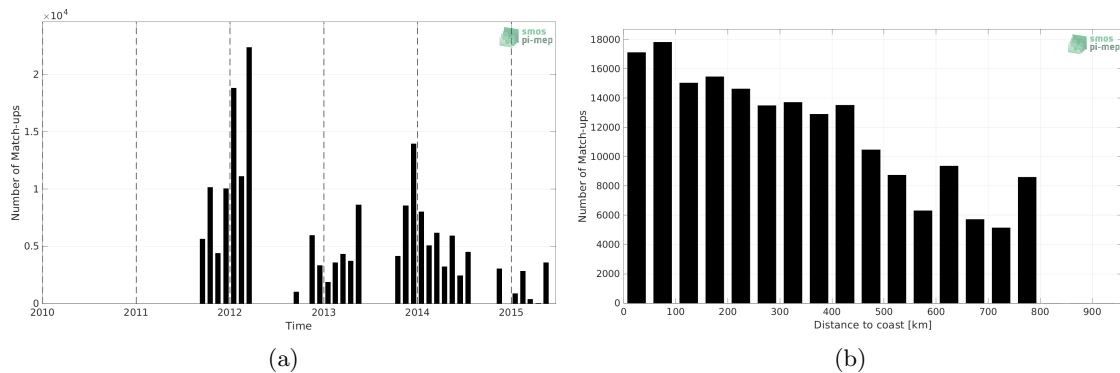
Figure 1: Number of match-ups between TSG (GOSUD-Sailing-ship) and Aquarius SSS L3 CAP v5 - Monthly (JPL) SSS as a function of time (a) and as function of the distance to coast (b) over the SMOS coastal zone (<800km) 60N-60S Pi-MEP region and for the full satellite product period.
