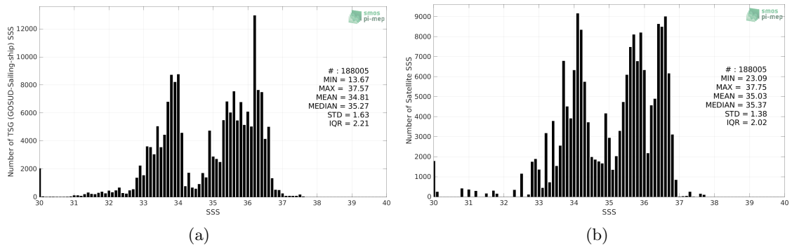
Figure 2: Histograms of SSS from TSG (GOSUD-Sailing-ship) (a) and Aquarius SSS L3 CAP v5 - Monthly (JPL) (b) considering all match-up pairs per bins of 0.1 over the SMOS coastal zone (<800km) 60N-60S Pi-MEP region and for the full satellite product period.
