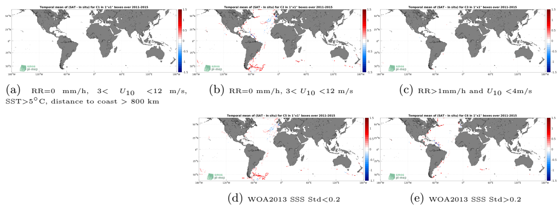
Figure 12: Temporal mean gridded over spatial boxes of size 1^\circ \times 1^\circ of \Delta SSS (Aquarius SSS L3 CAP v5 - Monthly (JPL) - TSG (GOSUD-Sailing-ship)) for 5 different subdatasets corresponding to:RR=0 mm/h, 3 < U_{10} < 12 m/s, SST >5^\circ\text{C} , distance to coast > 800 km (a), RR=0 mm/h, 3 < U_{10} < 12 m/s (b), RR >1 mm/h and U_{10} < 4 m/s (c), WOA2013 SSS Std <0.2 (d), WOA2013 SSS Std >0.2 (e).
