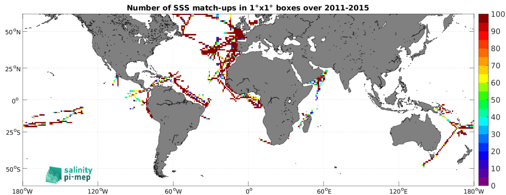
Figure 5: Number of SSS match-ups between TSG (GOSUD-Research-vessel) SSS and the Aquarius SSS L3 CAP v5 - Monthly (JPL) SSS product for the SMOS coastal zone (<800km) 60N-60S Pi-MEP region over 1^\circ \times 1^\circ boxes and for the full satellite product period.
