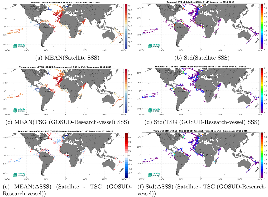
Figure 7: Temporal mean (left) and Std (right) of SSS from Aquarius SSS L3 CAP v5 - Monthly (JPL) (top), TSG (GOSUD-Research-vessel) (middle), and of \Delta SSS (Satellite - TSG (GOSUD-Research-vessel)). Only match-up pairs are used to generate these maps.
