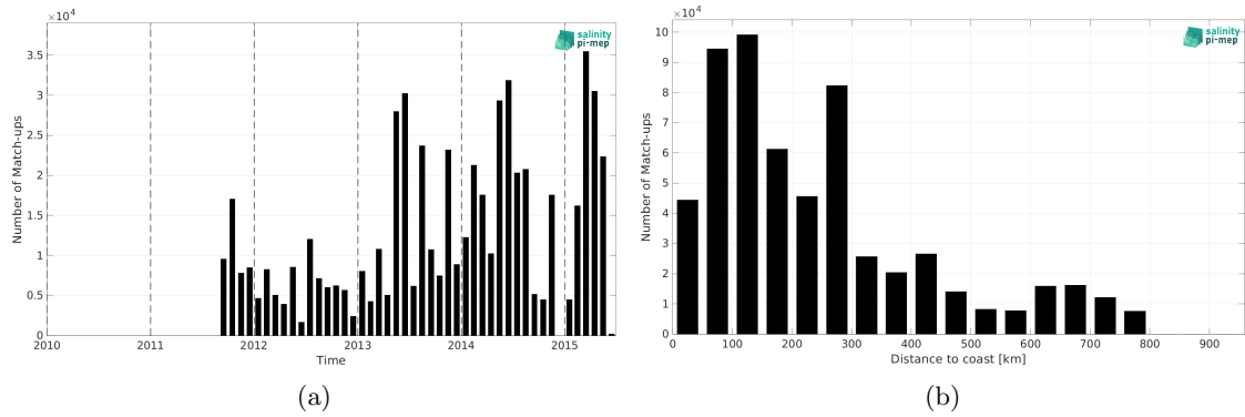
Figure 2: Number of match-ups between TSG (GOSUD-Research-vessel) and Aquarius SSS L3 CAP v5 - Monthly (JPL) SSS as a function of time (a) and as function of the distance to coast (b) over the SMOS coastal zone (<800km) 60N-60S Pi-MEP region and for the full satellite product period.
