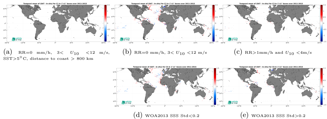
Figure 14: Temporal mean gridded over spatial boxes of size 1^\circ \times 1^\circ of \Delta SSS (Aquarius SSS L3 CAP v5 - Monthly (JPL) - TSG (GOSUD-Research-vessel)) for 5 different subdatasets corresponding to:RR=0 mm/h, 3 < U_{10} < 12 m/s, SST >5^\circ\text{C} , distance to coast > 800 km (a), RR=0 mm/h, 3 < U_{10} < 12 m/s (b), RR >1 mm/h and U_{10} < 4 m/s (c), WOA2013 SSS Std <0.2 (d), WOA2013 SSS Std >0.2 (e).
