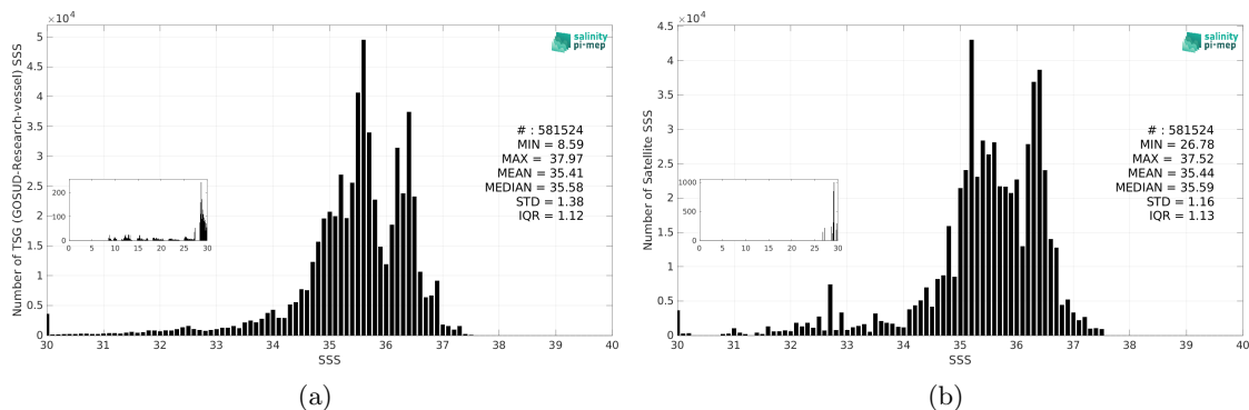
Figure 3: Histograms of SSS from TSG (GOSUD-Research-vessel) (a) and Aquarius SSS L3 CAP v5 - Monthly (JPL) (b) considering all match-up pairs per bins of 0.1 over the SMOS coastal zone (<800km) 60N-60S Pi-MEP region and for the full satellite product period.
