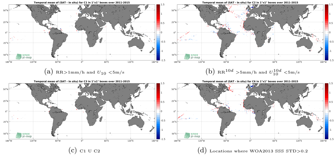
Figure 12: Temporal mean gridded over spatial boxes of size 1^\circ \times 1^\circ of \Delta SSS (Aquarius-L3-JPL-V5-MONTHLY - TSG-GOSUD-Research-vessel) for 4 different subdatasets corresponding to: RR > 1\text{mm/h} and U_{10} < 5\text{m/s} (a), RR^{10d} > 5\text{mm/h} and U_{10}^{10d} < 5\text{m/s} (b), C1 U C2 (c), Locations where WOA2013 SSS STD > 0.2 (d).
