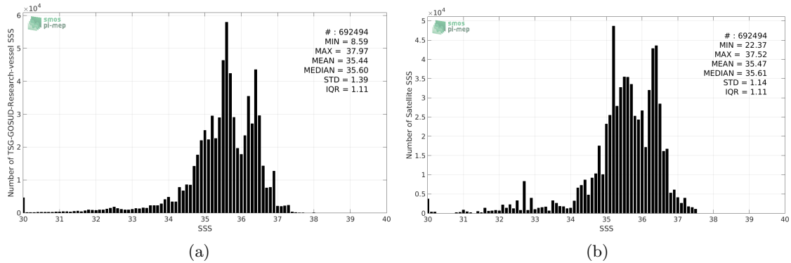
Figure 2: Histograms of SSS from TSG-GOSUD-Research-vessel (a) and Aquarius-L3-JPL-V5-MONTHLY (b) considering all match-up pairs per bins of 0.1 over the SMOS coastal zone ( \approx 800 km) 60N-60S Pi-MEP region and for the full satellite product period.
