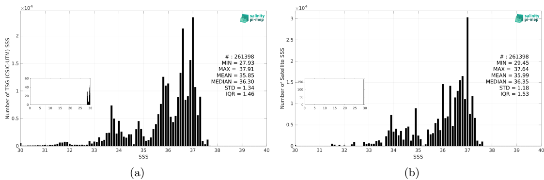
Figure 3: Histograms of SSS from TSG (CSIC-UTM) (a) and Aquarius SSS L3 CAP v5 - Monthly (JPL) (b) considering all match-up pairs per bins of 0.1 over the SMOS coastal zone (<800km) 60N-60S Pi-MEP region and for the full satellite product period.
