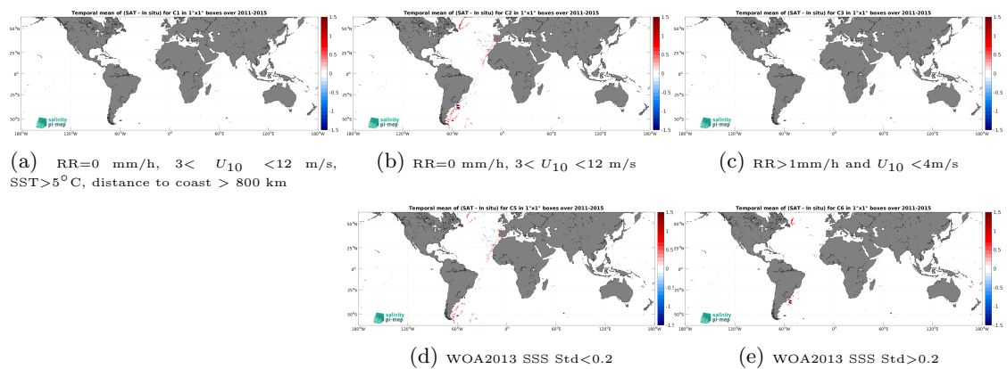
Figure 14: Temporal mean gridded over spatial boxes of size 1^\circ \times 1^\circ of \Delta\text{SSS} (Aquarius SSS L3 CAP v5 - Monthly (JPL) - TSG (CSIC-UTM)) for 5 different subdatasets corresponding to: RR=0 mm/h, 3 < U_{10} < 12 m/s, SST > 5°C, distance to coast > 800 km (a), RR=0 mm/h, 3 < U_{10} < 12 m/s (b), RR > 1mm/h and U_{10} < 4 m/s (c), WOA2013 SSS Std < 0.2 (d), WOA2013 SSS Std > 0.2 (e).
