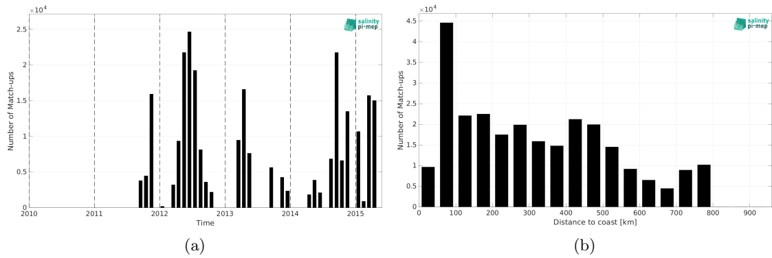
Figure 2: Number of match-ups between TSG (CSIC-UTM) and Aquarius SSS L3 CAP v5 - Monthly (JPL) SSS as a function of time (a) and as function of the distance to coast (b) over the SMOS coastal zone (<800km) 60N-60S Pi-MEP region and for the full satellite product period.
