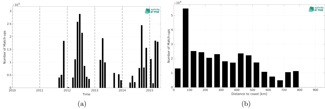
Figure 1: Number of match-ups between TSG (CSIC-UTM) and Aquarius SSS L3 CAP v5 - Monthly (JPL) SSS as a function of time (a) and as function of the distance to coast (b) over the SMOS coastal zone (<800km) 60N-60S Pi-MEP region and for the full satellite product period.
