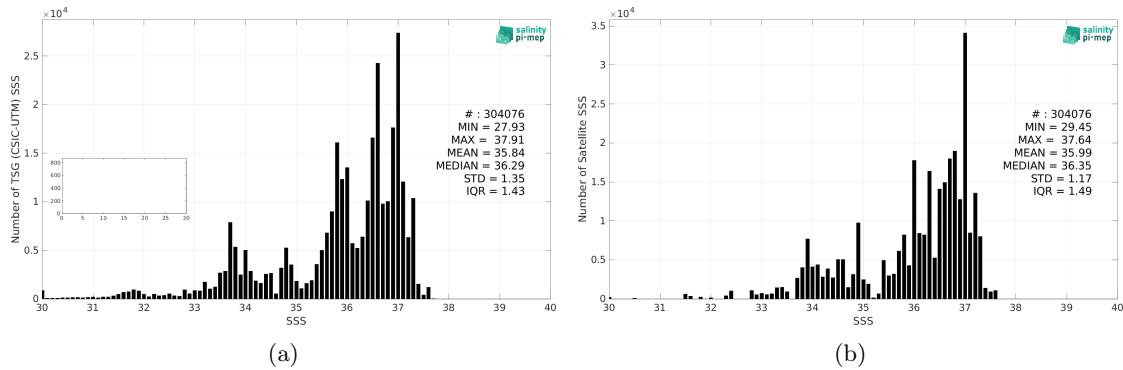
Figure 2: Histograms of SSS from TSG (CSIC-UTM) (a) and Aquarius SSS L3 CAP v5 - Monthly (JPL) (b) considering all match-up pairs per bins of 0.1 over the SMOS coastal zone (<800km) 60N-60S Pi-MEP region and for the full satellite product period.
