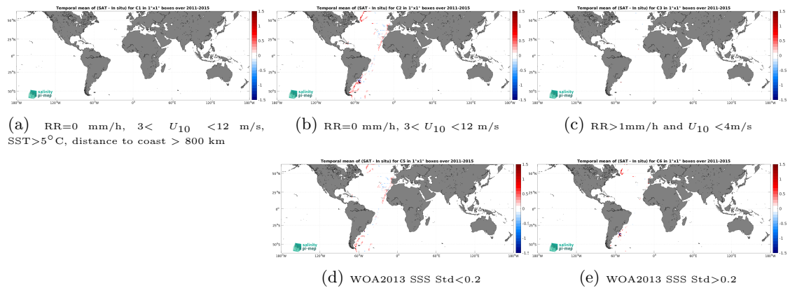
Figure 12: Temporal mean gridded over spatial boxes of size 1^\circ \times 1^\circ of \Delta\text{SSS} (Aquarius SSS L3 CAP v5 - Monthly (JPL) - TSG (CSIC-UTM)) for 5 different subdatasets corresponding to:RR=0 mm/h, 3 < U_{10} < 12 m/s, SST >5^\circ\text{C} , distance to coast > 800 km (a), RR=0 mm/h, 3 < U_{10} < 12 m/s (b), RR >1 mm/h and U_{10} < 4 m/s (c), WOA2013 SSS Std <0.2 (d), WOA2013 SSS Std >0.2 (e).
