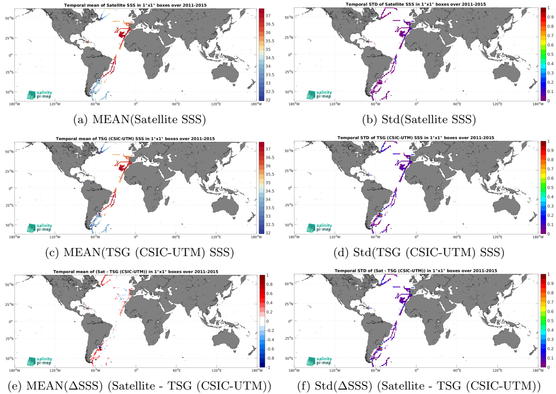
Figure 6: Temporal mean (left) and Std (right) of SSS from Aquarius SSS L3 CAP v5 - Monthly (JPL) (top), TSG (CSIC-UTM) (middle), and of \Delta SSS (Satellite - TSG (CSIC-UTM)). Only match-up pairs are used to generate these maps.
