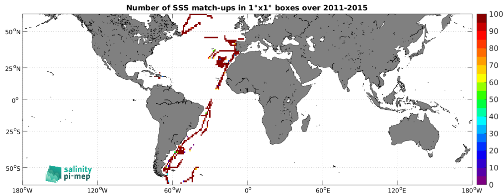
Figure 4: Number of SSS match-ups between TSG (CSIC-UTM) SSS and the Aquarius SSS L3 CAP v5 - Monthly (JPL) SSS product for the SMOS coastal zone (<800km) 60N-60S Pi-MEP region over 1^\circ \times 1^\circ boxes and for the full satellite product period.
