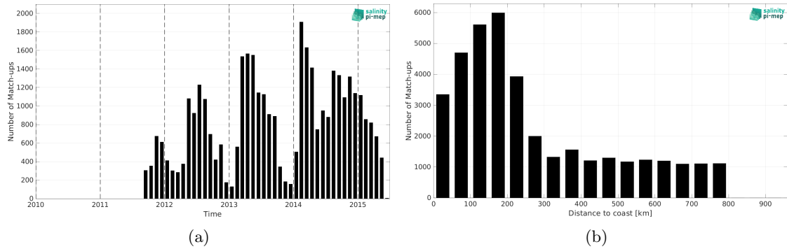
Figure 2: Number of match-ups between Marine mammals and Aquarius SSS L3 CAP v5 - Monthly (JPL) SSS as a function of time (a) and as function of the distance to coast (b) over the SMOS coastal zone (<800km) 60N-60S Pi-MEP region and for the full satellite product period.
