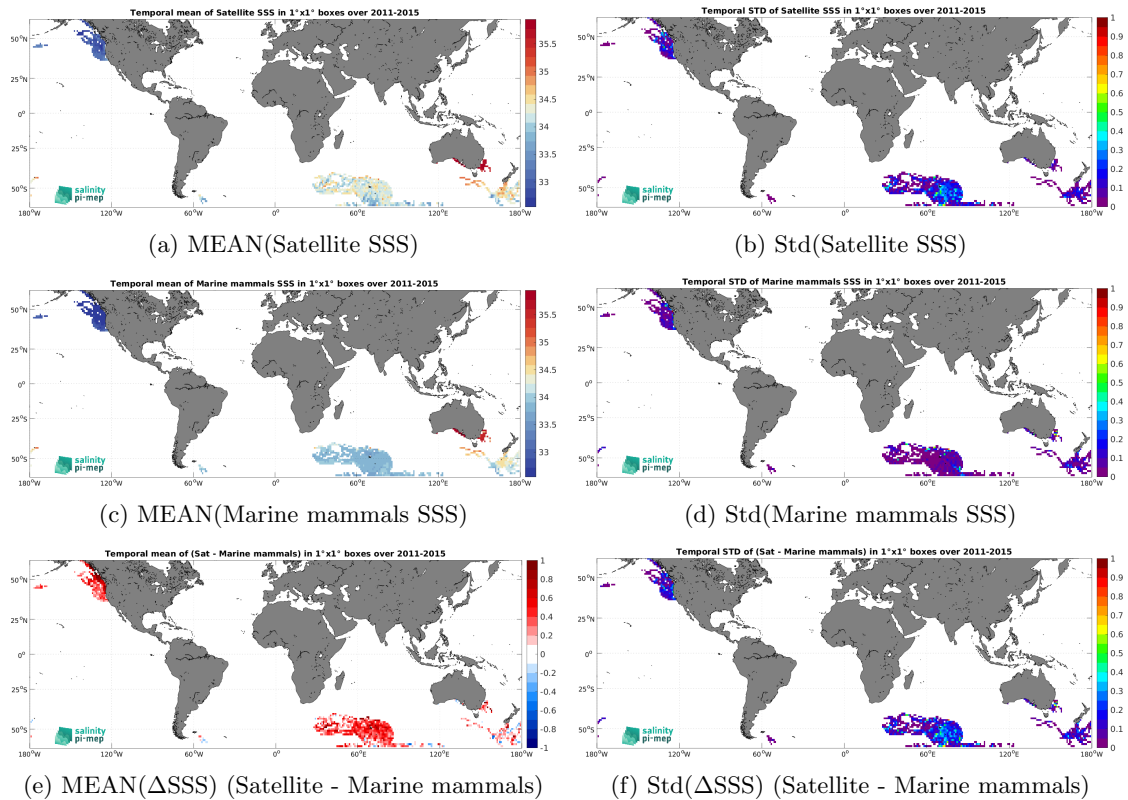
Figure 7: Temporal mean (left) and Std (right) of SSS from Aquarius SSS L3 CAP v5 - Monthly (JPL) (top), Marine mammals (middle), and of \Delta SSS (Satellite - Marine mammals). Only match-up pairs are used to generate these maps.
