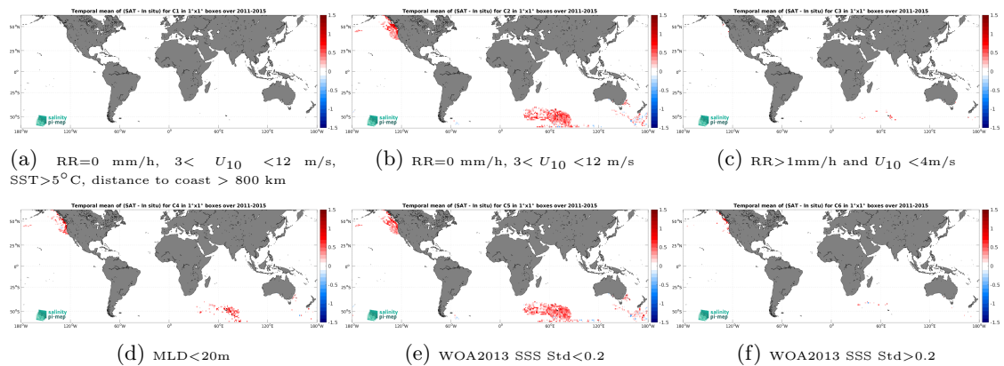
Figure 14: Temporal mean gridded over spatial boxes of size 1^\circ \times 1^\circ of \Delta SSS (Aquarius SSS L3 CAP v5 - Monthly (JPL) - Marine mammals) for 6 different subdatasets corresponding to:RR=0 mm/h, 3 < U_{10} < 12 m/s, SST >5^\circ C, distance to coast > 800 km (a), RR=0 mm/h, 3 < U_{10} < 12 m/s (b), RR >1 mm/h and U_{10} < 4 m/s (c),MLD <20 m (d),WOA2013 SSS Std <0.2 (e),WOA2013 SSS Std >0.2 (f).
