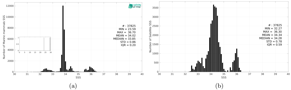
Figure 3: Histograms of SSS from Marine mammals (a) and Aquarius SSS L3 CAP v5 - Monthly (JPL) (b) considering all match-up pairs per bins of 0.1 over the SMOS coastal zone (<800km) 60N-60S Pi-MEP region and for the full satellite product period.
