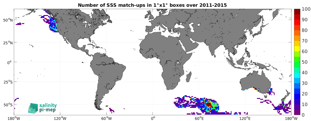
Figure 5: Number of SSS match-ups between Marine mammals SSS and the Aquarius SSS L3 CAP v5 - Monthly (JPL) SSS product for the SMOS coastal zone (<800km) 60N-60S Pi-MEP region over 1^\circ \times 1^\circ boxes and for the full satellite product period.
