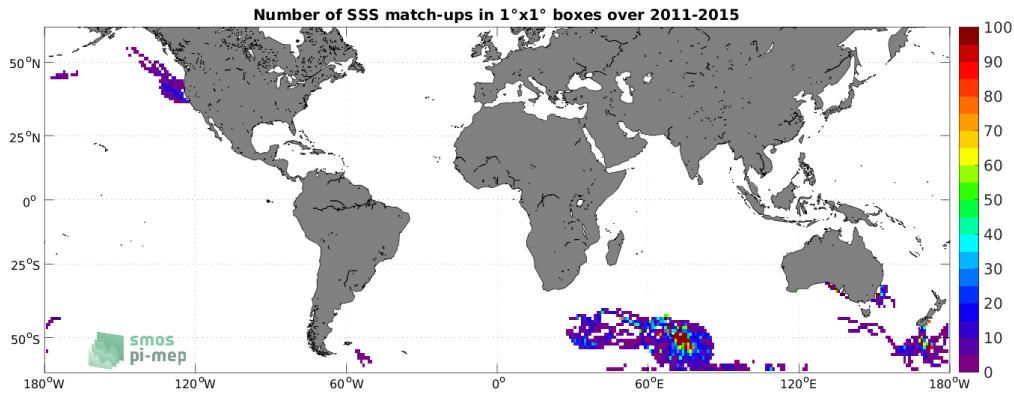
Figure 4: Number of SSS match-ups between Marine mammals SSS and the Aquarius SSS L3 CAP v5 - Monthly (JPL) SSS product for the SMOS coastal zone (<800km) 60N-60S Pi-MEP region over 1°x1° boxes and for the full satellite product period.
