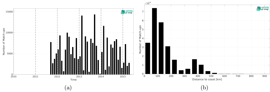
Figure 2: Number of match-ups between ICES and Aquarius SSS L3 CAP v5 - Monthly (JPL) SSS as a function of time (a) and as function of the distance to coast (b) over the SMOS coastal zone (<800km) 60N-60S Pi-MEP region and for the full satellite product period.
