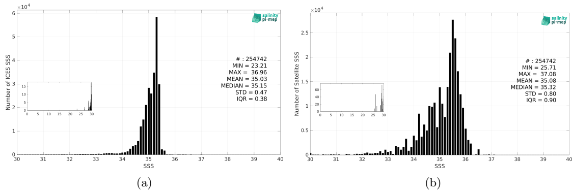
Figure 3: Histograms of SSS from ICES (a) and Aquarius SSS L3 CAP v5 - Monthly (JPL) (b) considering all match-up pairs per bins of 0.1 over the SMOS coastal zone (<800km) 60N-60S Pi-MEP region and for the full satellite product period.
