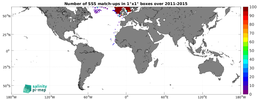
Figure 5: Number of SSS match-ups between ICES SSS and the Aquarius SSS L3 CAP v5 - Monthly (JPL) SSS product for the SMOS coastal zone (<800km) 60N-60S Pi-MEP region over 1^\circ \times 1^\circ boxes and for the full satellite product period.
