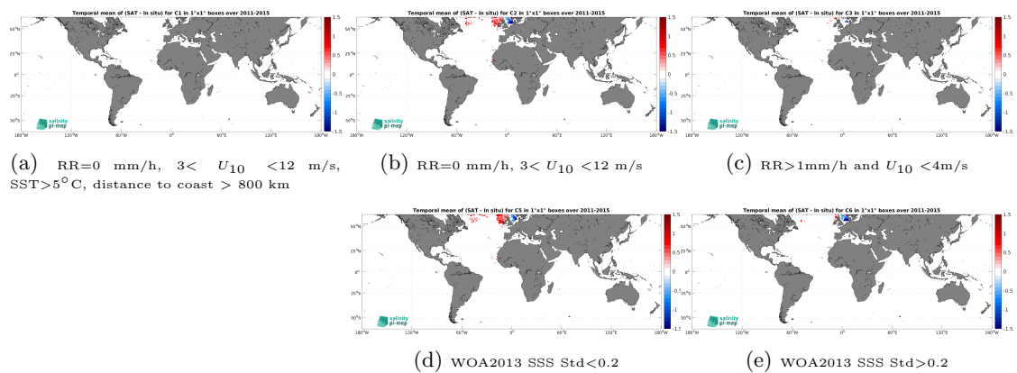
Figure 14: Temporal mean gridded over spatial boxes of size 1^\circ \times 1^\circ of \Delta SSS (Aquarius SSS L3 CAP v5 - Monthly (JPL) - ICES) for 5 different subdatasets corresponding to:RR=0 mm/h, 3 < U_{10} < 12 m/s, SST >5^\circ\text{C} , distance to coast > 800 km (a), RR=0 mm/h, 3 < U_{10} < 12 m/s (b), RR >1 mm/h and U_{10} < 4 m/s (c), WOA2013 SSS Std <0.2 (d), WOA2013 SSS Std >0.2 (e).
