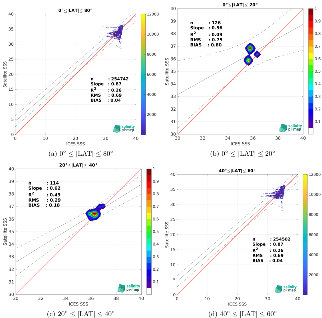
Figure 10: Contour maps of the concentration of Aquarius SSS L3 CAP v5 - Monthly (JPL) SSS (y-axis) versus ICES SSS (x-axis) at match-up pairs for different latitude bands. For each plot, the red line shows x=y . The black thin and dashed lines indicate a linear fit through the data cloud and the \pm 95\% confidence levels, respectively. The number match-up pairs n , the slope and R^2 coefficient of the linear fit, the root mean square (RMS) and the mean bias between satellite and in situ data are indicated for each latitude band in each plots.
