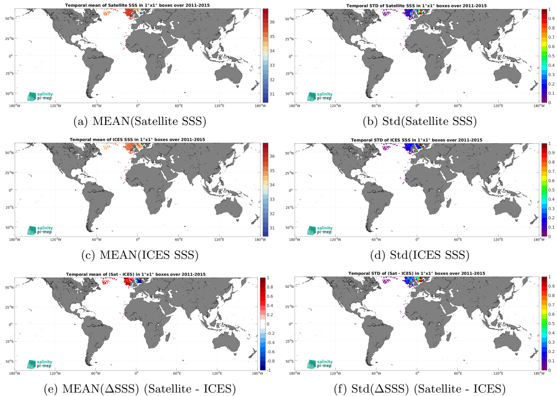
Figure 7: Temporal mean (left) and Std (right) of SSS from Aquarius SSS L3 CAP v5 - Monthly (JPL) (top), ICES (middle), and of \Delta SSS (Satellite - ICES). Only match-up pairs are used to generate these maps.
