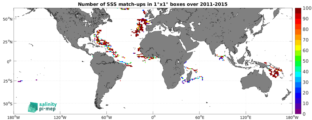
Figure 4: Number of SSS match-ups between Surface drifters SSS and the Aquarius SSS L3 CAP v5 - Monthly (JPL) SSS product for the SMOS coastal zone (<800km) 60N-60S Pi-MEP region over 1^\circ \times 1^\circ boxes and for the full satellite product period.
