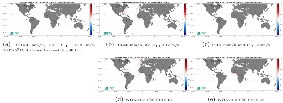
Figure 13: Temporal mean gridded over spatial boxes of size 1^\circ \times 1^\circ of \Delta SSS (Aquarius SSS L3 CAP v5 - Monthly (JPL) - Surface drifters) for 5 different subdatasets corresponding to:RR=0 mm/h, 3 < U_{10} < 12 m/s, SST >5^\circ\text{C} , distance to coast > 800 km (a), RR=0 mm/h, 3 < U_{10} < 12 m/s (b), RR >1 mm/h and U_{10} < 4 m/s (c), WOA2013 SSS Std <0.2 (d), WOA2013 SSS Std >0.2 (e).
