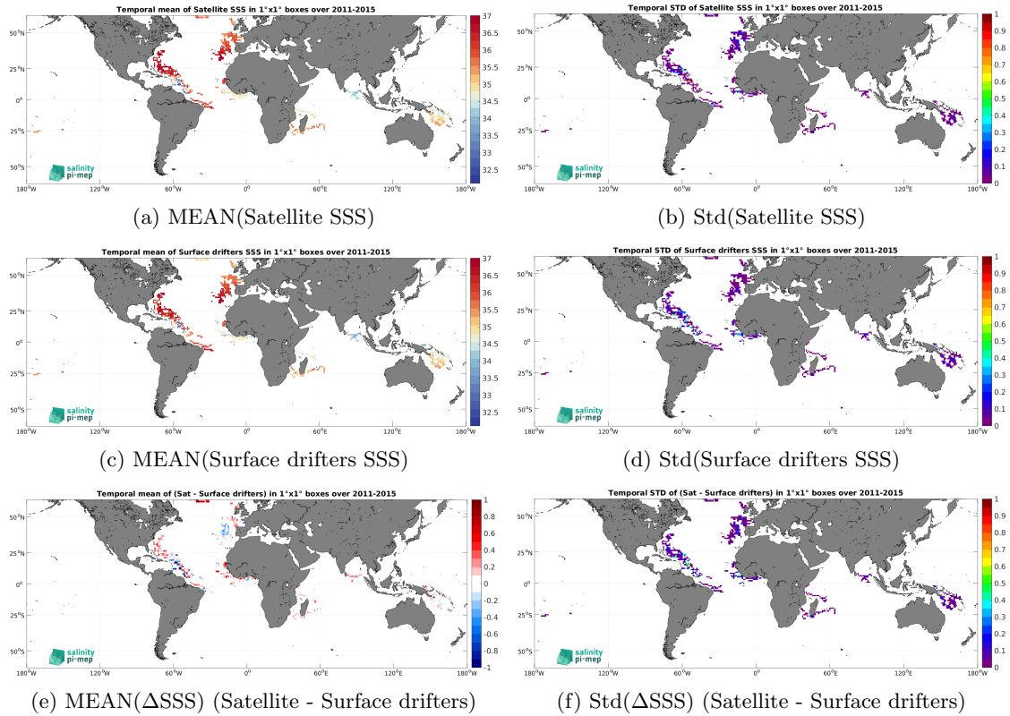
Figure 6: Temporal mean (left) and Std (right) of SSS from Aquarius SSS L3 CAP v5 - Monthly (JPL) (top), Surface drifters (middle), and of \Delta SSS (Satellite - Surface drifters). Only match-up pairs are used to generate these maps.
