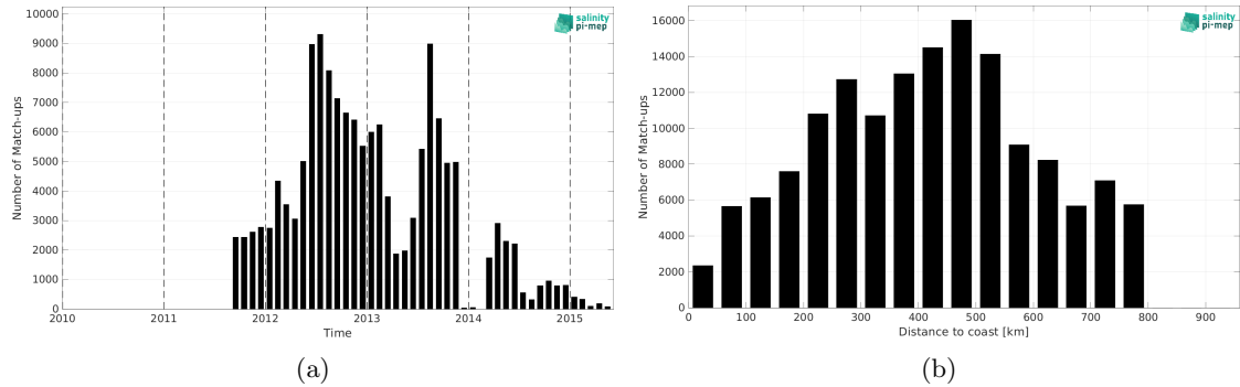
Figure 2: Number of match-ups between Surface drifters and Aquarius SSS L3 CAP v5 - Monthly (JPL) SSS as a function of time (a) and as function of the distance to coast (b) over the SMOS coastal zone (<800km) 60N-60S Pi-MEP region and for the full satellite product period.
