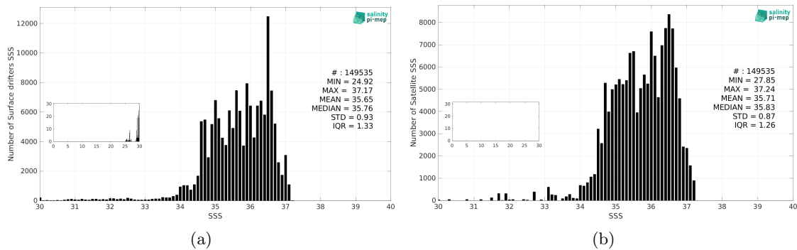
Figure 3: Histograms of SSS from Surface drifters (a) and Aquarius SSS L3 CAP v5 - Monthly (JPL) (b) considering all match-up pairs per bins of 0.1 over the SMOS coastal zone (<800km) 60N-60S Pi-MEP region and for the full satellite product period.
