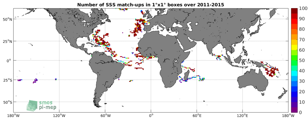
Figure 3: Number of SSS match-ups between Surface drifters SSS and the Aquarius-L3-JPL-V5-MONTHLY SSS product for the SMOS coastal zone ( \approx 800\text{km} ) 60N-60S Pi-MEP region over 1^\circ \times 1^\circ boxes and for the full satellite product period.
