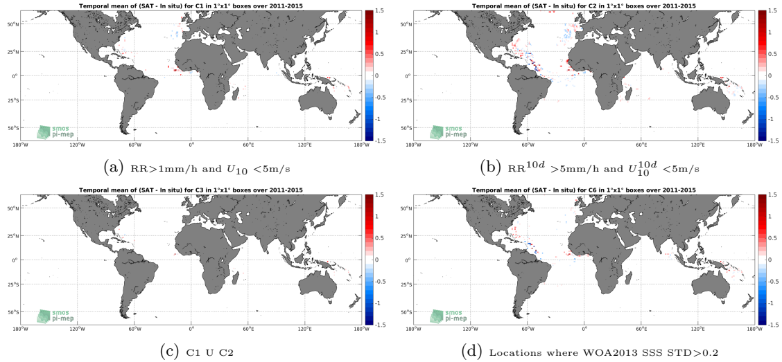
Figure 11: Temporal mean gridded over spatial boxes of size 1^\circ \times 1^\circ of \Delta SSS (Aquarius-L3-JPL-V5-MONTHLY - Surface drifters) for 4 different subdatasets corresponding to: RR > 1\text{mm/h} and U_{10} < 5\text{m/s} (a), RR^{10d} > 5\text{mm/h} and U_{10}^{10d} < 5\text{m/s} (b), C1 U C2 (c), Locations where WOA2013 SSS STD > 0.2 (d).
