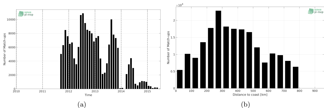
Figure 1: Number of match-ups between Surface drifters and Aquarius-L3-JPL-V5-MONTHLY SSS as a function of time (a) and as function of the distance to coast (b) over the SMOS coastal zone ( \pm 800 km) 60N-60S Pi-MEP region and for the full satellite product period.
