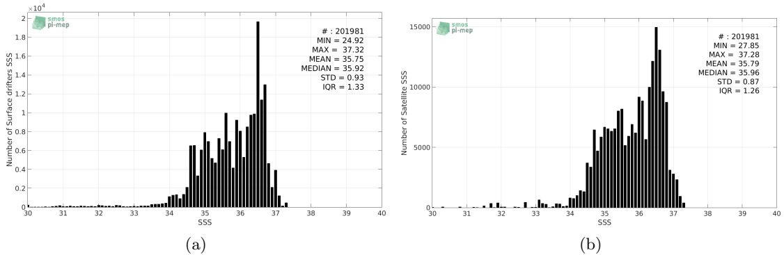
Figure 2: Histograms of SSS from Surface drifters (a) and Aquarius-L3-JPL-V5-MONTHLY (b) considering all match-up pairs per bins of 0.1 over the SMOS coastal zone ( \approx 800\text{km} ) 60N-60S Pi-MEP region and for the full satellite product period.
