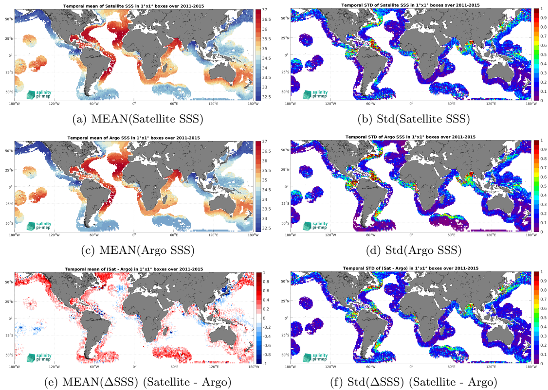
Figure 6: Temporal mean (left) and Std (right) of SSS from Aquarius SSS L3 CAP v5 - Monthly (JPL) (top), Argo (middle), and of \Delta SSS (Satellite - Argo). Only match-up pairs are used to generate these maps.
