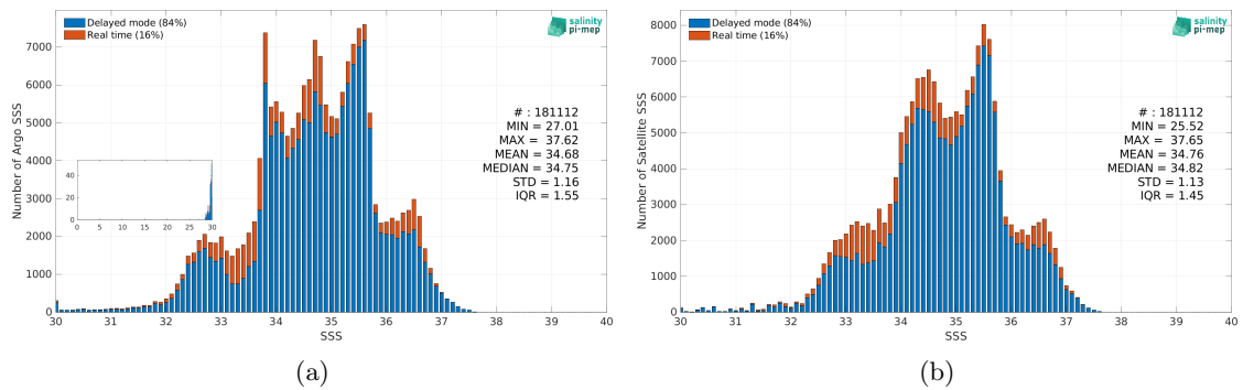
Figure 2: Histograms of SSS from Argo (a) and Aquarius SSS L3 CAP v5 - Monthly (JPL) (b) considering all match-up pairs per bins of 0.1 over the SMOS coastal zone (<800km) 60N-60S Pi-MEP region and for the full satellite product period.
