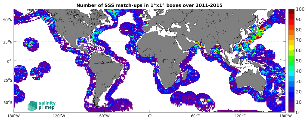
Figure 4: Number of SSS match-ups between Argo SSS and the Aquarius SSS L3 CAP v5 - Monthly (JPL) SSS product for the SMOS coastal zone (<800km) 60N-60S Pi-MEP region over 1^\circ \times 1^\circ boxes and for the full satellite product period.
