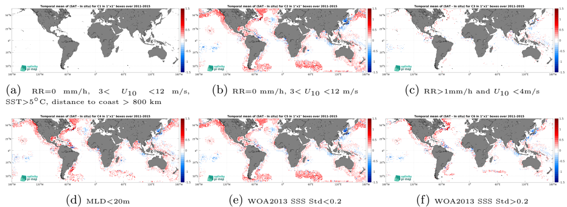
Figure 12: Temporal mean gridded over spatial boxes of size 1^\circ \times 1^\circ of \Delta SSS (Aquarius SSS L3 CAP v5 - Monthly (JPL) - Argo) for 6 different subdatasets corresponding to:RR=0 mm/h, 3 < U_{10} < 12 m/s, SST >5^\circ C, distance to coast > 800 km (a), RR=0 mm/h, 3 < U_{10} < 12 m/s (b), RR >1 mm/h and U_{10} < 4 m/s (c),MLD <20 m (d),WOA2013 SSS Std <0.2 (e),WOA2013 SSS Std >0.2 (f).
