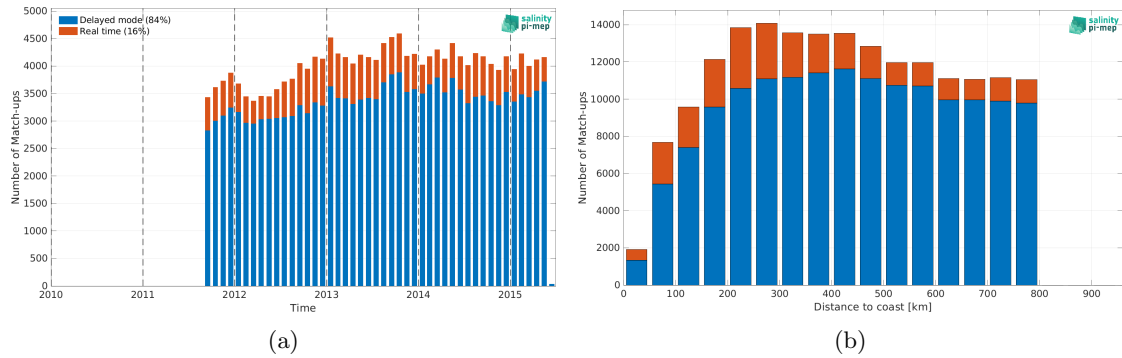
Figure 1: Number of match-ups between Argo and Aquarius SSS L3 CAP v5 - Monthly (JPL) SSS as a function of time (a) and as function of the distance to coast (b) over the SMOS coastal zone (<800km) 60N-60S Pi-MEP region and for the full satellite product period.
