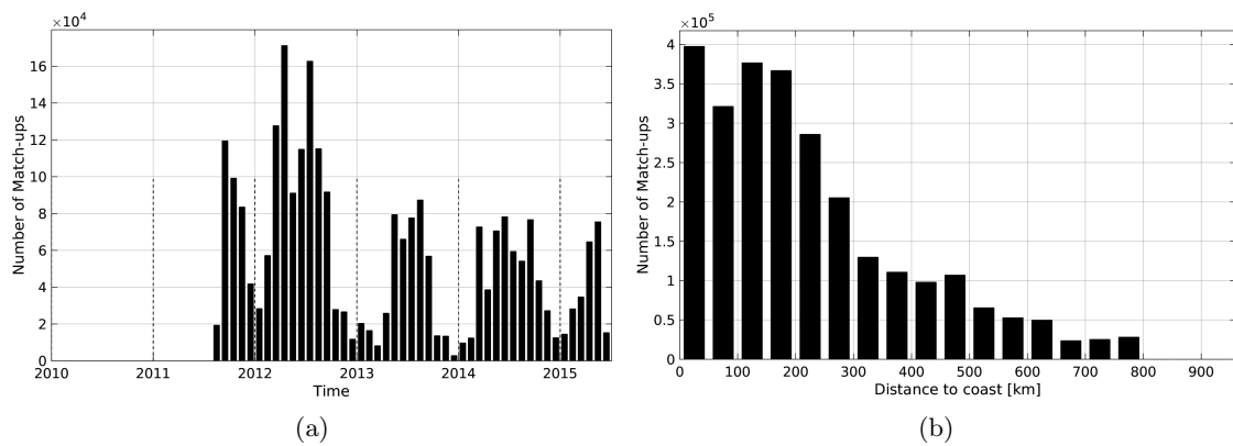
Figure 1: Number of match-ups between TSG-SAMOS and Aquarius-L3-JPL-V4-7DAY-RUNNING SSS as a function of time (a) and as function of the distance to coast (b) over the SMOS coastal zone ( \approx 800 km) 60N-60S Pi-MEP region and for the full satellite product period.
