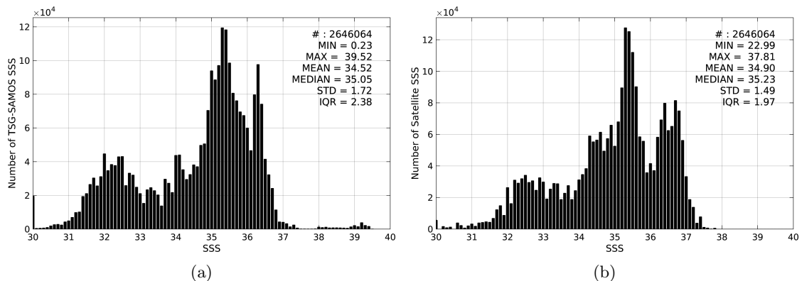
Figure 2: Histograms of SSS from TSG-SAMOS (a) and Aquarius-L3-JPL-V4-7DAY-RUNNING (b) considering all match-up pairs per bins of 0.1 over the SMOS coastal zone ( \approx 800 km) 60N-60S Pi-MEP region and for the full satellite product period.
