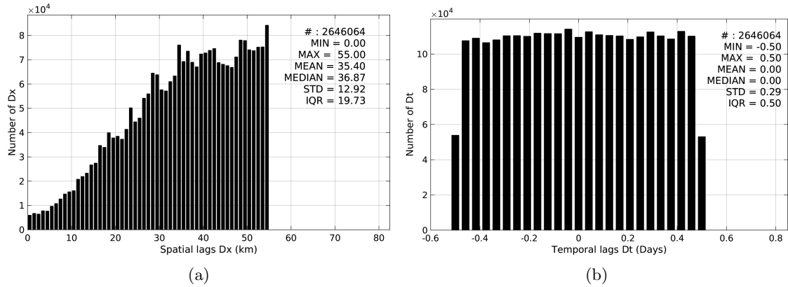
Figure 5: Histograms of the spatial (a) and temporal (b) lags between the time of the TSG-SAMOS measurements and the date of the corresponding Aquarius-L3-JPL-V4-7DAY-RUNNING SSS product.
