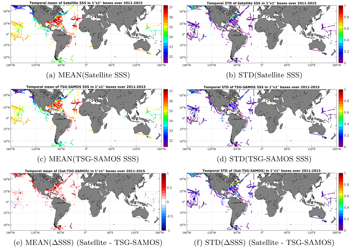
Figure 6: Temporal mean (left) and STD (right) of SSS from Aquarius-L3-JPL-V4-7DAY-RUNNING (top), TSG-SAMOS (middle), and of \Delta SSS (Satellite - TSG-SAMOS). Only match-up pairs are used to generate these maps.
