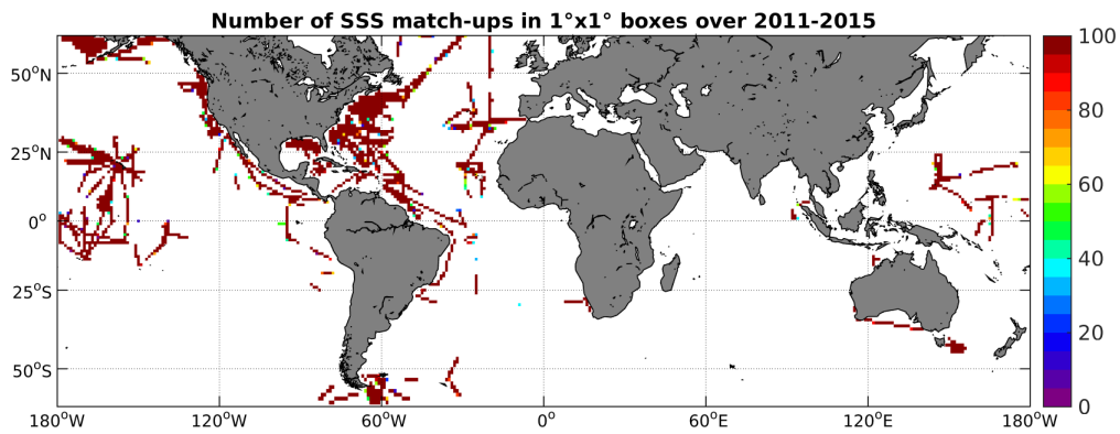
Figure 4: Number of SSS match-ups between TSG-SAMOS SSS and the Aquarius-L3-JPL-V4-7DAY-RUNNING SSS product for the SMOS coastal zone ( \approx 800\text{km} ) 60N-60S Pi-MEP region over 1^\circ \times 1^\circ boxes and for the full satellite product period.
