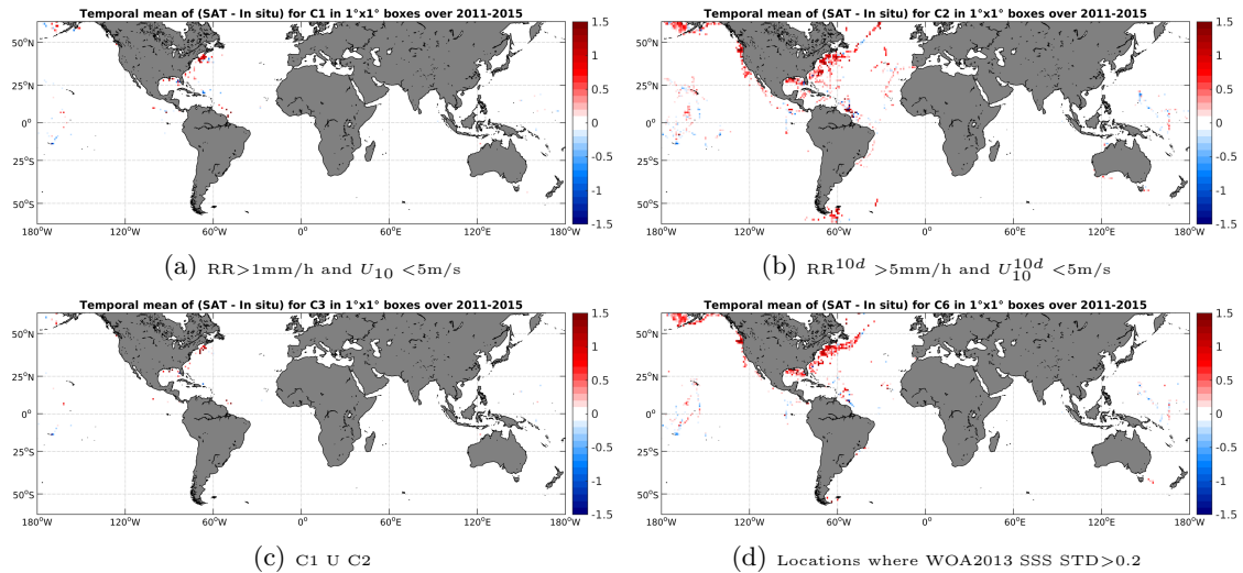
Figure 12: Temporal mean gridded over spatial boxes of size 1^\circ \times 1^\circ of \Delta SSS (Aquarius-L3-JPL-V4-7DAY-RUNNING - TSG-SAMOS) for 4 different subdatasets corresponding to: RR > 1\text{mm/h} and U_{10} < 5\text{m/s} (a), RR^{10d} > 5\text{mm/h} and U_{10}^{10d} < 5\text{m/s} (b), C1 U C2 (c), Locations where WOA2013 SSS STD > 0.2 (d).
