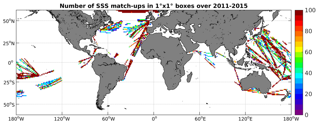
Figure 4: Number of SSS match-ups between TSG-LEGOS-DM SSS and the Aquarius-L3-JPL-V4-7DAY-RUNNING SSS product for the SMOS coastal zone ( \pm 800\text{km} ) 60N-60S Pi-MEP region over 1^\circ \times 1^\circ boxes and for the full satellite product period.
