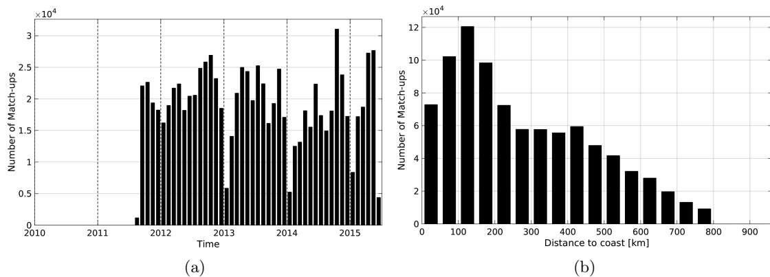
Figure 1: Number of match-ups between TSG-LEGOS-DM and Aquarius-L3-JPL-V4-7DAY-RUNNING SSS as a function of time (a) and as function of the distance to coast (b) over the SMOS coastal zone ( \pm 800 km) 60N-60S Pi-MEP region and for the full satellite product period.
