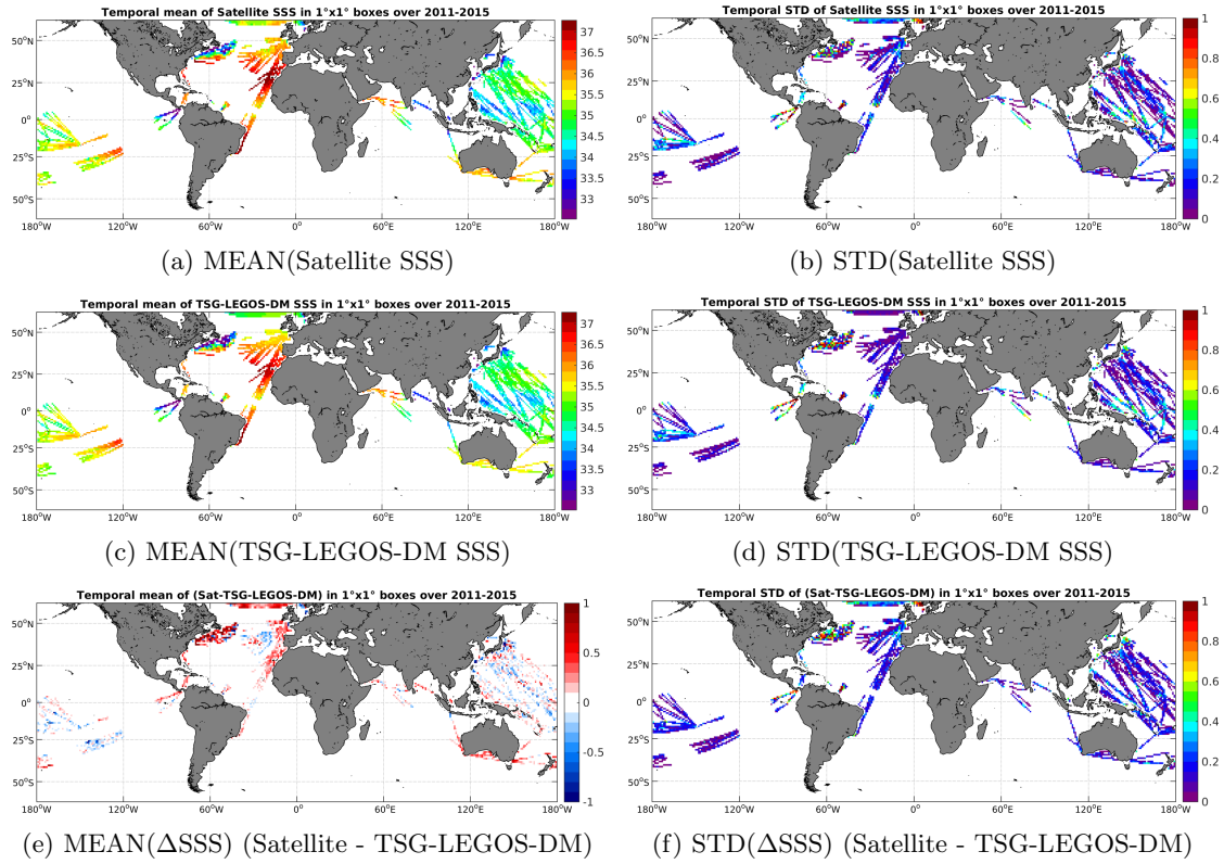
Figure 6: Temporal mean (left) and STD (right) of SSS from Aquarius-L3-JPL-V4-7DAY-RUNNING (top), TSG-LEGOS-DM (middle), and of \Delta SSS (Satellite - TSG-LEGOS-DM). Only match-up pairs are used to generate these maps.
