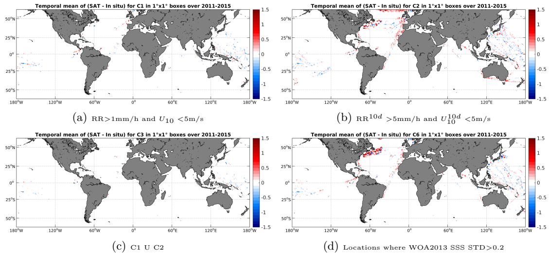
Figure 12: Temporal mean gridded over spatial boxes of size 1^\circ \times 1^\circ of \Delta SSS (Aquarius-L3-JPL-V4-7DAY-RUNNING - TSG-LEGOS-DM) for 4 different subdatasets corresponding to: RR > 1\text{mm/h} and U_{10} < 5\text{m/s} (a), RR^{10d} > 5\text{mm/h} and U_{10}^{10d} < 5\text{m/s} (b), C1 U C2 (c), Locations where WOA2013 SSS STD > 0.2 (d).
