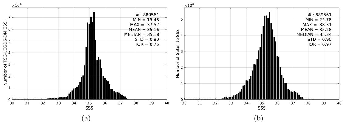
Figure 2: Histograms of SSS from TSG-LEGOS-DM (a) and Aquarius-L3-JPL-V4-7DAY-RUNNING (b) considering all match-up pairs per bins of 0.1 over the SMOS coastal zone ( \pm 800 km) 60N-60S Pi-MEP region and for the full satellite product period.
