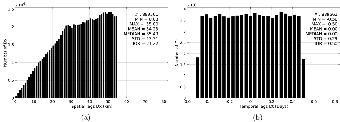
Figure 5: Histograms of the spatial (a) and temporal (b) lags between the time of the TSG-LEGOS-DM measurements and the date of the corresponding Aquarius-L3-JPL-V4-7DAY-RUNNING SSS product.
